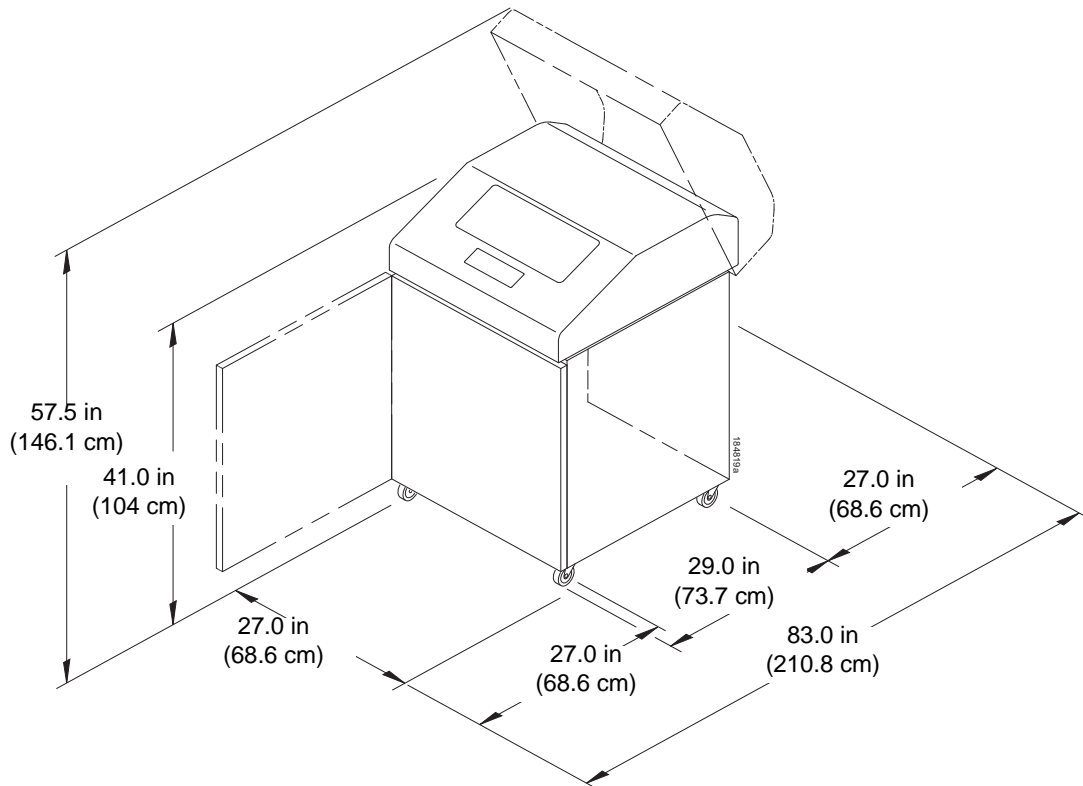
Figure 2. Cabinet Model
