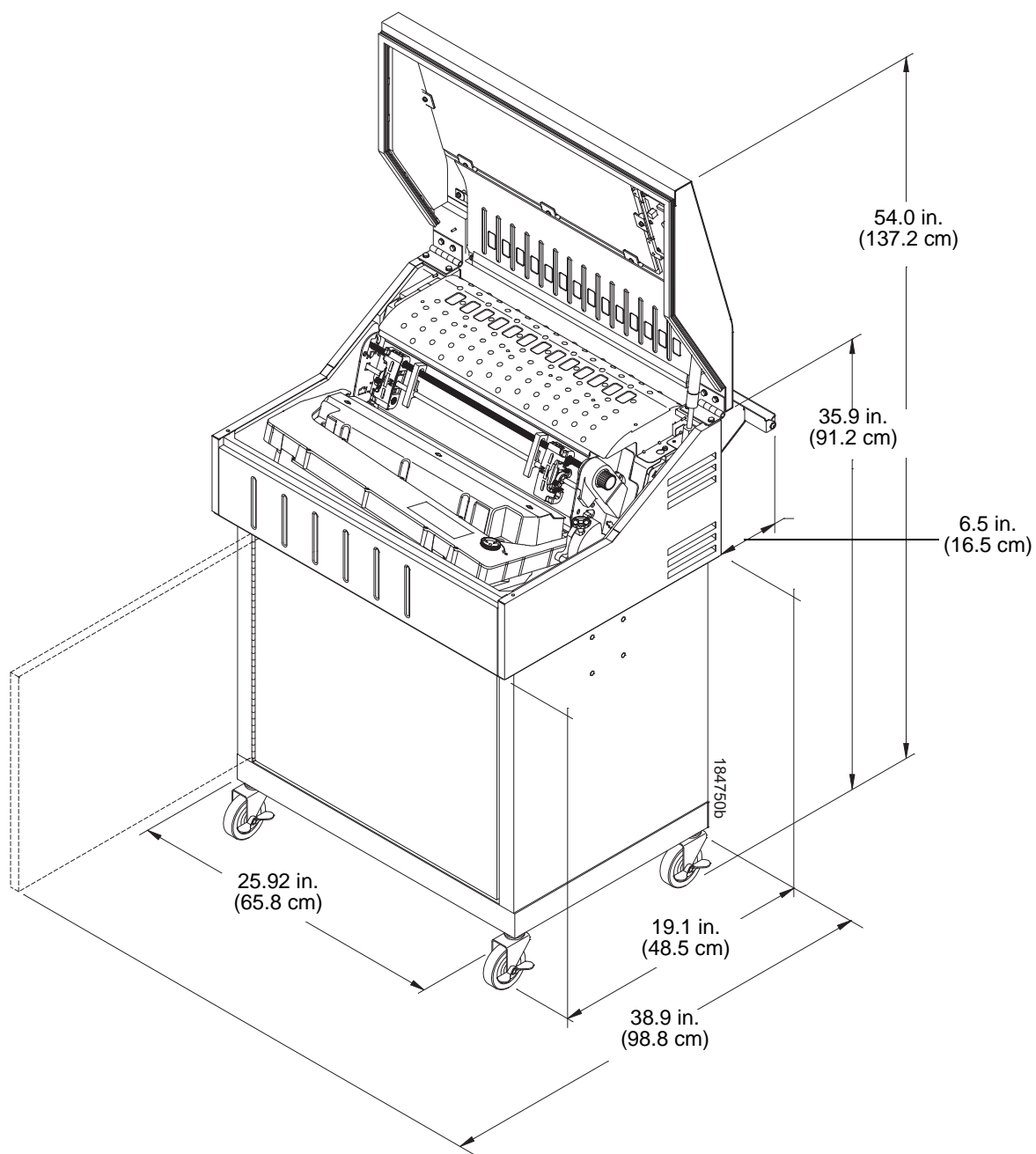
Figure 5. Enclosed Pedestal
