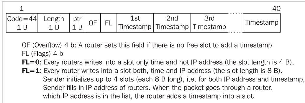
Figure 5.20: Timestamp
