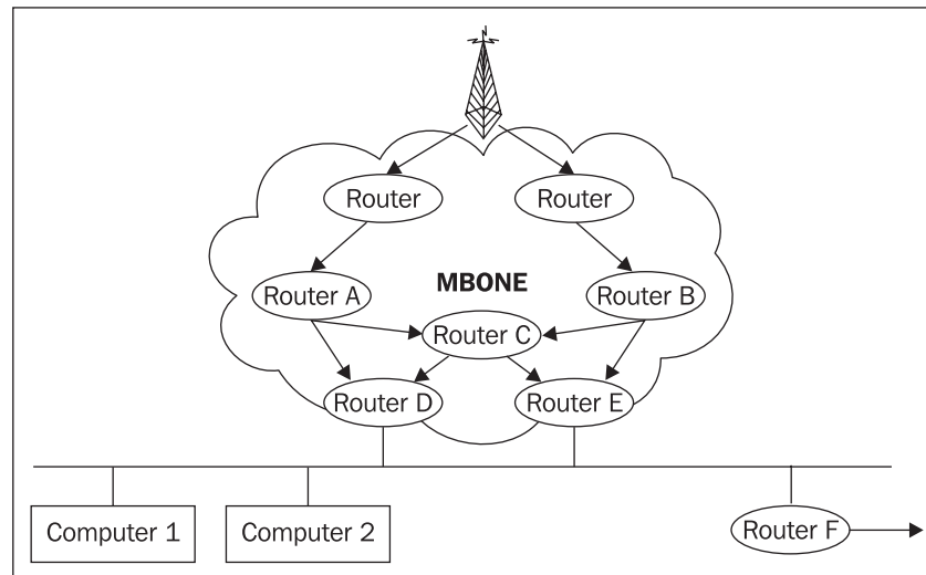
Figure 5.31: Multicasts flooding
