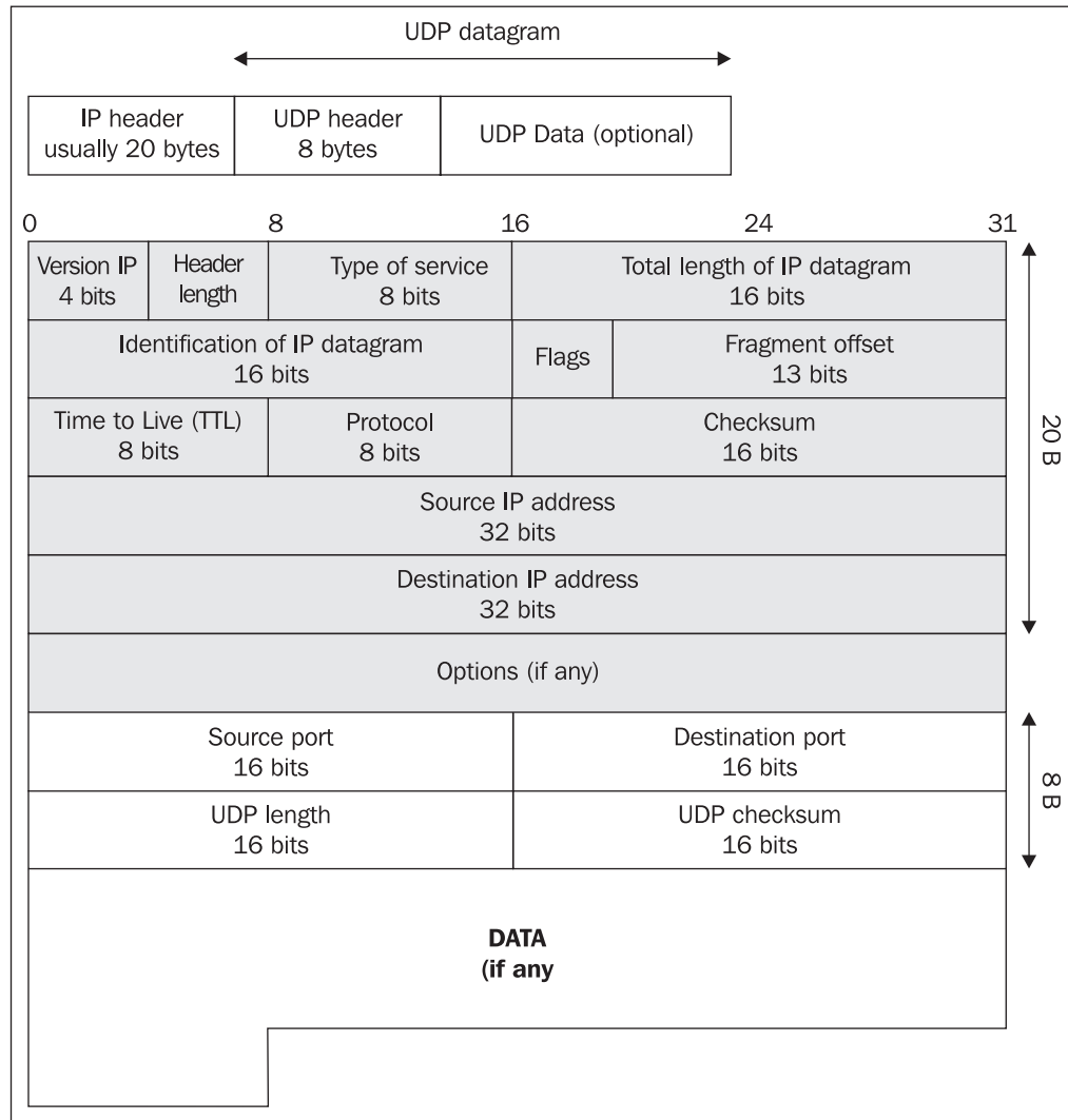
Figure 10.2: UDP
