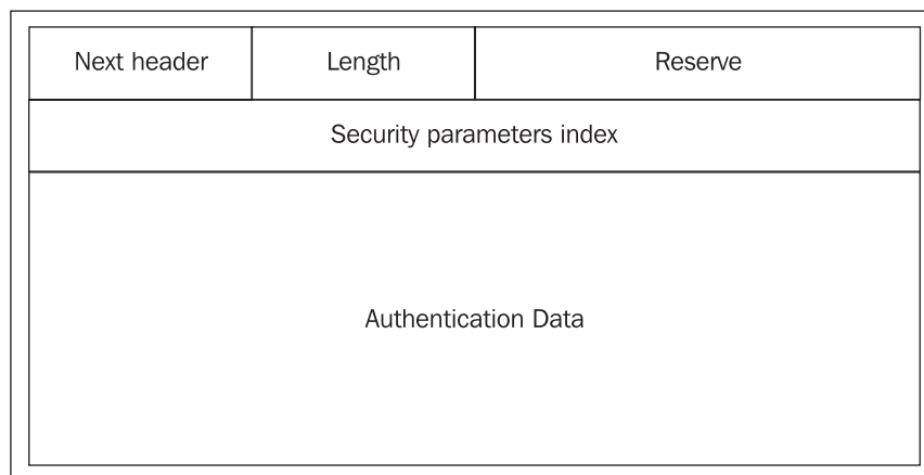
Figure 8.8: Authentication Header
