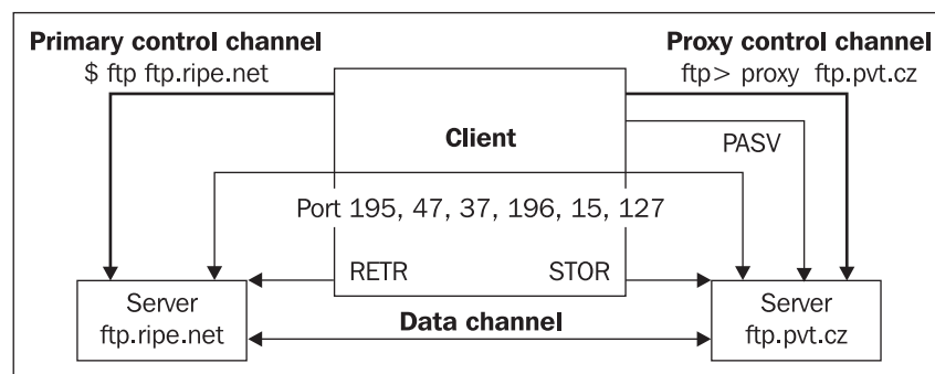
Figure 13.4: FTP proxy
