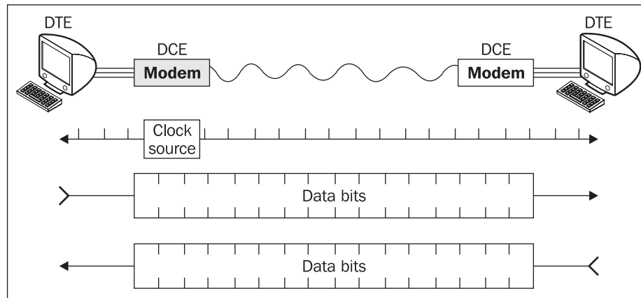
Figure 3.2: Synchronous transport
