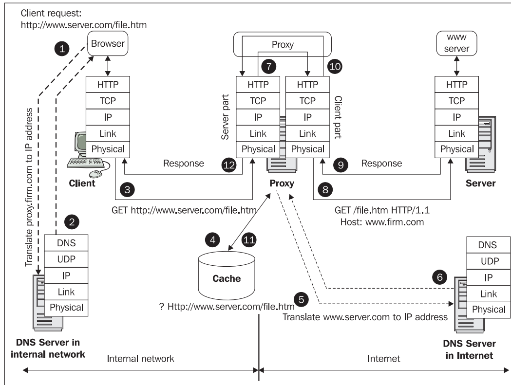
Figure 14.4: Proxy
