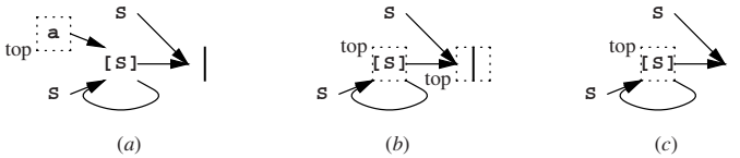
Fig. 11.12. Predictions with a non- \epsilon grammar loop
