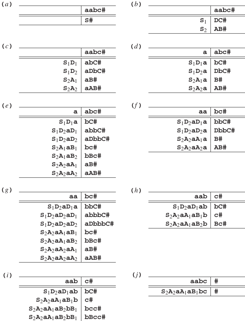
Fig. 6.8. The breadth-first parsing of the sentence aabc
