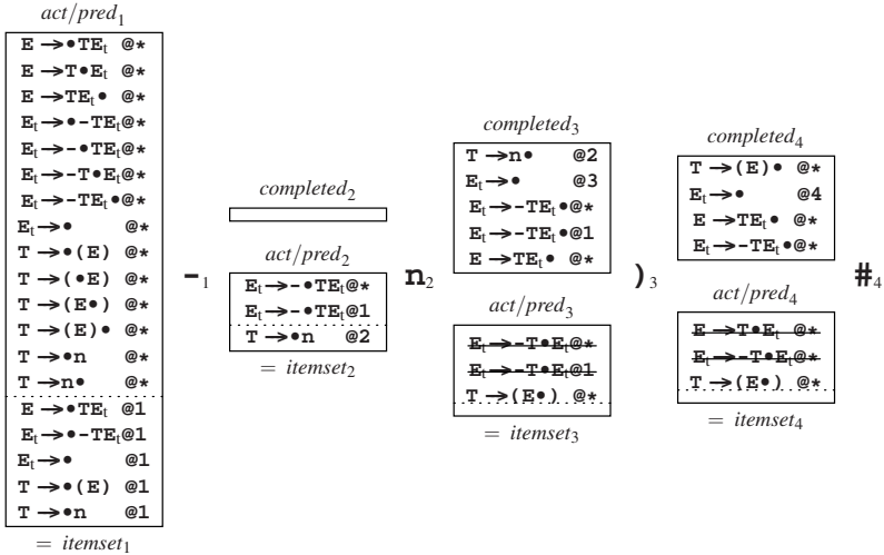
Fig. 12.11. Earley-on-LL(1) suffix parsing of (-n)
