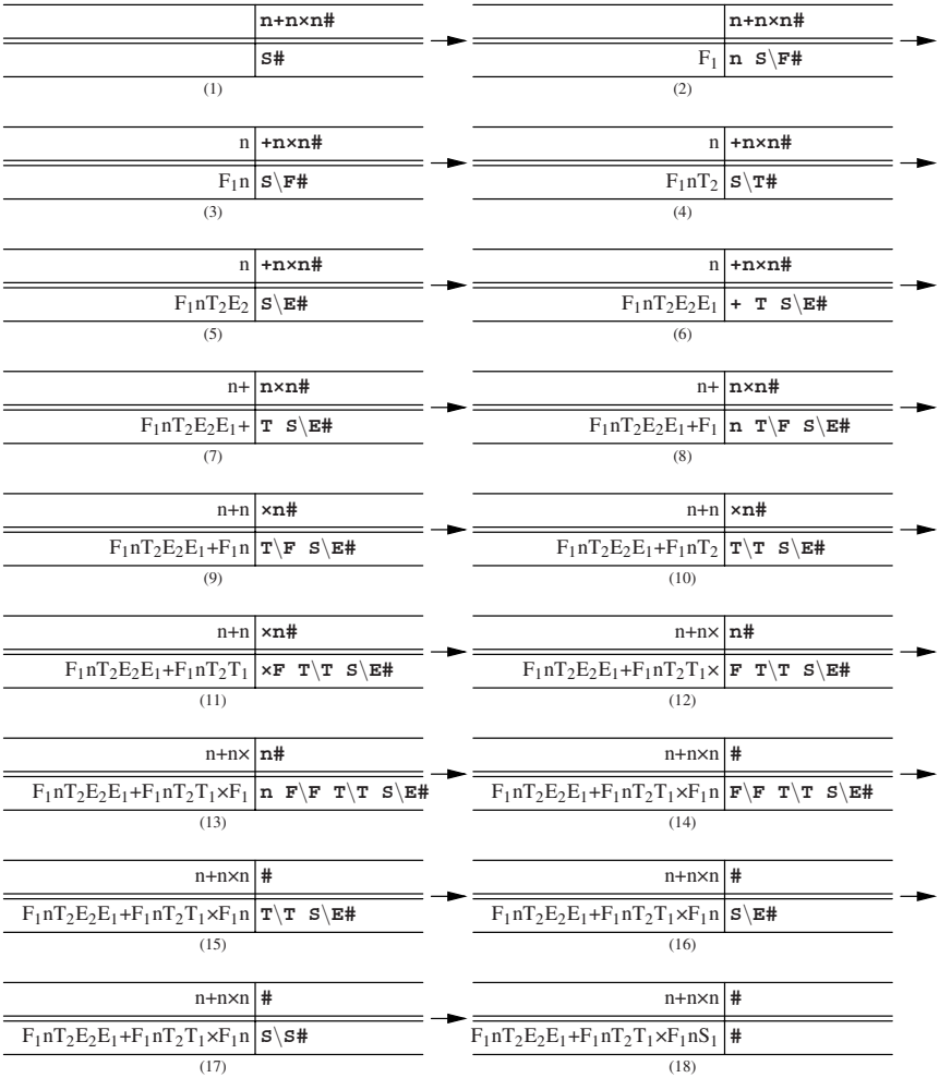
Fig. 10.5. Left-corner parsing of the input n+nxn
