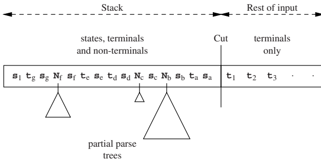
Fig. 9.12. The structure of an LR parse
