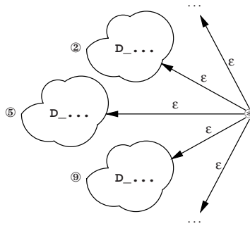
Fig. 9.47. Combined backwards-scanning automaton \overleftarrow{\mathcal{F}} for LR-regular parsing
