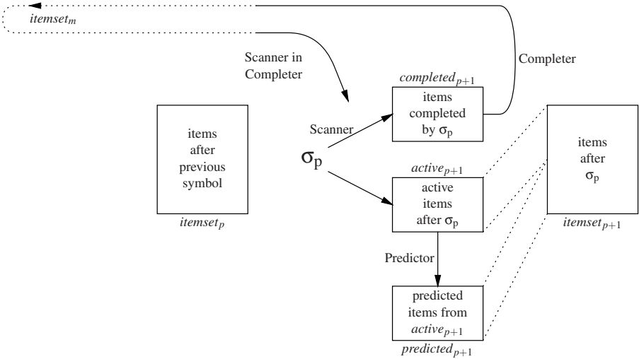
Fig. 7.10. The Earley item sets and their processes for one input symbol
