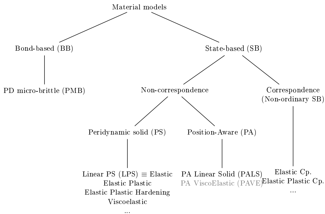
Figure 3.3.: Classification of peridynamic material models
