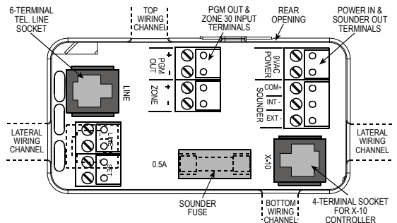
Figure 2. Sunken Wiring Area Layout
