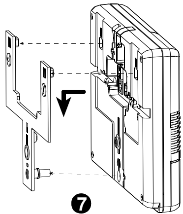
Figure 3 - Mounting
