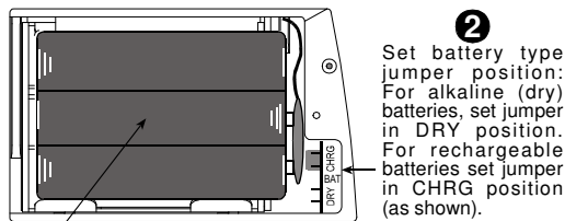
Figure 1. Backup Battery Insertion
