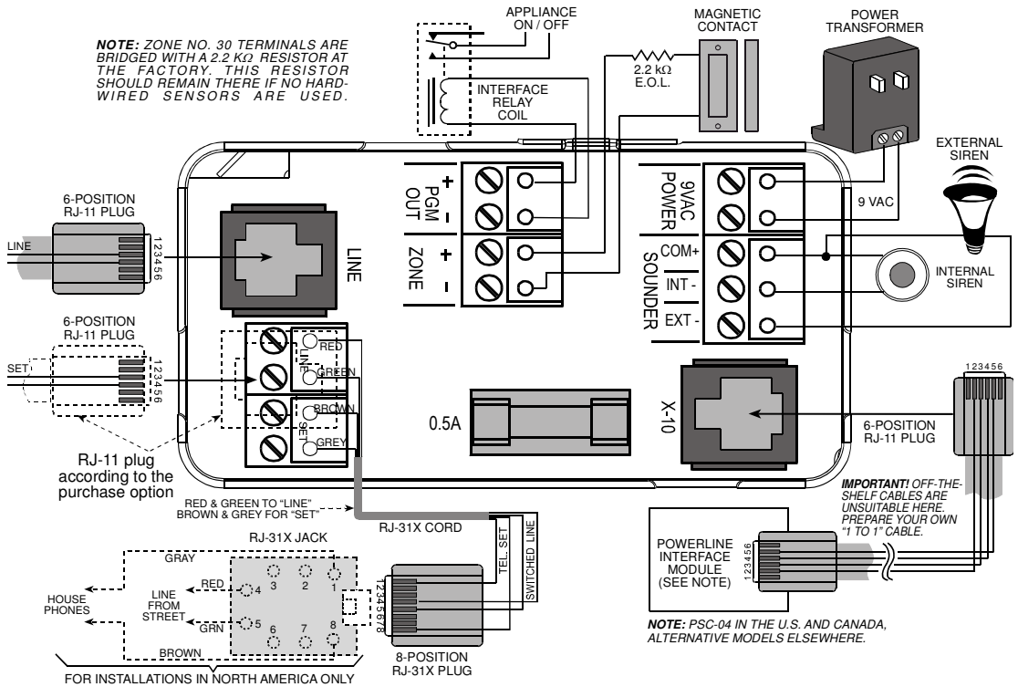
Figure 4. Wiring Diagram
