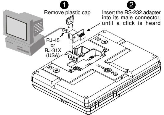
Figure 18. Inserting the RS232 Module
