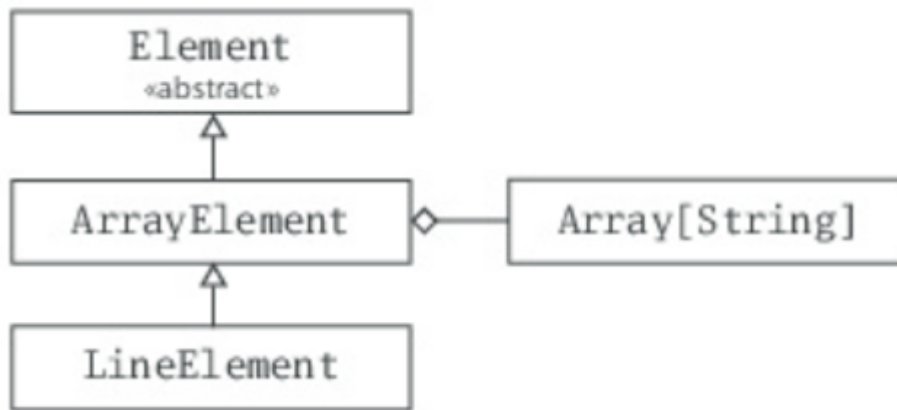
Figure 10.2 - Class diagram for LineElement.
