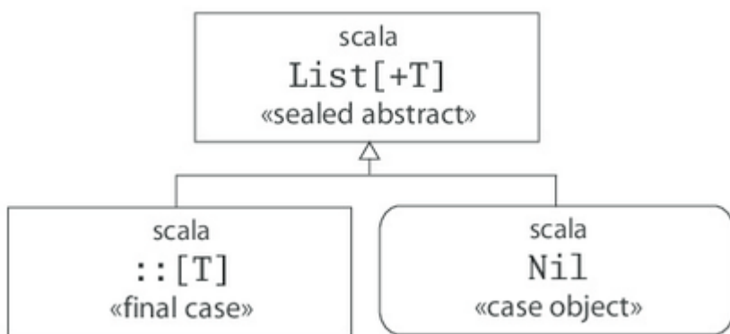
Figure 22.1 - Class hierarchy for Scala lists.
