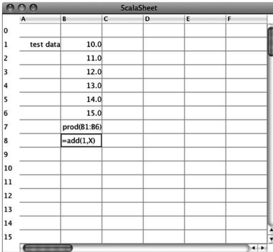
Figure 35.3 - Cells displaying their formulas.
