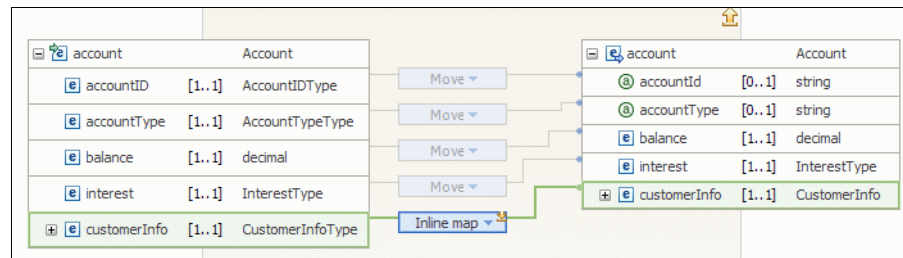
Figure 10-17 Account mapping
