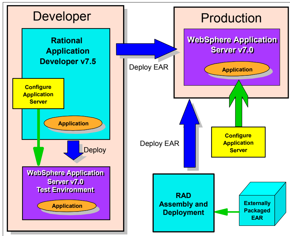
Figure 26-4 Deployment architecture
