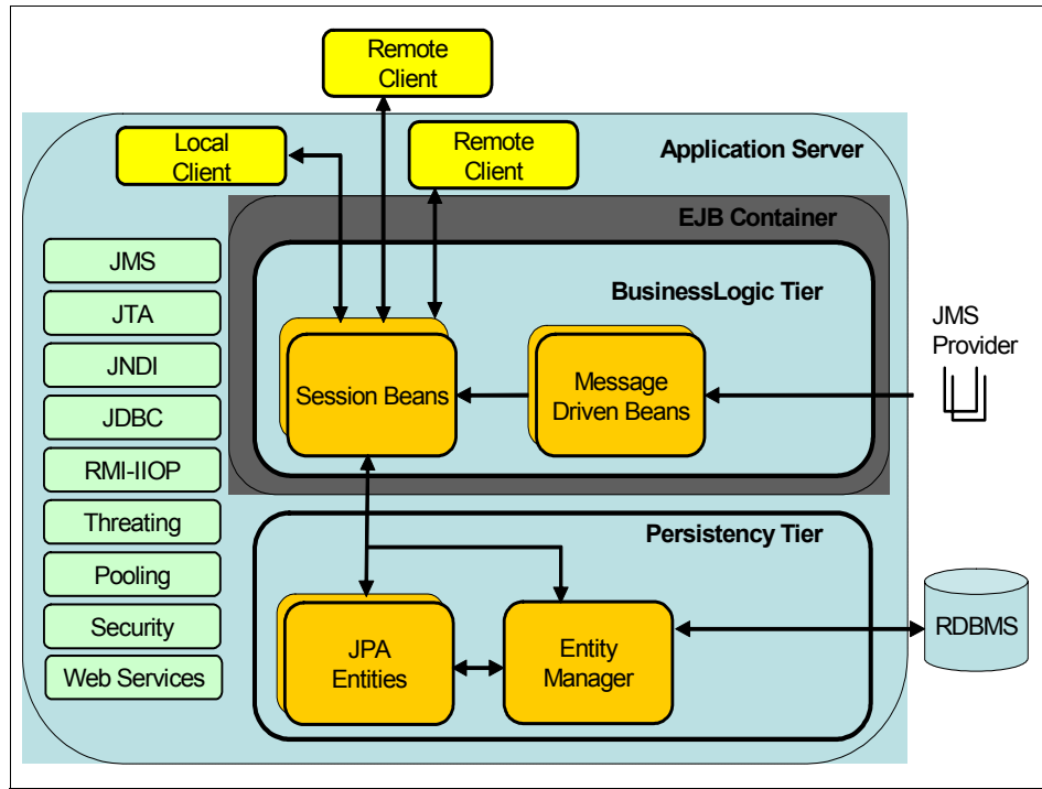
Figure 14-1 EJB 3.0 architecture
