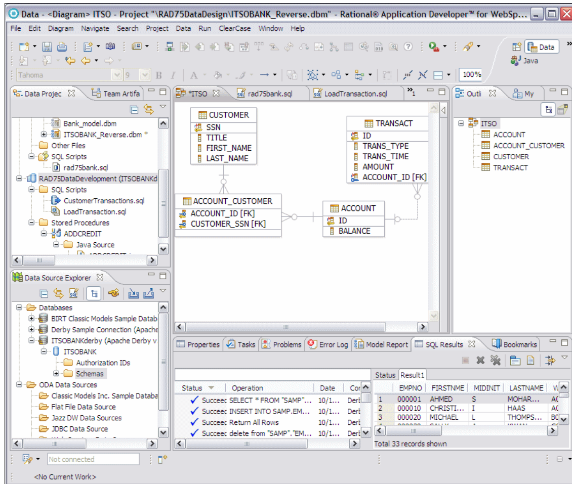
Figure 4-9 Data perspective
