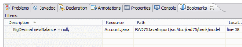
Figure 8-43 Bookmarks view
