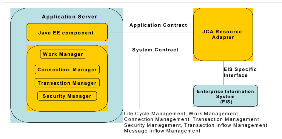
Figure 20-2 System contract, application server, resource adapter integration
