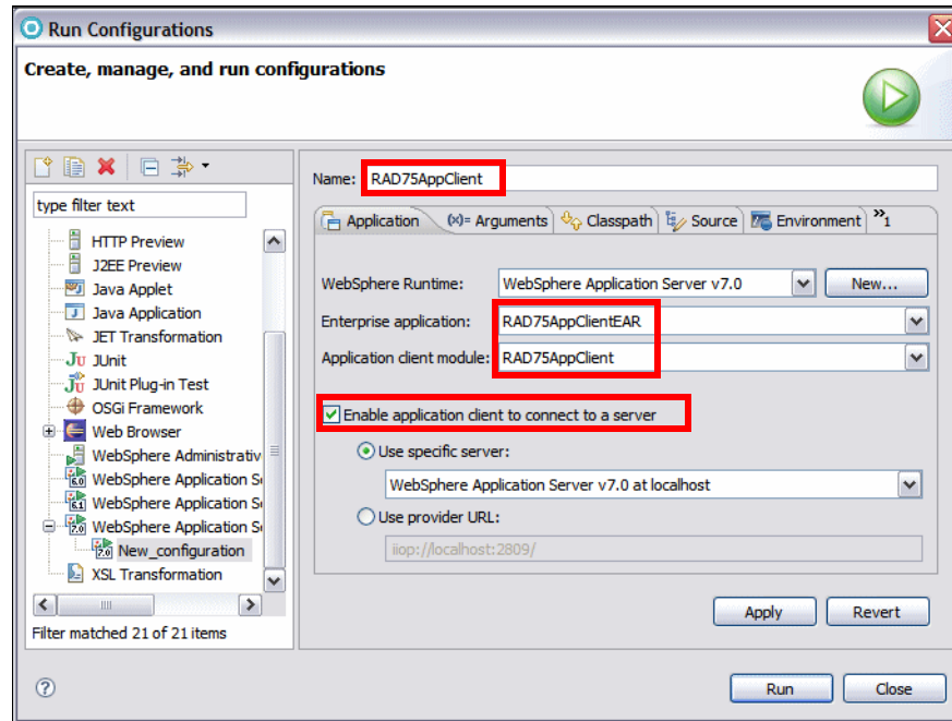
Figure 17-11 Create a new run configuration for the application client
