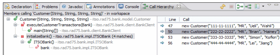
Figure 8-9 Call Hierarchy view [Callee Hierarchy]
