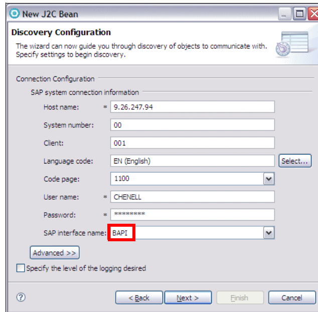
Figure 20-32 New J2C Bean - Discovery Configuration
