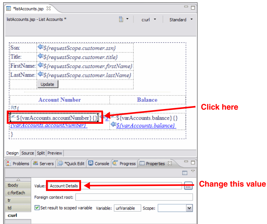
Figure 13-33 Configuring the AccountDetails URL
