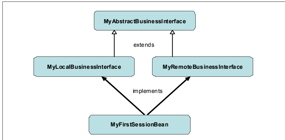
Figure 14-5 How to organize the EJB component interface
