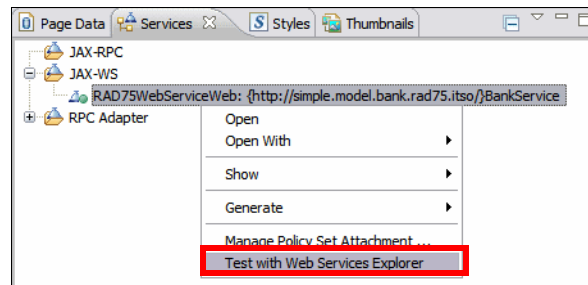
Figure 18-4 Test JAX-WS Web service using Web Services Explorer
