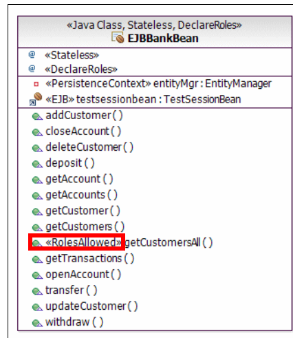
Figure 7-13 EJB 3.0 bean with method permissions on getCustomersAll method
