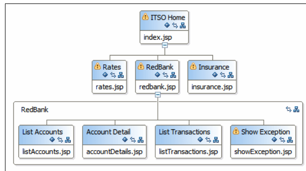
Figure 14-19 Web site navigation
