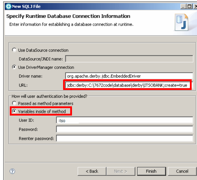
Figure 11-25 Specify Runtime Database Connection Information
