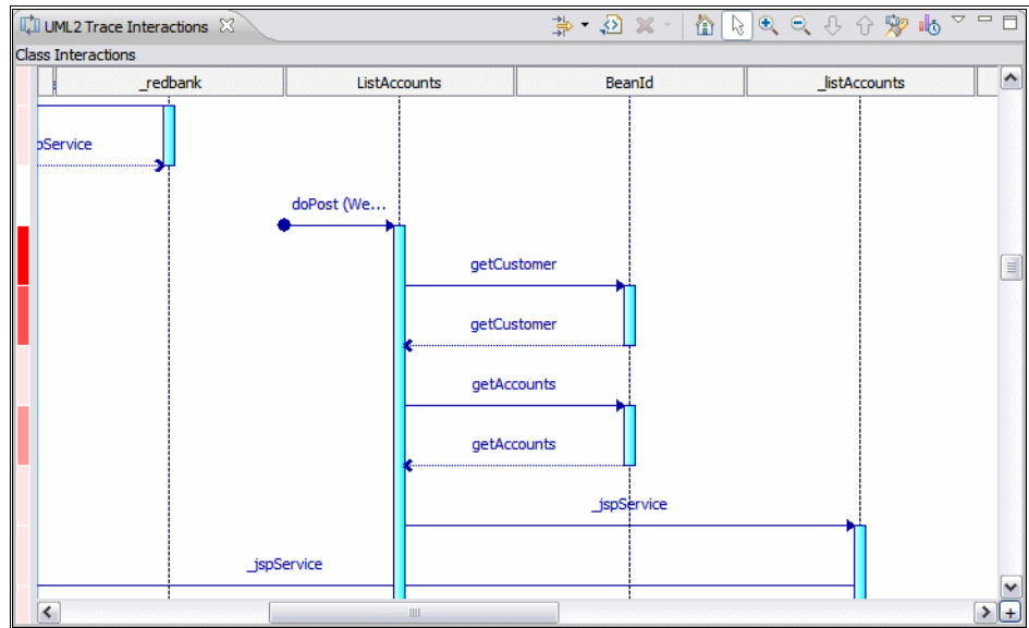
Figure 27-31 UML2 Class Interactions
