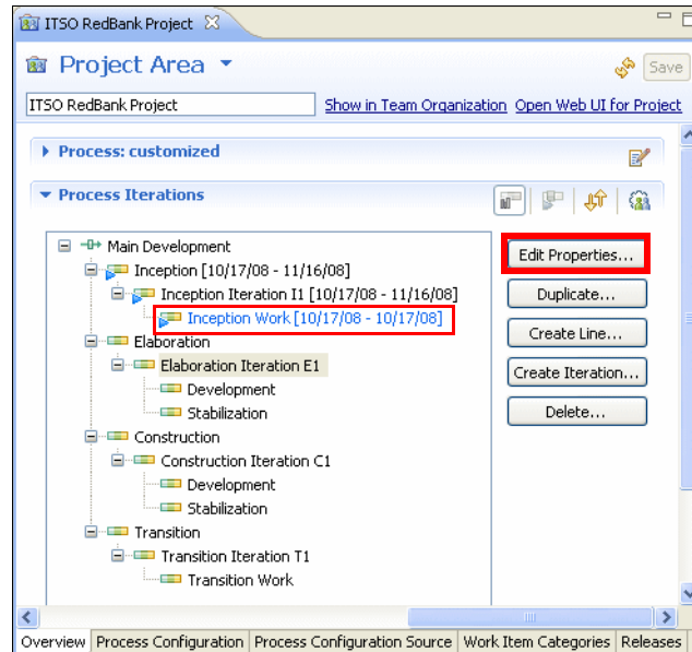
Figure 29-11 Define development lines, iterations, dates for the phases of the project
