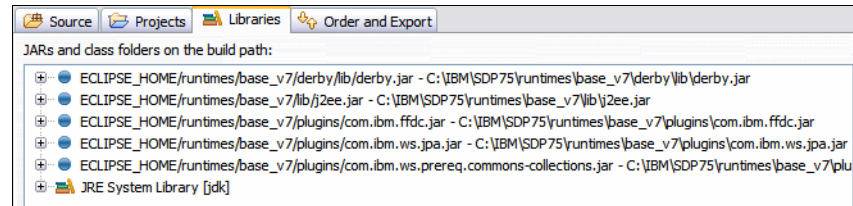
Figure 12-12 Library tab with five extra JAR files
