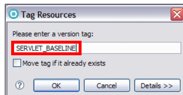
Figure 28-27 Tagging the project as a version
