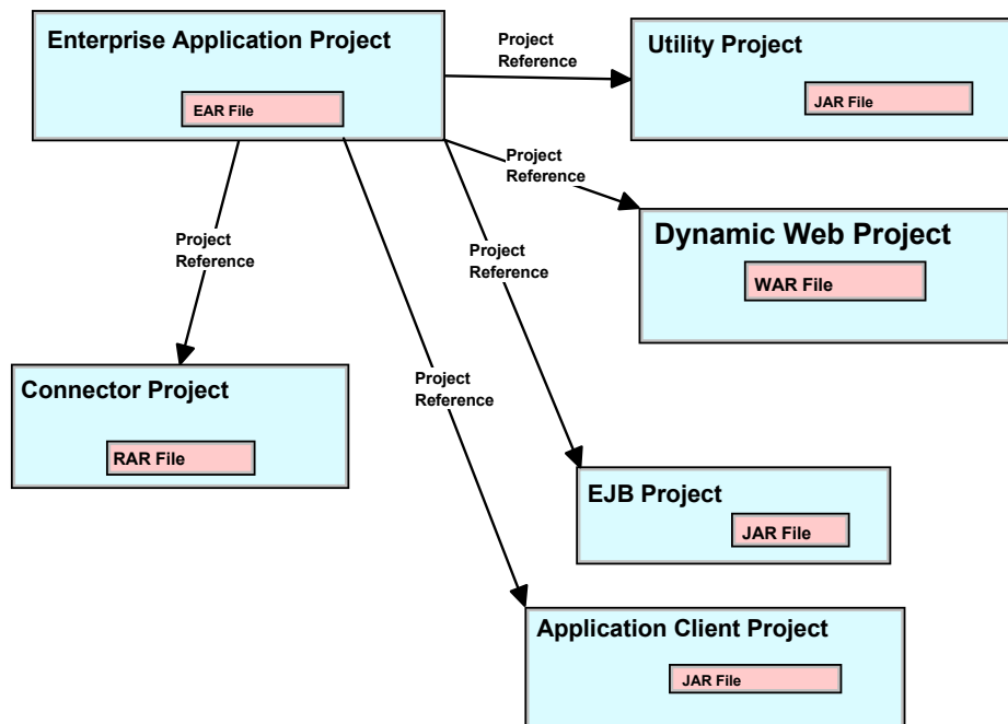
Figure 5-11 Java EE projects in Application Developer
