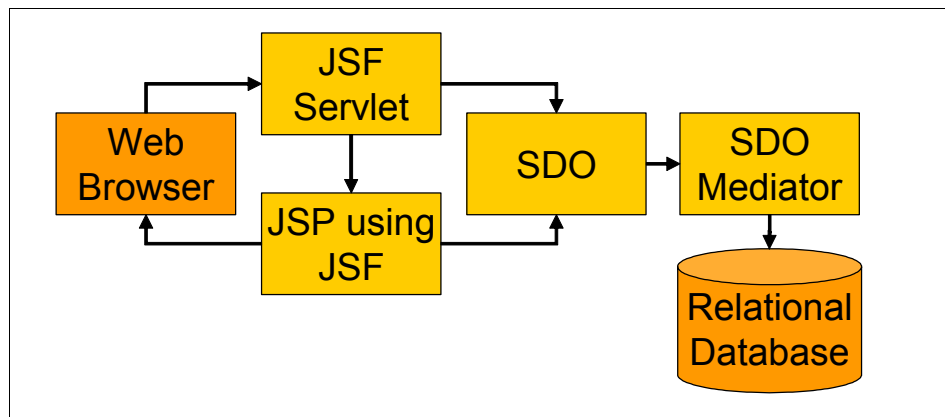
Figure 2-2 JSF and SDO
