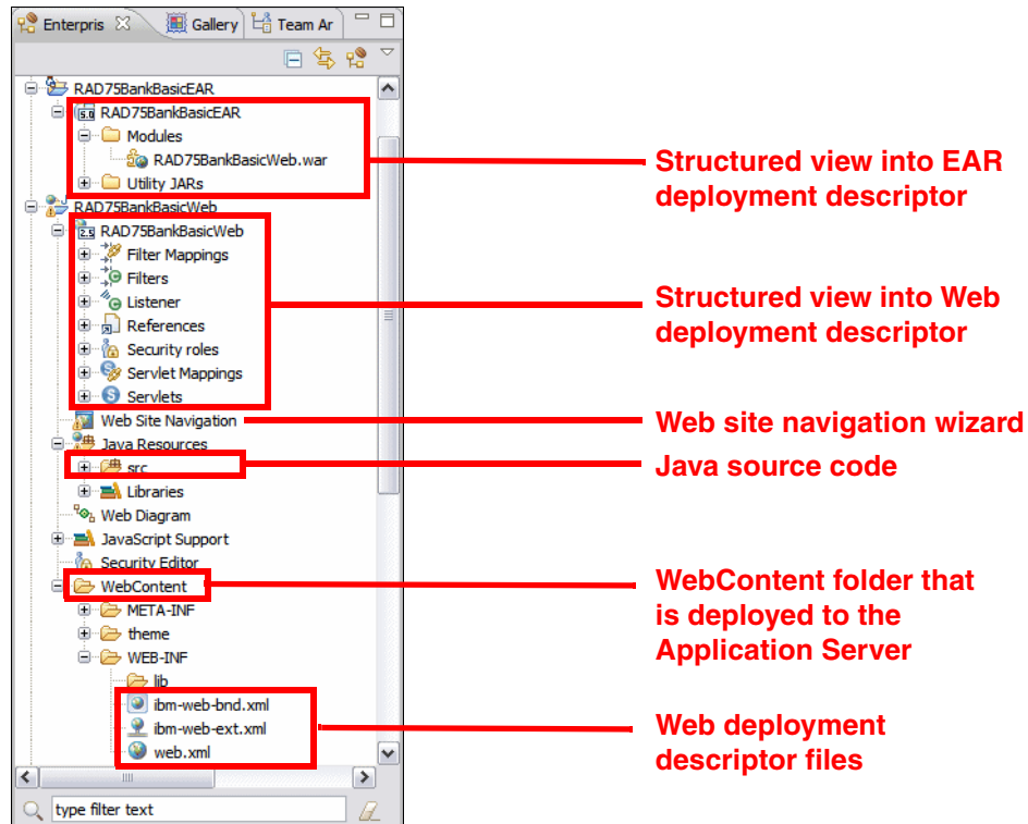
Figure 13-15 Web project directory structure
