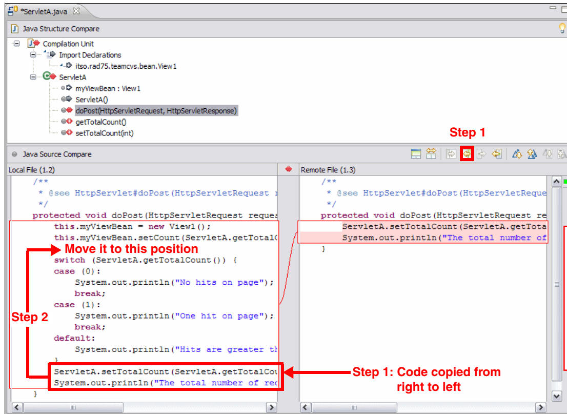
Figure 28-26 Merging changes from right to left
