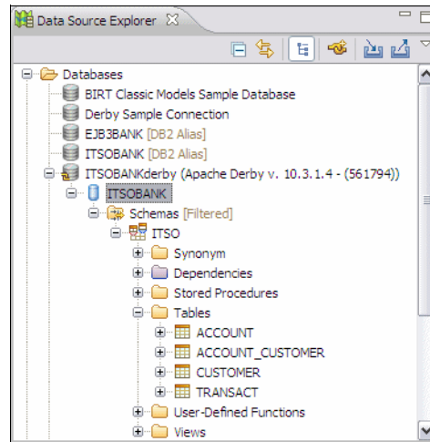
Figure 11-3 Connection with schema and tables in Data Source Explorer
