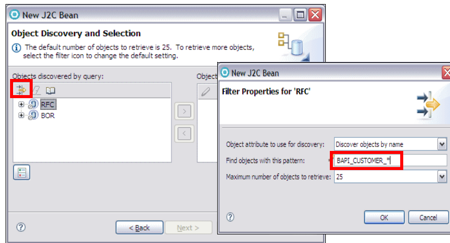
Figure 20-33 New J2C Bean - Object Discovery and Selection
