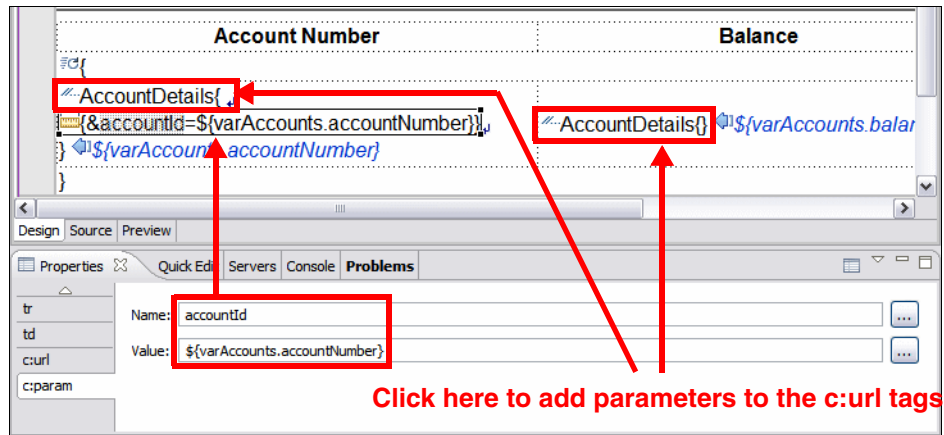
Figure 13-34 Adding parameters to c:url tags
