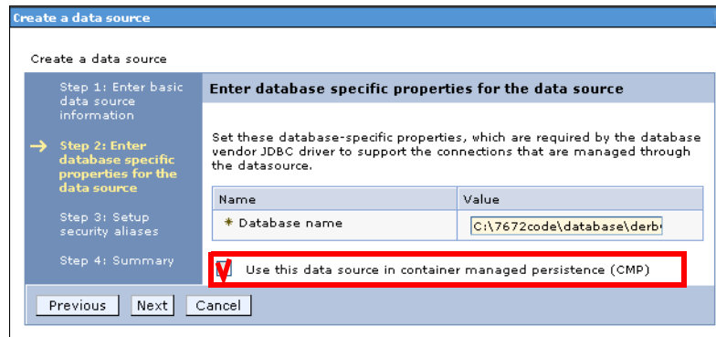
Figure 26-26 Enabling a data source to be used in CMP
