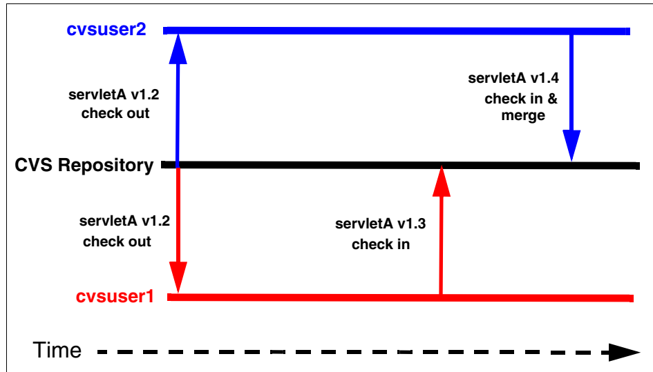
Figure 28-23 Parallel concurrent development of same resource by multiple developers
