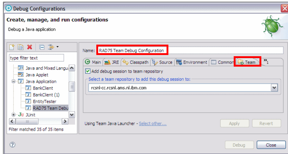
Figure 24-21 Debug configuration for a Java Application to be added to team repository
