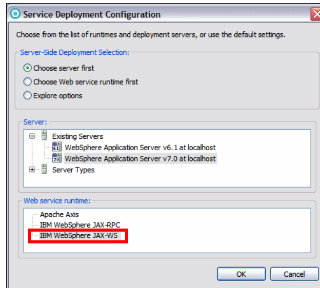
Figure 18-7 Web Service wizard: Service Deployment Configuration
