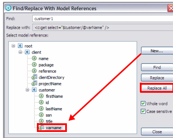
Figure 9-18 Replace all occurrences of customer
