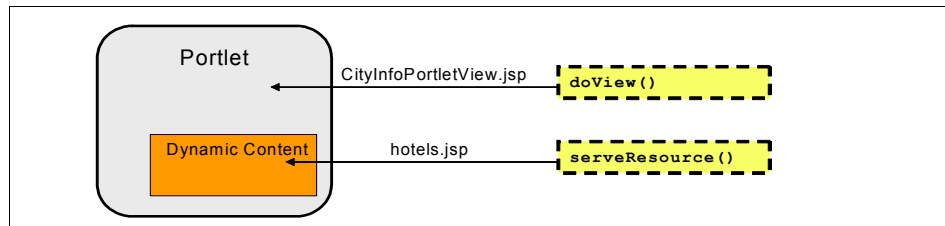
Figure 21-23 Resource serving portlet to add city hotels
