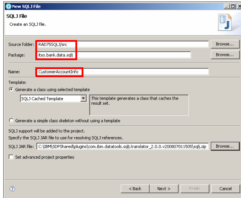
Figure 11-23 New SQLJ File
