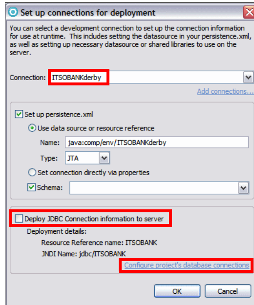
Figure 16-10 Deployment of JDBC connection
