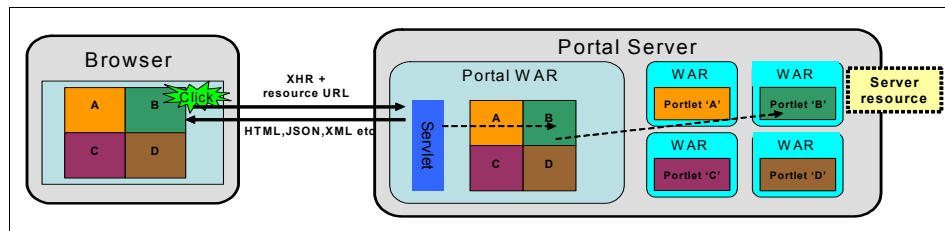
Figure 21-22 Portlet with Ajax support
