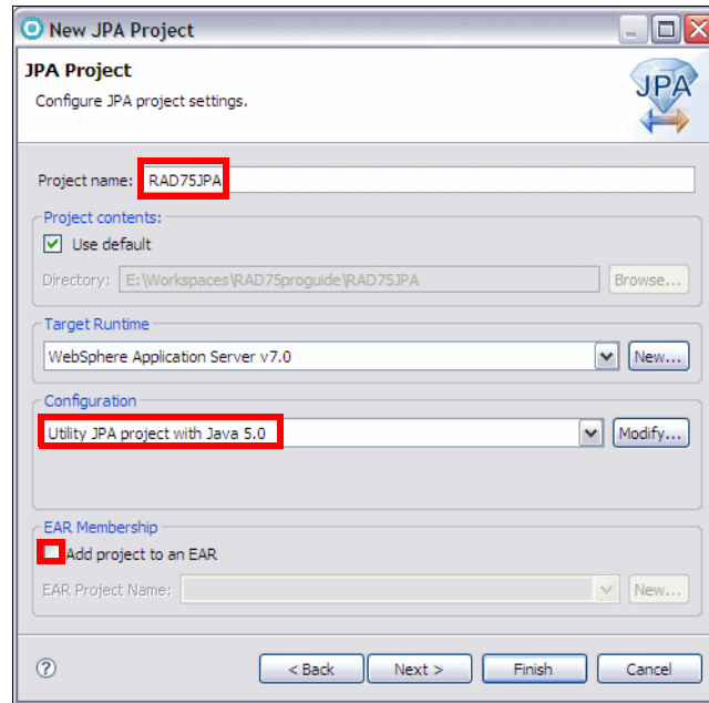
Figure 12-1 New JPA Project
