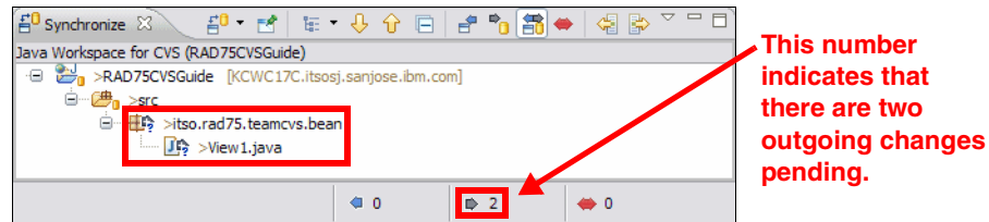
Figure 28-19 Synchronizing RAD75CVSGuide after creating the viewbean View1
