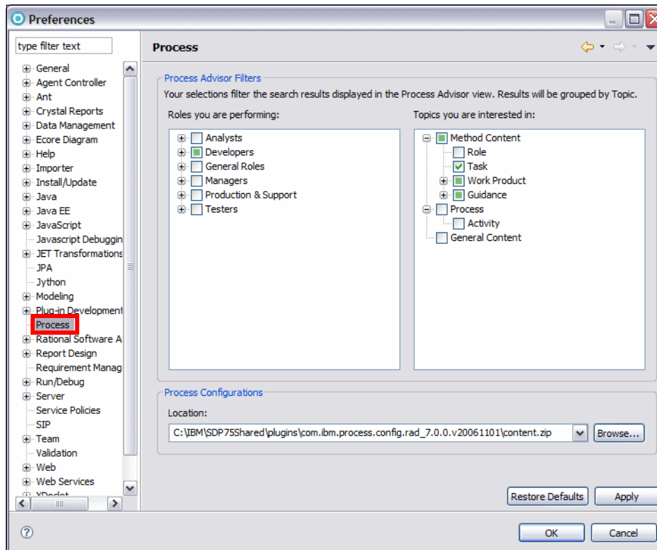
Figure 6-5 Process preferences
