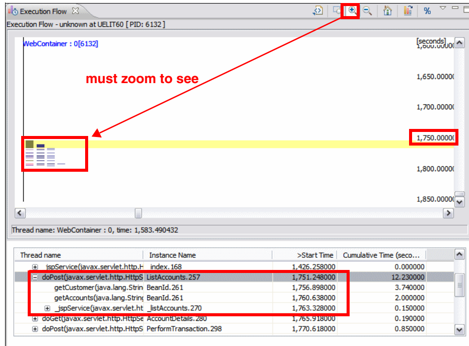
Figure 27-29 Execution Flow
