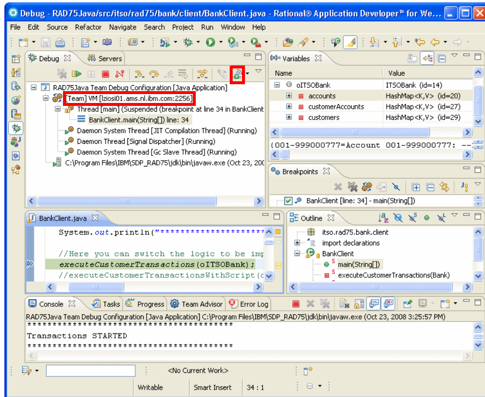
Figure 24-22 Team Debugging
