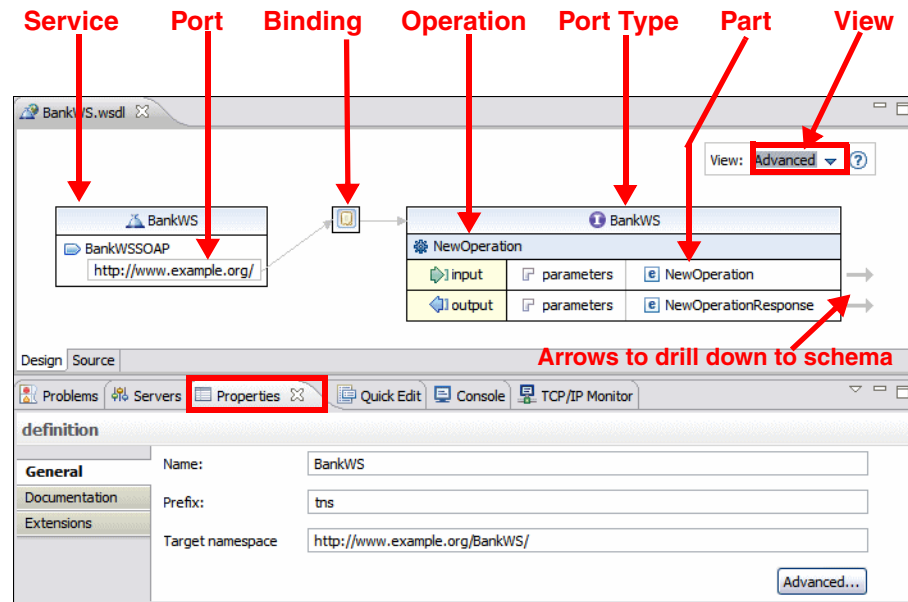
Figure 18-33 WSDL editor
