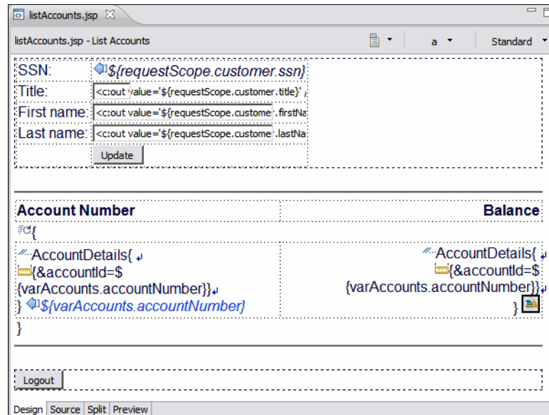
Figure 13-36 listAccounts.jsp finished
