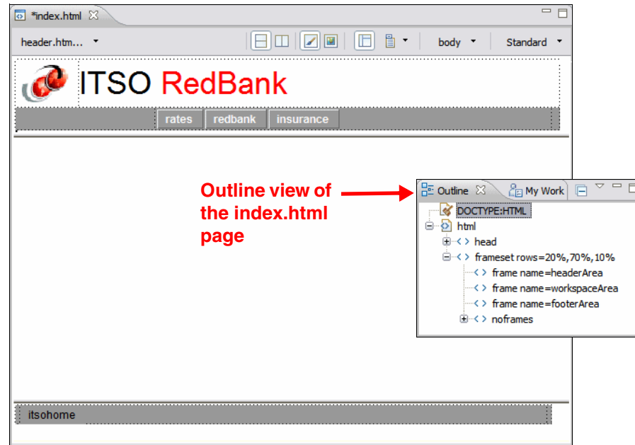
Figure 13-20 Frame design
