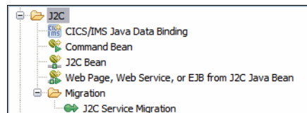
Figure 20-3 J2C wizards
