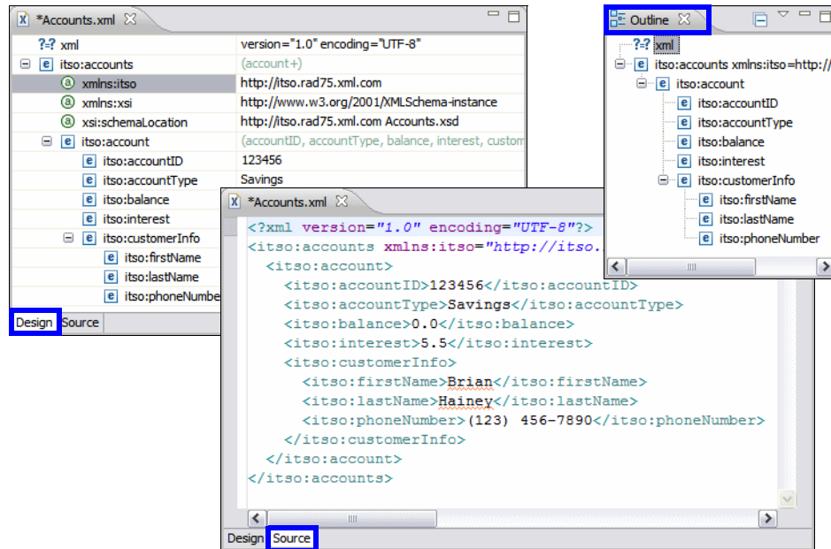
Figure 10-8 Design view, Source view, and Outline view
