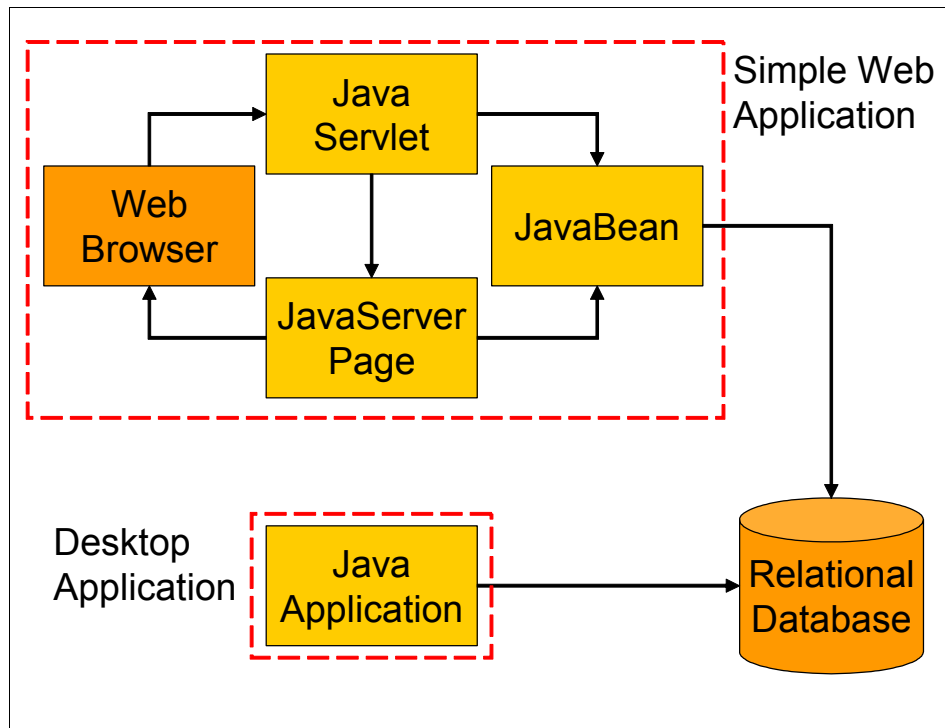
Figure 2-1 Simple Web application
