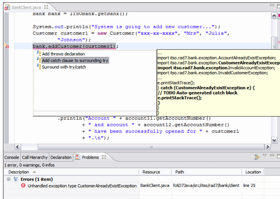
Figure 8-51 Java Editor with quick fix
