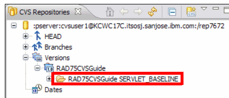
Figure 28-28 Repository view showing new project revision
