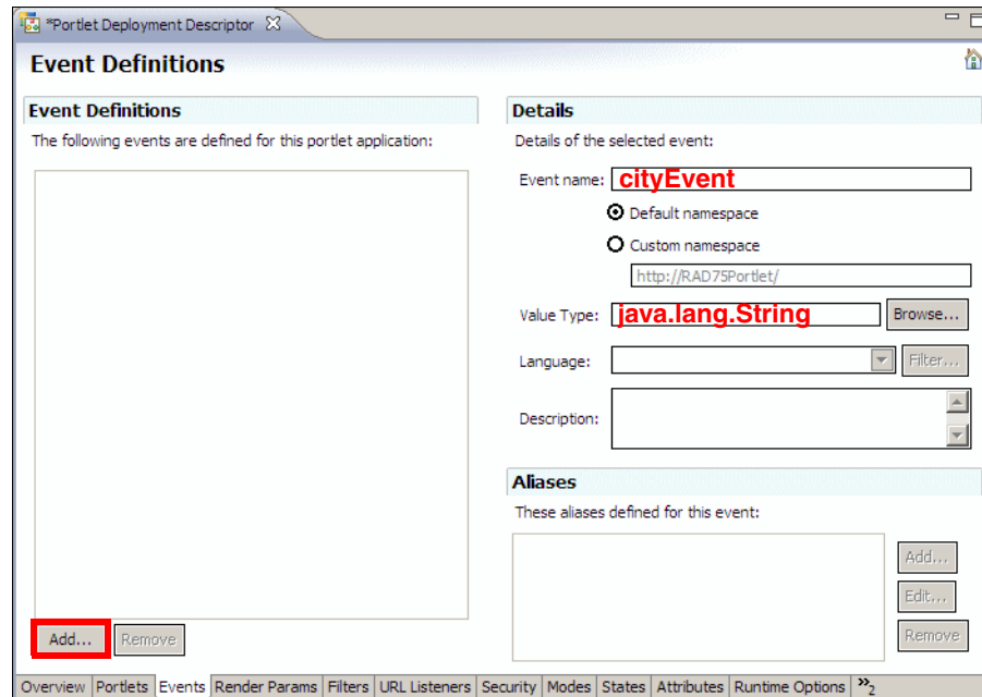
Figure 21-15 Portlet Deployment Descriptor: Events
