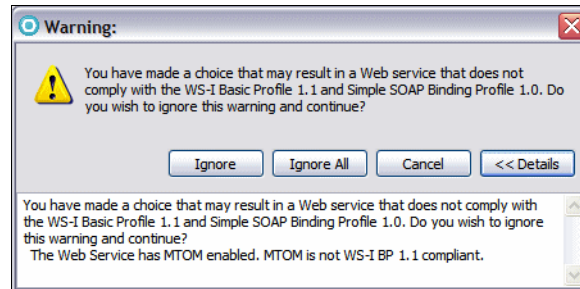
Figure 18-44 WS-I warning against MTOM
