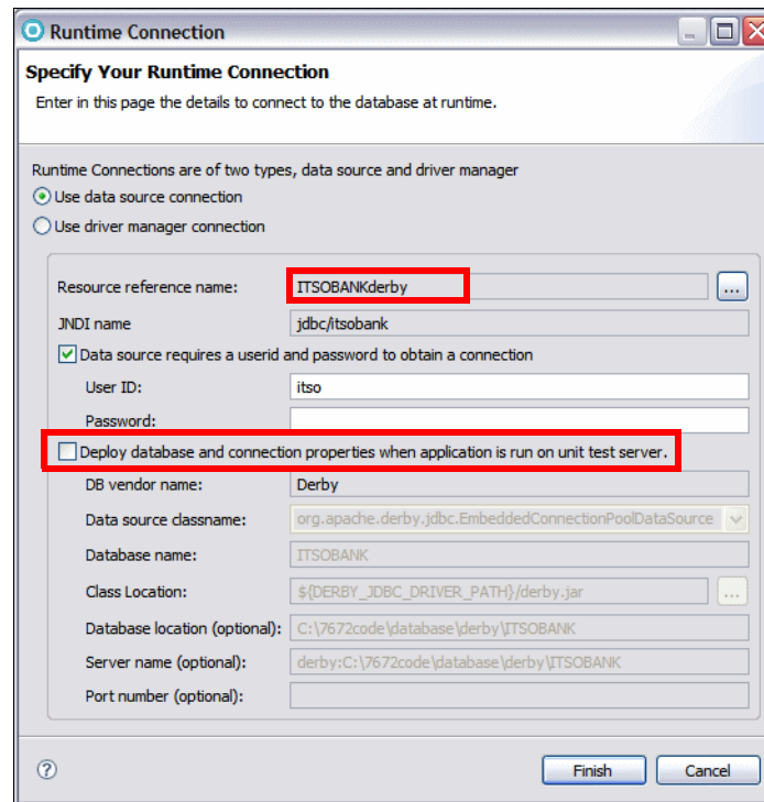
Figure 16-12 Deployment of the runtime connection
