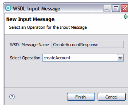
Figure 7-26 WSDL Input Message wizard
