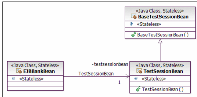
Figure 7-10 Class diagram showing three EJB 3.0 session beans with relationships.
