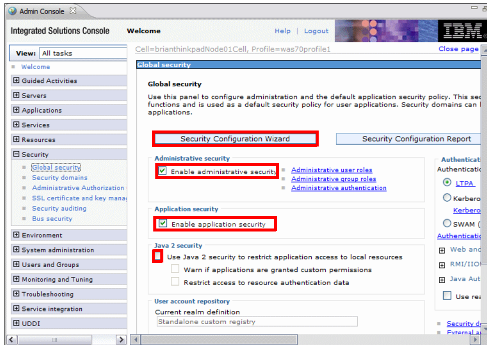
Figure 22-21 Configuring security
