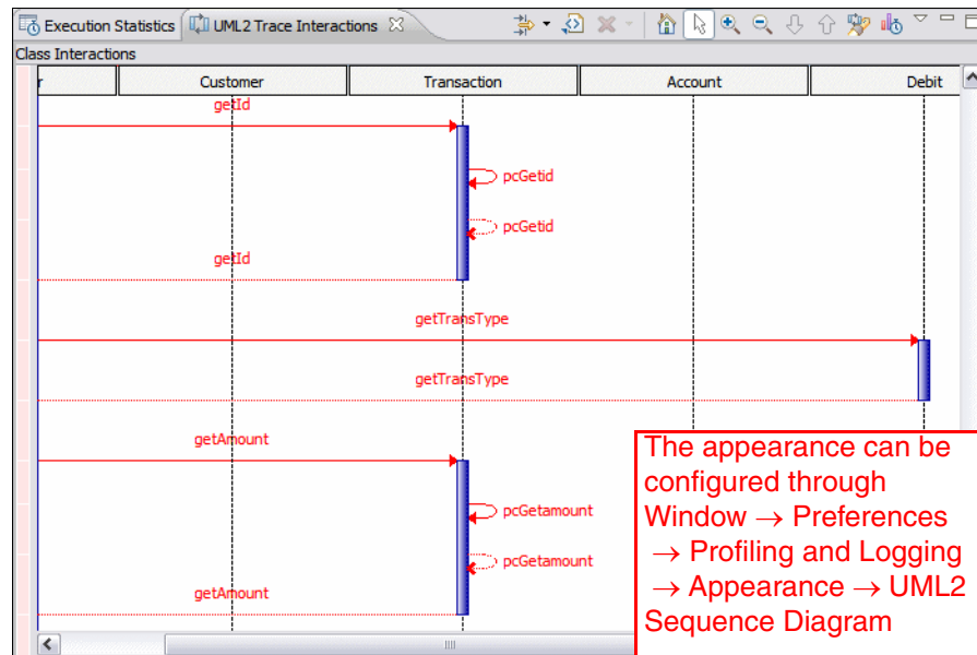
Figure 27-16 UML2 Interaction
