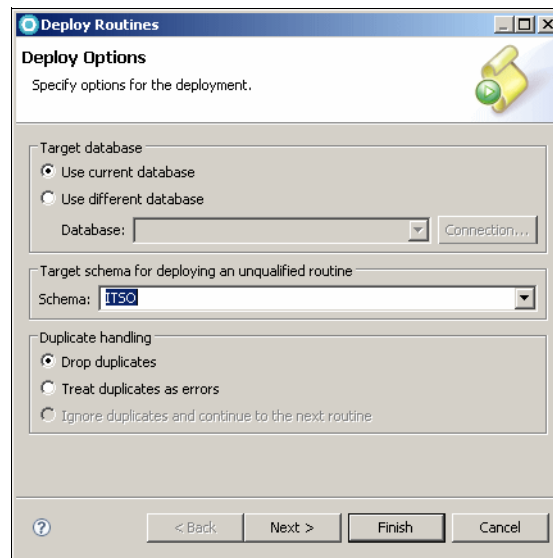
Figure 11-21 Deploy Routines
