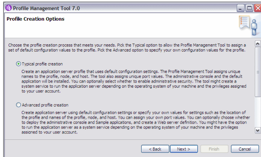
Figure 22-5 Profile options
