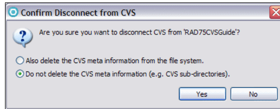
Figure 28-43 Disconnect confirmation
