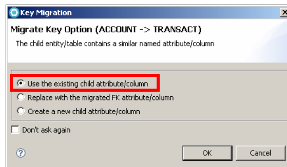
Figure 11-35 Key migration
