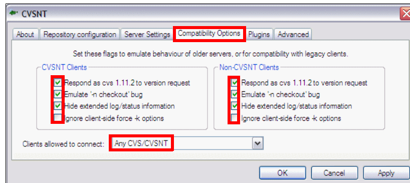
Figure 28-3 Compatibility options
