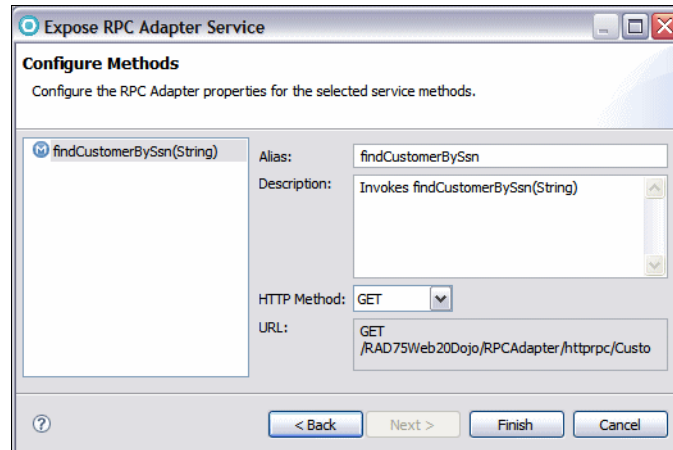
Figure 19-10 Configure Methods
