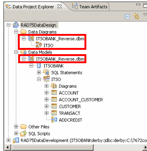
Figure 11-29 Data Design Project with physical model and diagram
