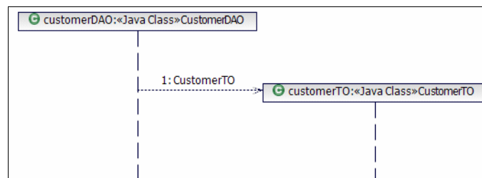
Figure 7-36 Sending a create message to create a new lifeline during an interaction
