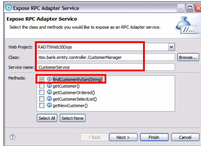
Figure 19-9 Exposing a service
