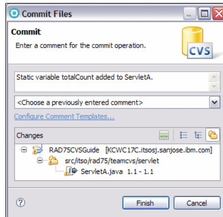
Figure 28-22 Adding comment for changes to ServletA
