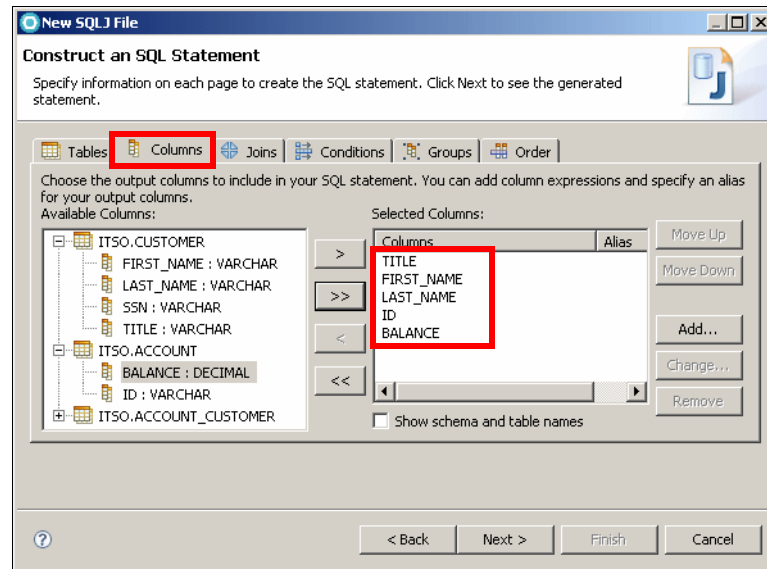
Figure 11-24 Select the output columns
