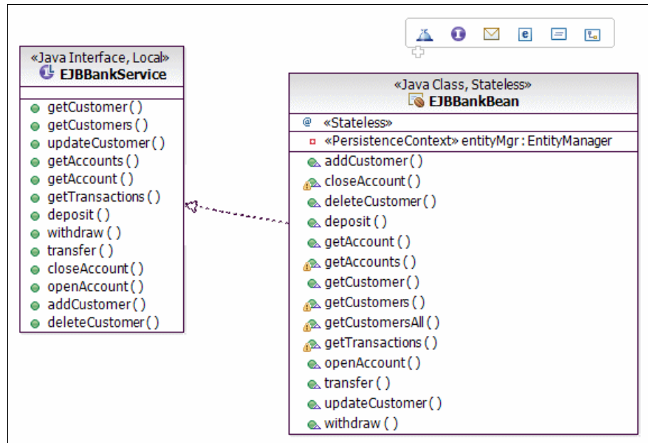
Figure 7-8 Visualization of an EJB 3.0 Enterprise JavaBeans
