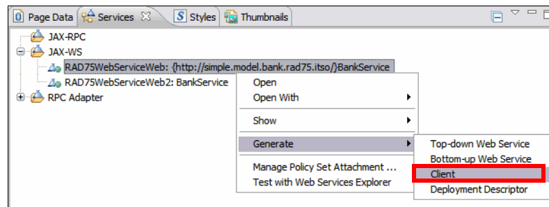
Figure 18-11 Generate Web service client
