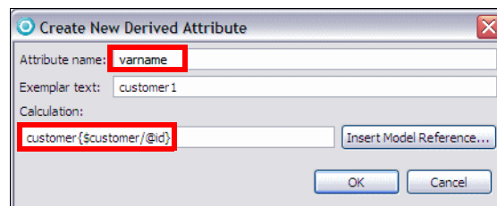
Figure 9-17 Creating the varName derived attribute
