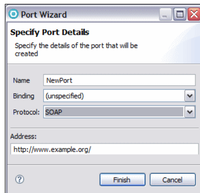
Figure 7-17 Port wizard
