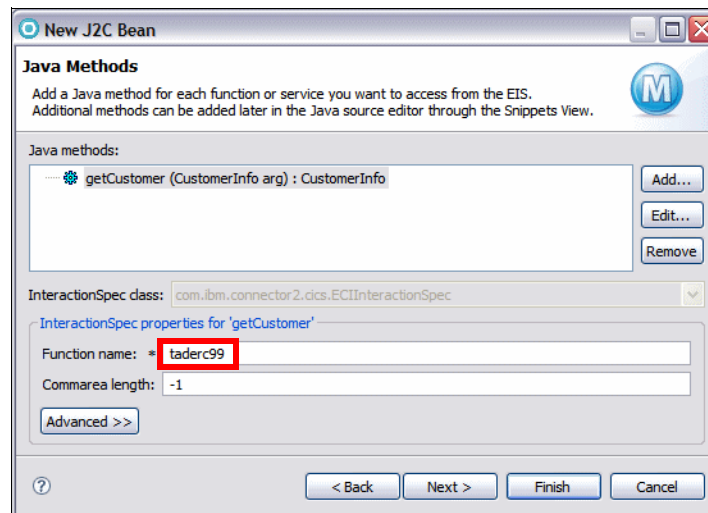
Figure 20-8 InteractionSpec properties
