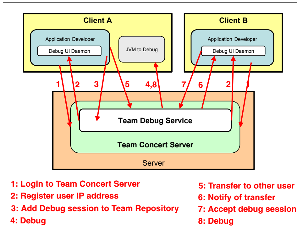
Figure 24-20 Workflow for transferring Java Debug session
