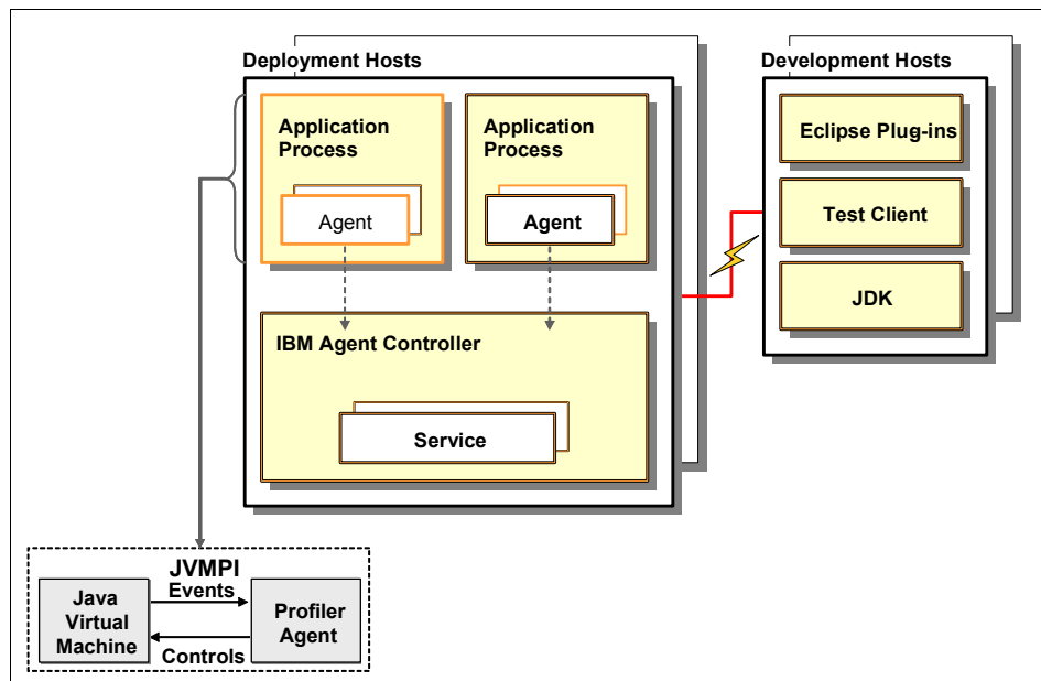
Figure 27-1 Profiling architecture of IBM Rational Application Developer V7.0
