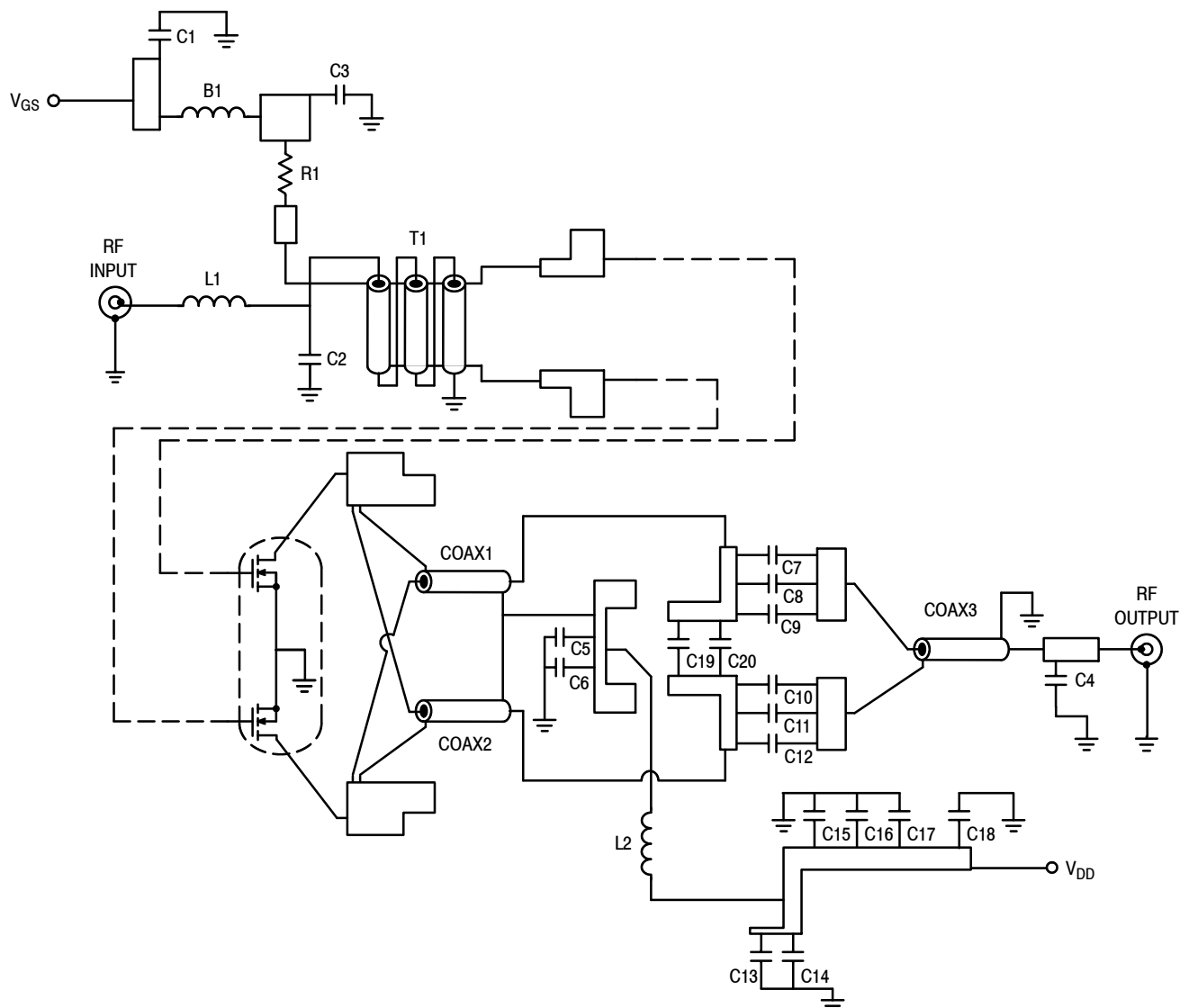
Figure 3. 2 Meter Amateur Reference Design Schematic Diagram
