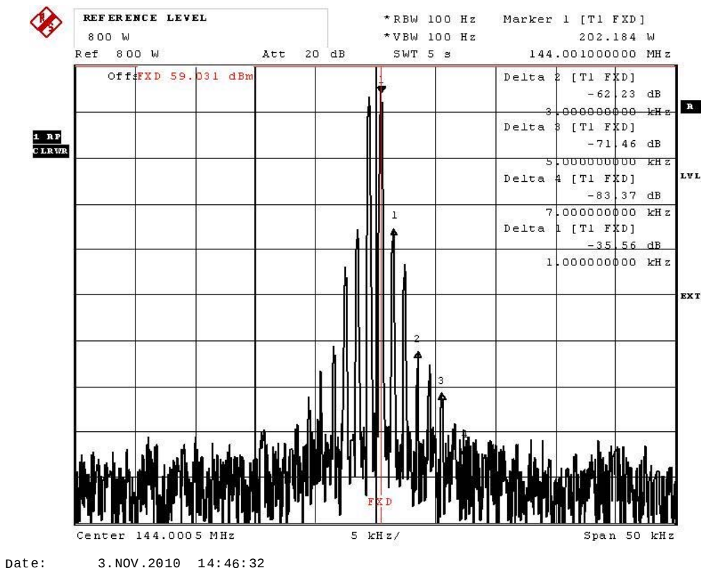
Figure 7. 800 W Two-Tone Spectrum
