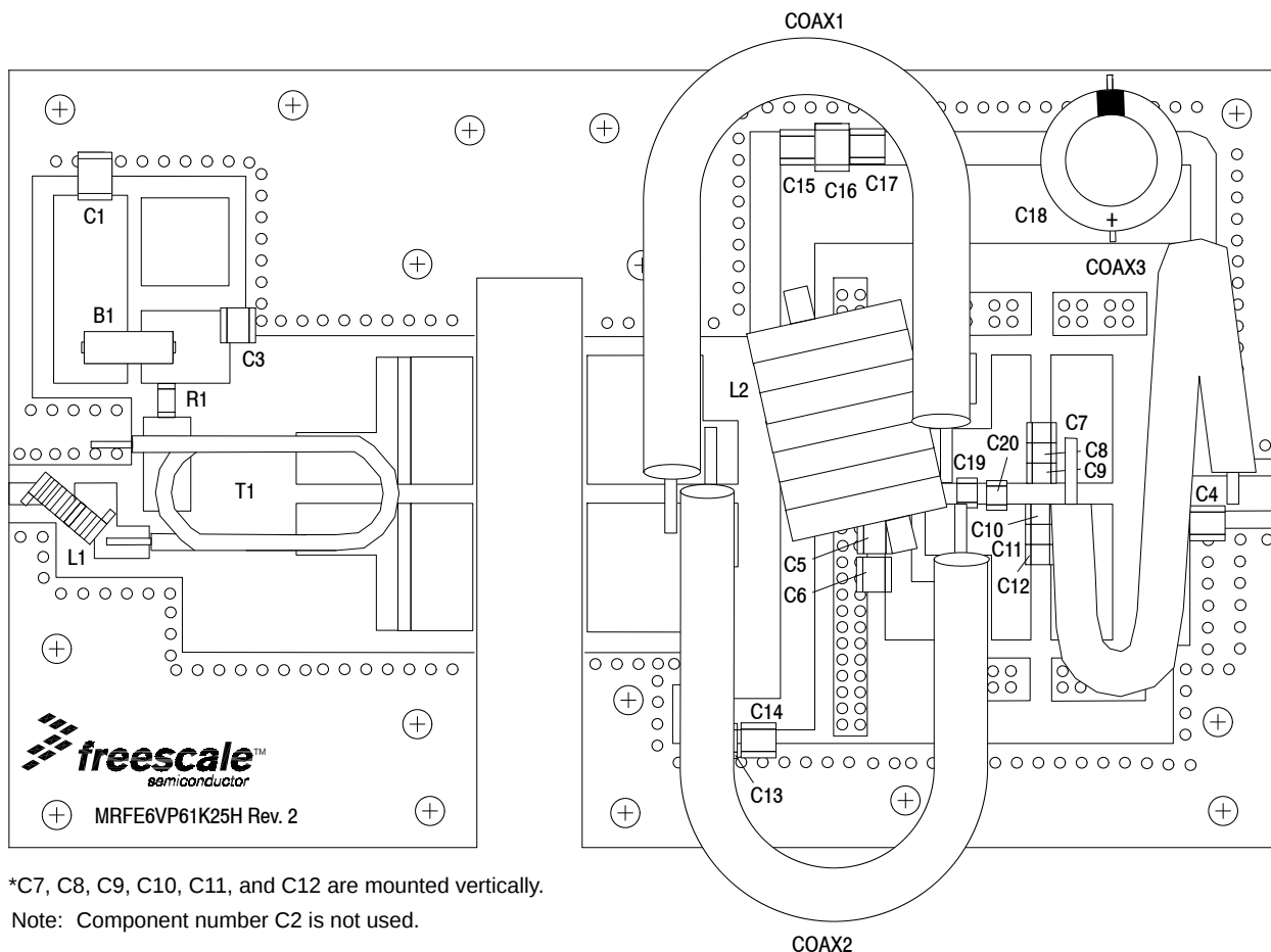
Figure 4. 2 Meter Amateur Reference Design Component Layout
