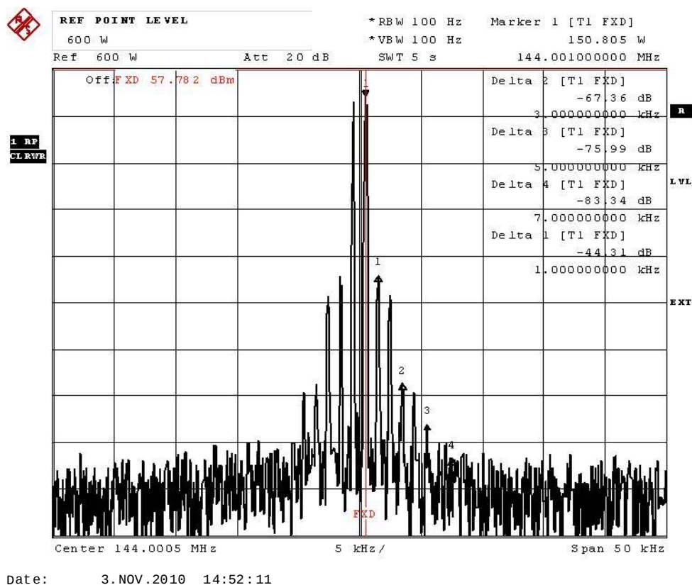
Figure 8. 600 W Two-Tone spectrum
