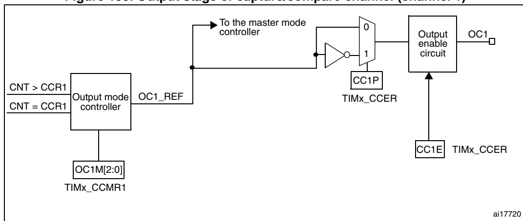
Figure 195. Output stage of capture/compare channel (channel 1)
