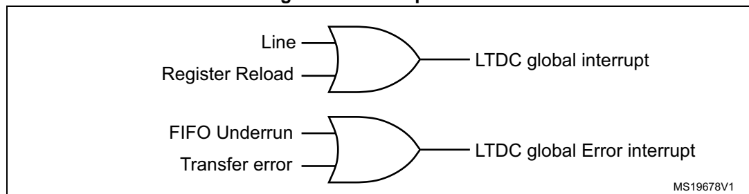
Figure 85. Interrupt events
