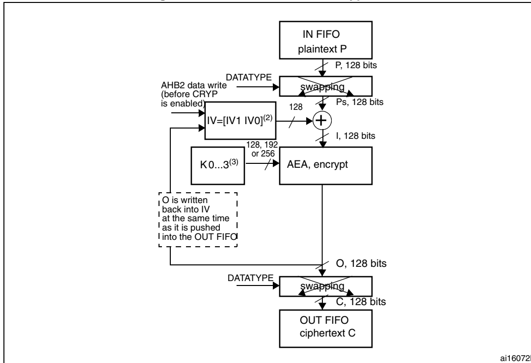
Figure 224. AES-CBC mode encryption
