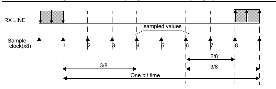
Figure 302. Data sampling when oversampling by 8
