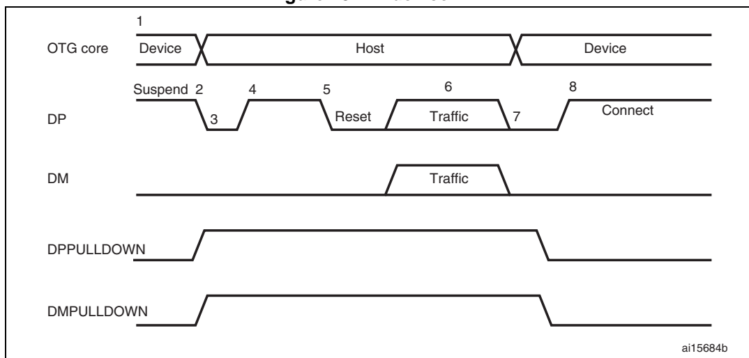
Figure 431. B-device HNP
