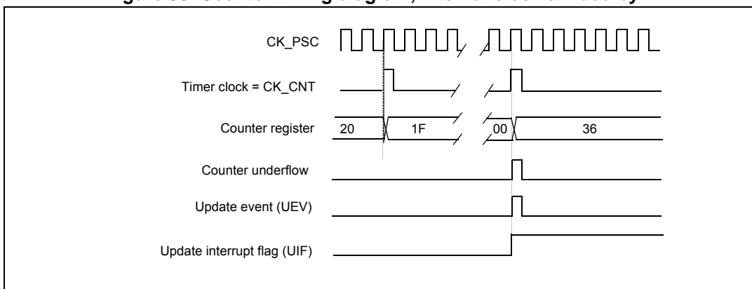
Figure 98. Counter timing diagram, internal clock divided by N
