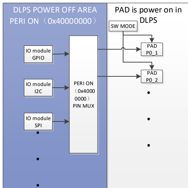
Figure 20.3 Peripherals and PAD Circuits Diagram
