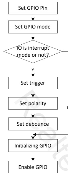
Figure 20.2 GPIO Initialization Flow Chart
