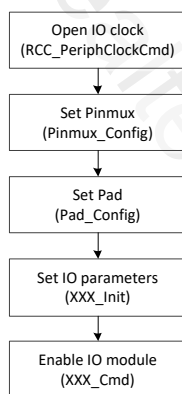
Figure 20. 1 Initialization Flow Chart
