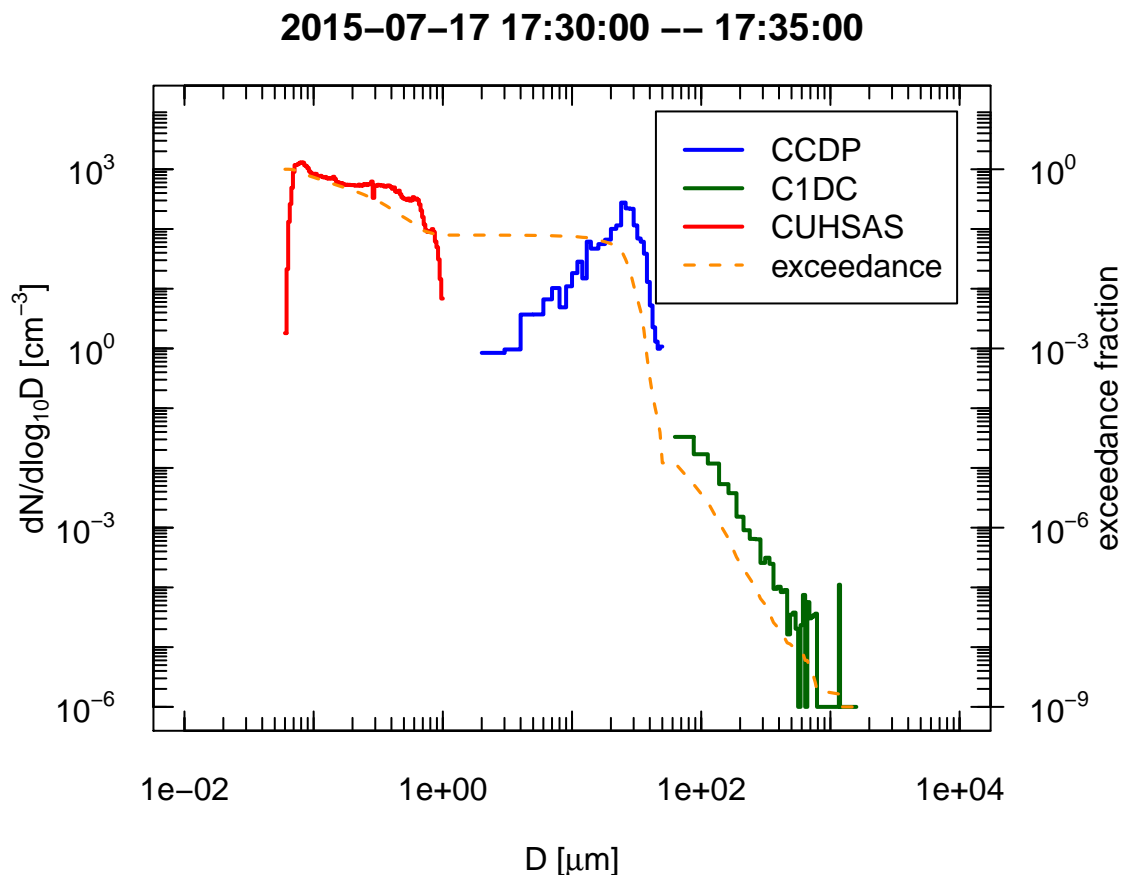
Figure 2: Size distribution measured during the CSET project, research flight 6, 17:30:00 – 17:35:00 UTC.
