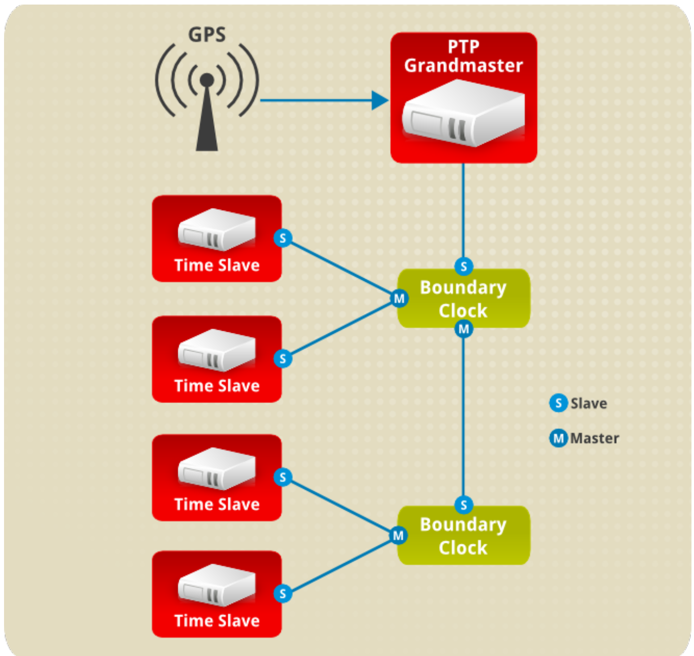
Figure 22.1. PTP grandmaster, boundary, and slave Clocks
