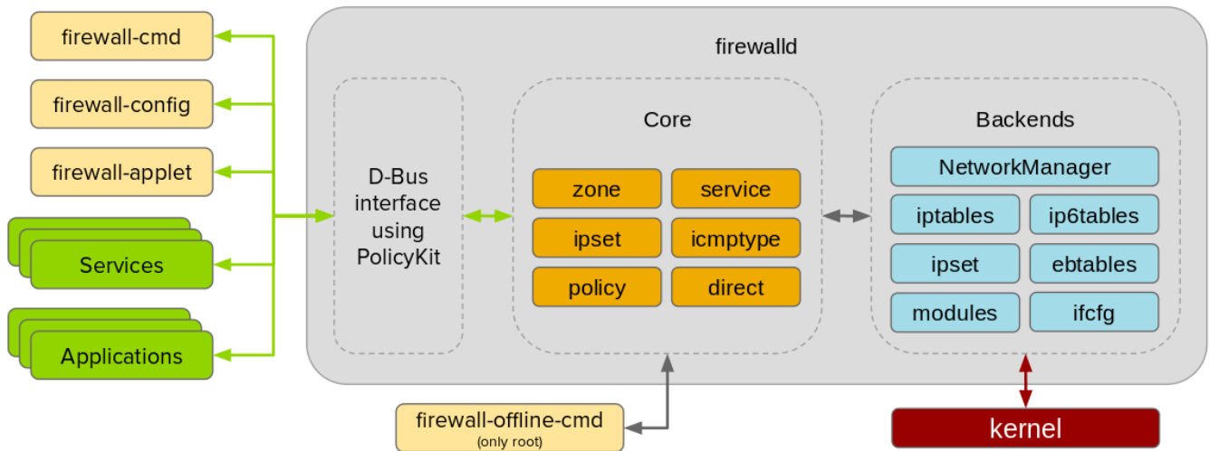
Figure 4.3. The firewalld Architecture
