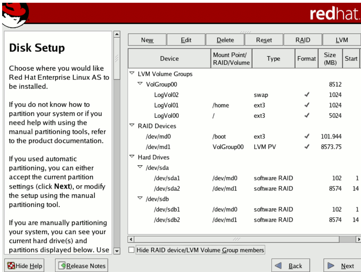
Figure 5.9. Final Sample RAID With LVM Configuration
