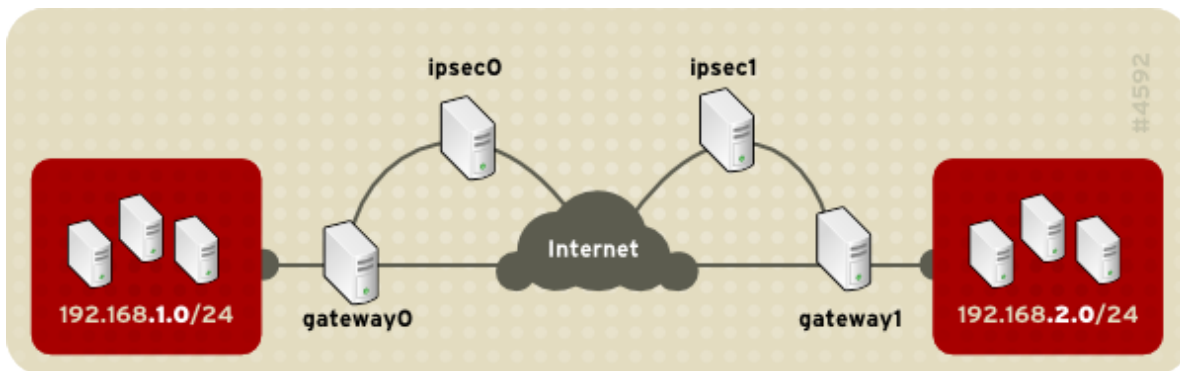
Figure 45.11. A network-to-network IPsec tunneled connection
