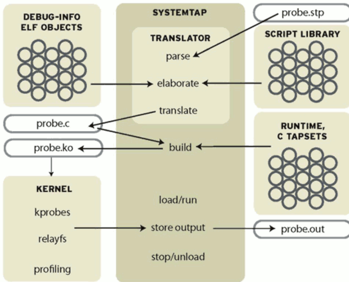
Figure 38.1. Flow of Data in SystemTap
