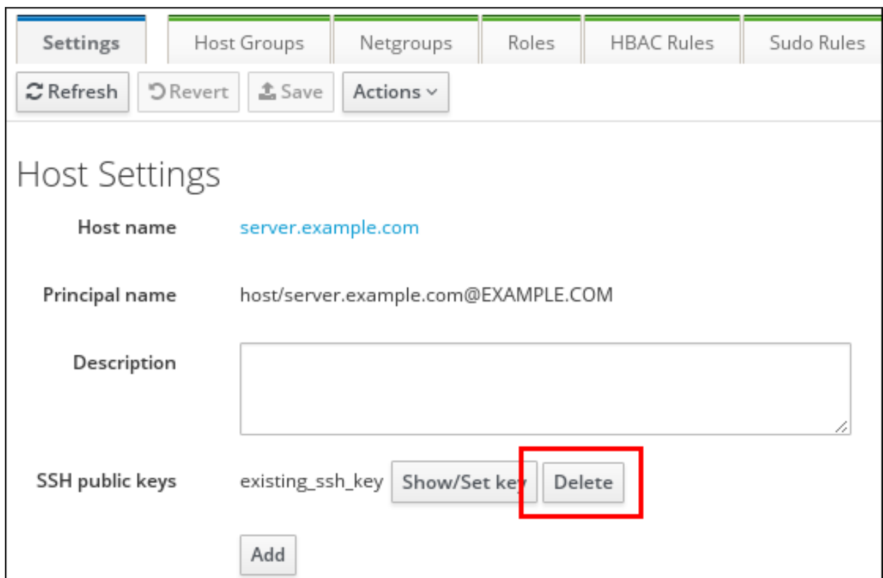
Figure 13.12. Public Key Deletion
