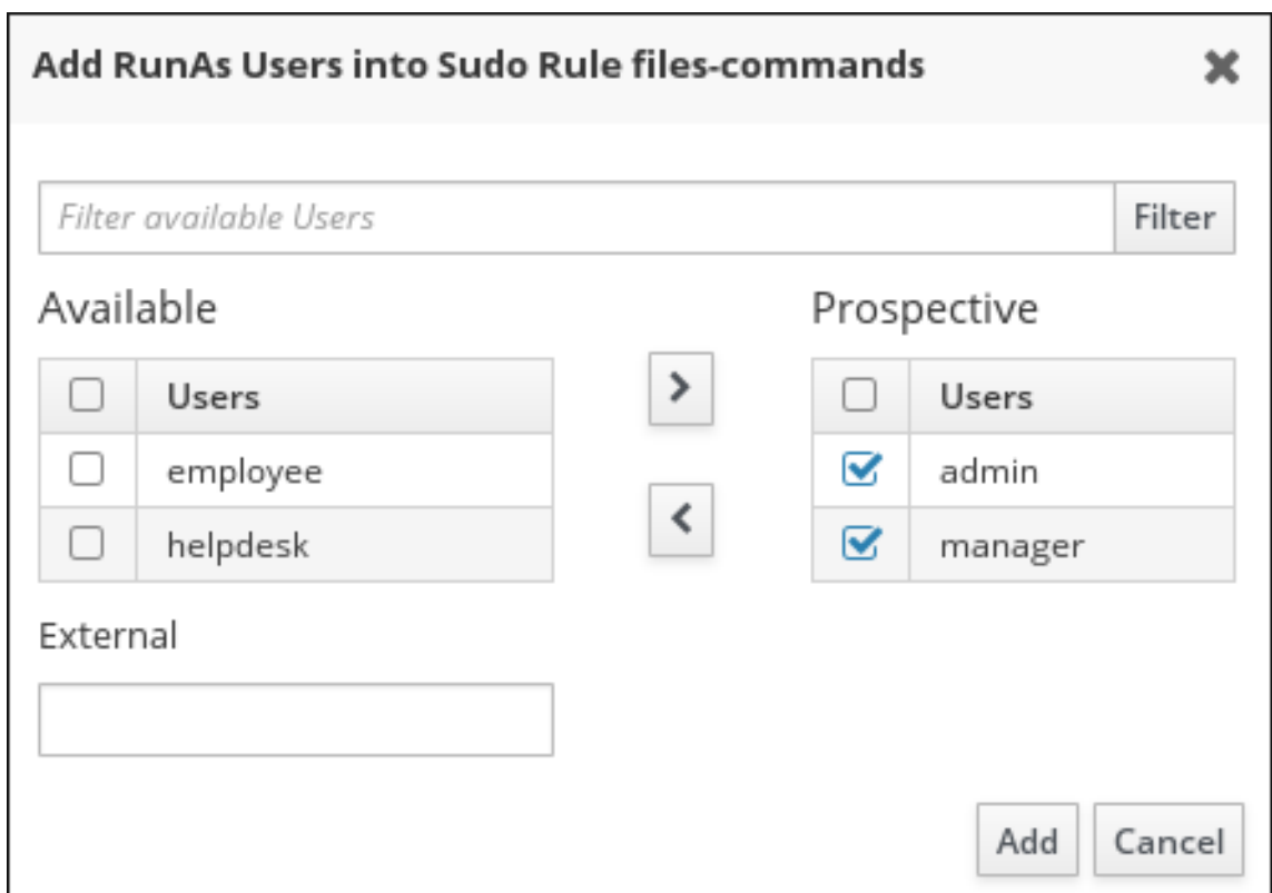
Figure 21.13. Selecting Users for the Command
