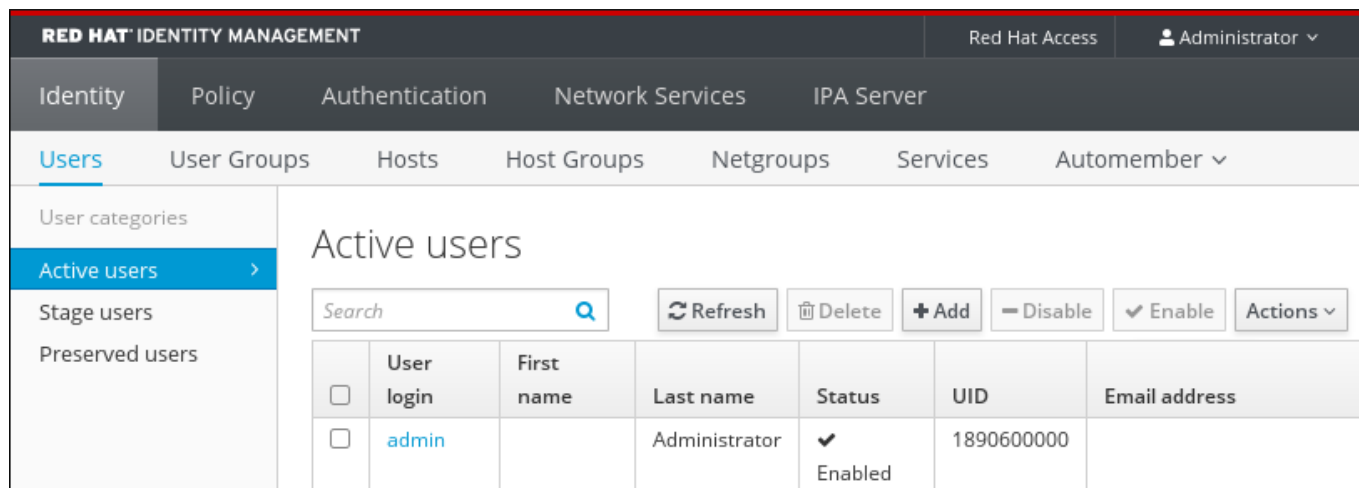
Figure 7.2. The IdM Web UI Layout
