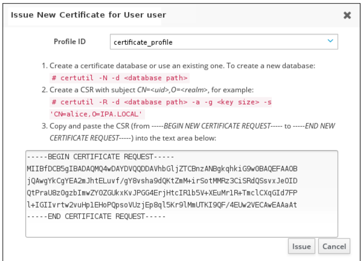
Figure 9.48. Issuing a Certificate for a User
