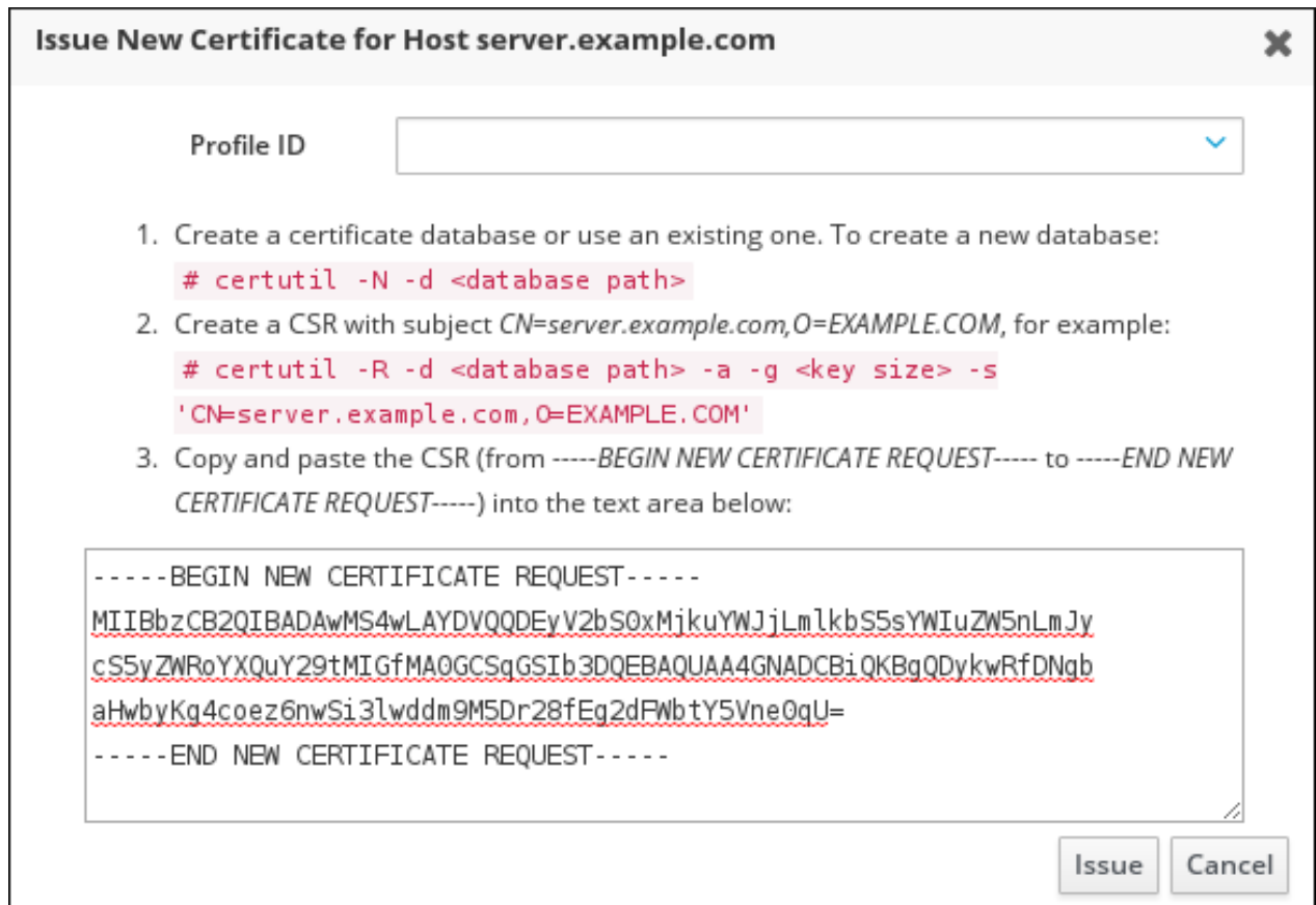
Figure 13.7. Issuing a Certificate
