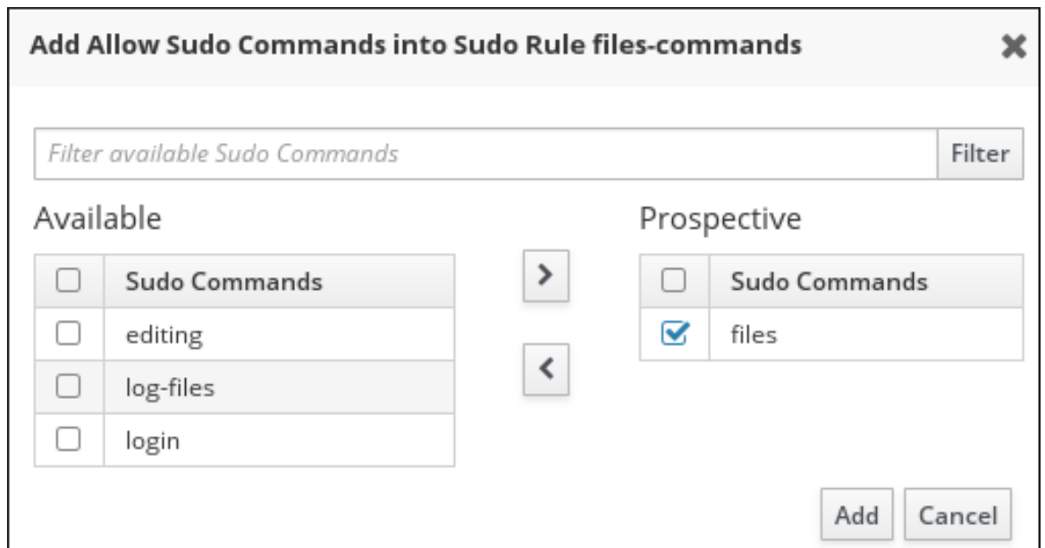
Figure 21.11. Selecting Commands for a sudo Rule
