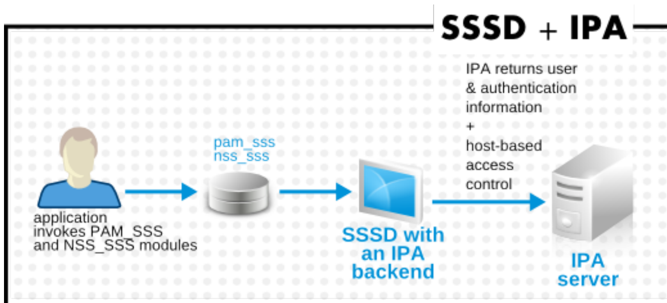
Figure 32.2. Clients and SSSD with an IdM Backend
