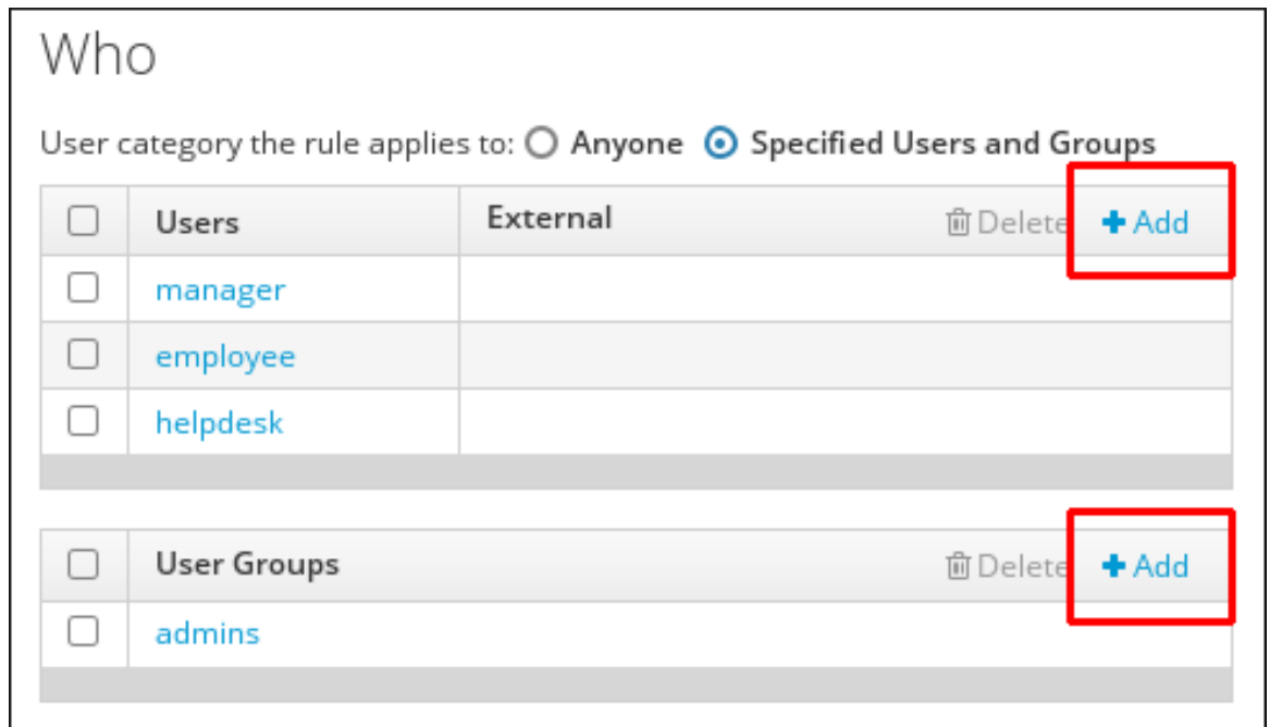
Figure 21.6. Adding Users to a sudo Rule
