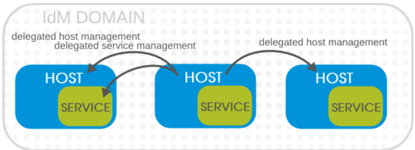
Figure 15.1. Host and Service Delegation
