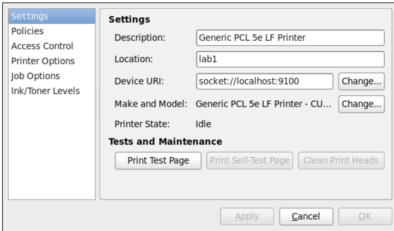
Figure 16.10. Settings page
