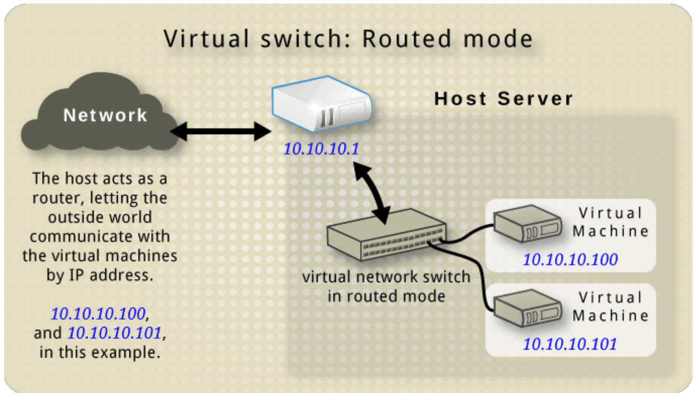
Figure 20.5. Virtual network switch in routed mode
