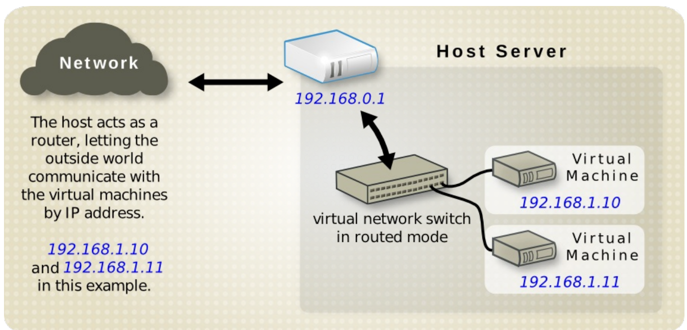
Figure 20.10. Virtual server using static IP addresses
