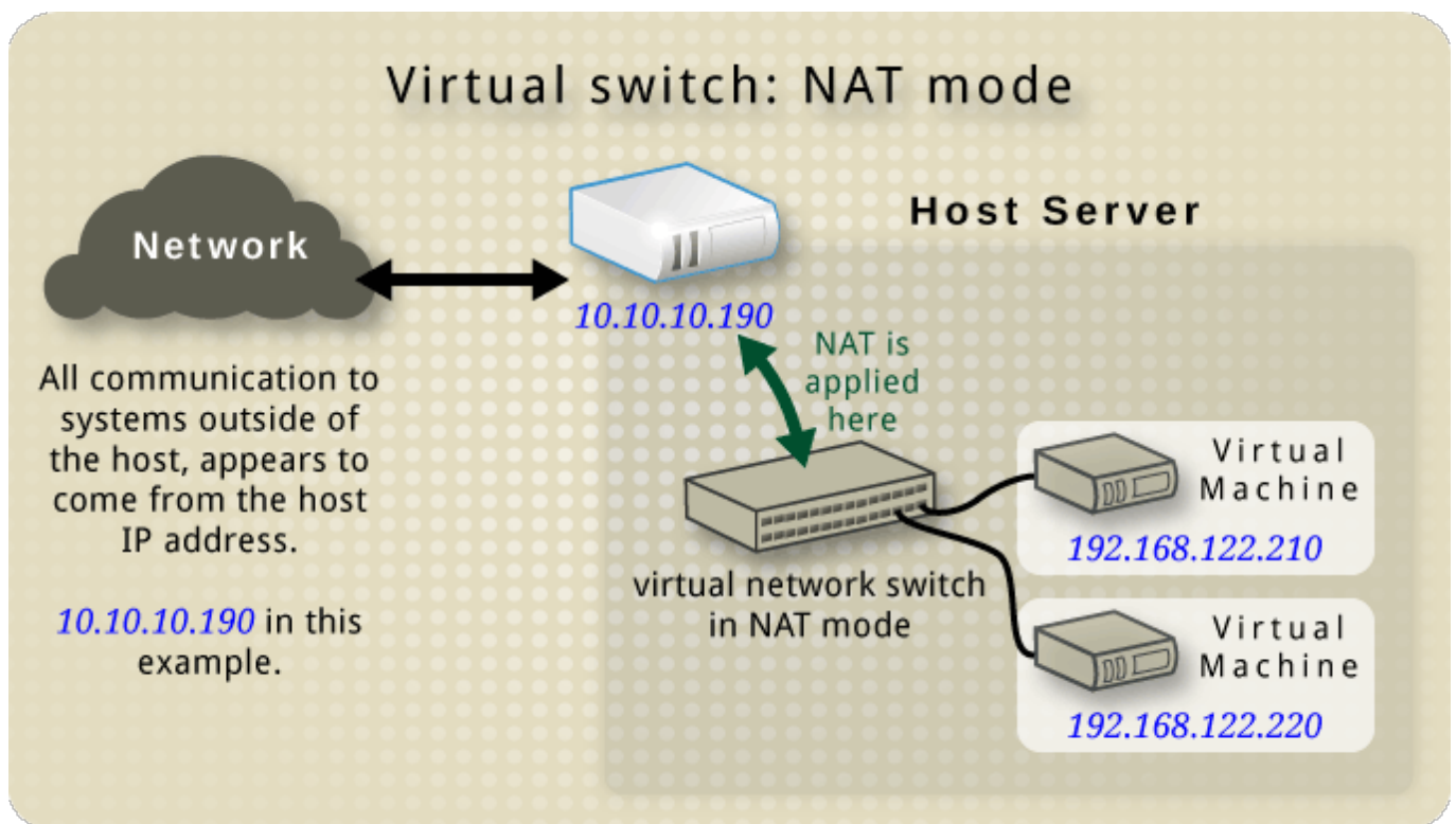
Figure 20.3. Virtual network switch using NAT with two guests
