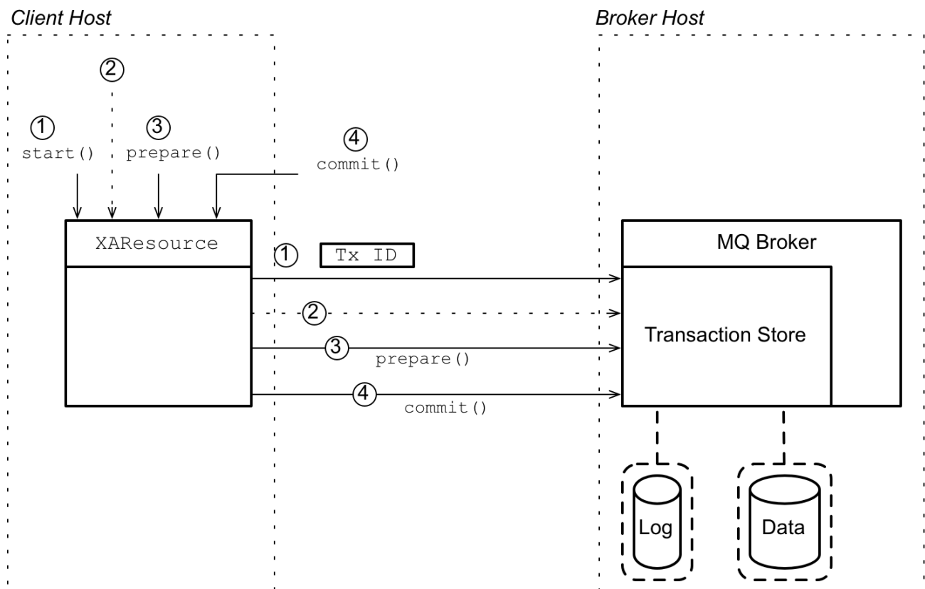
Figure 7.2. JMS XA Resource Connected to Remote Broker
