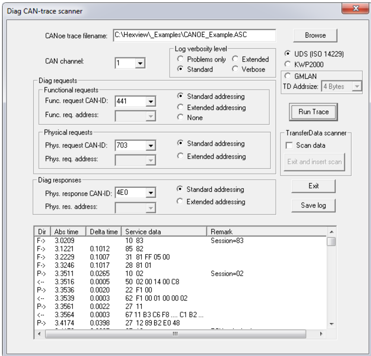
Figure 2-31: Dialog to run a CANoe trace
