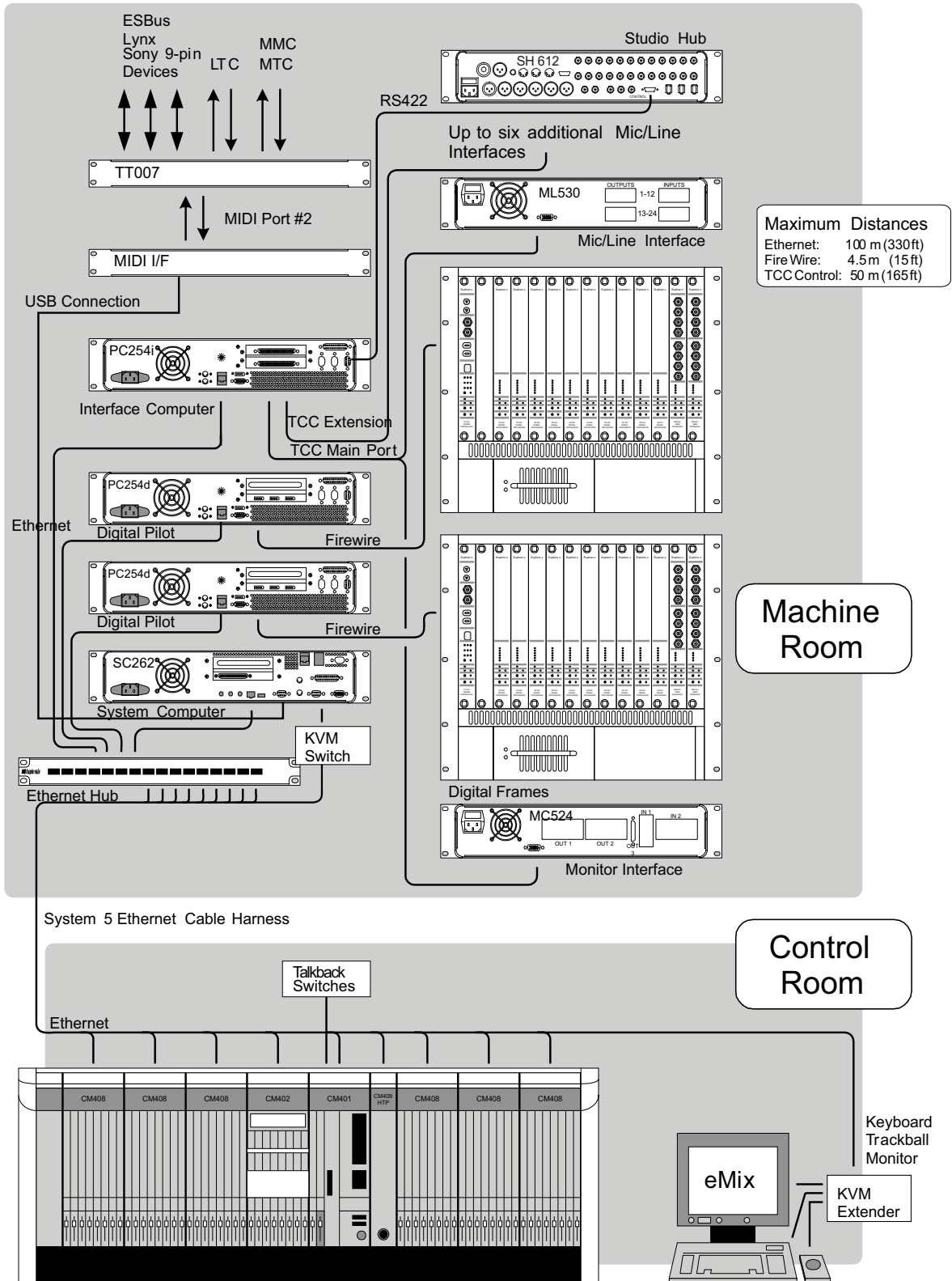
Figure 2-15 Control Hookup
