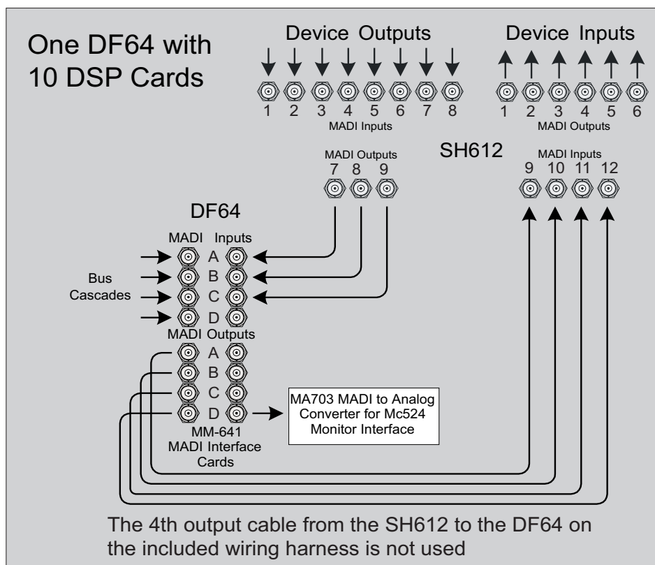
Figure 2-11 MADI hookup: one DF64 core, 10 or 11 DSP cards, one SH612
