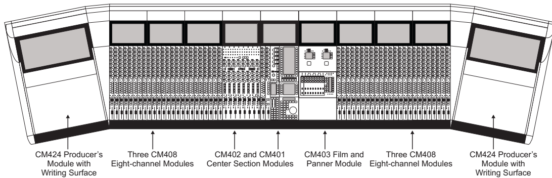
Figure 2-2 System 5 Console
