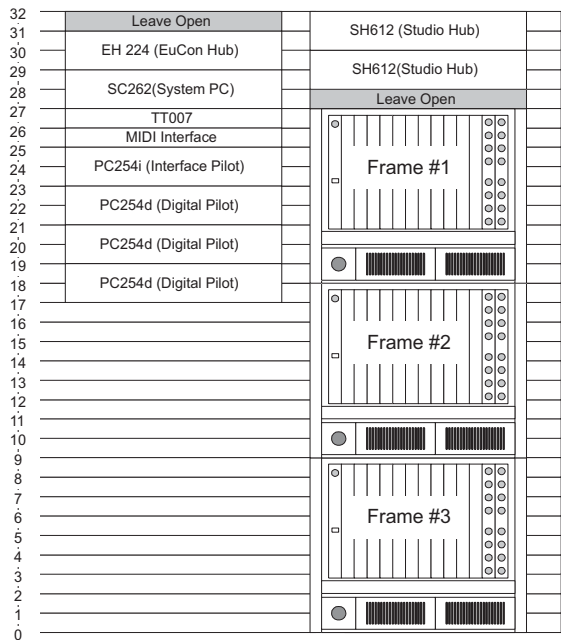
Figure 2-7 Three-frame System
