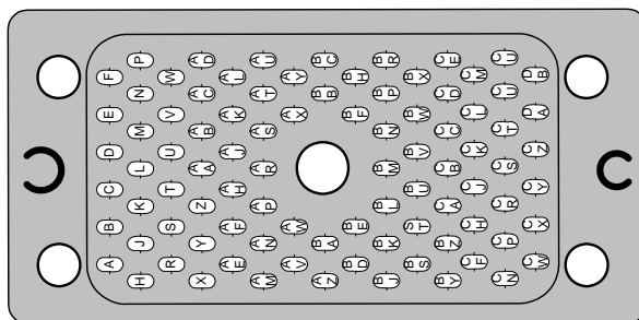
Figure 3-12 Elco 90 Connector
