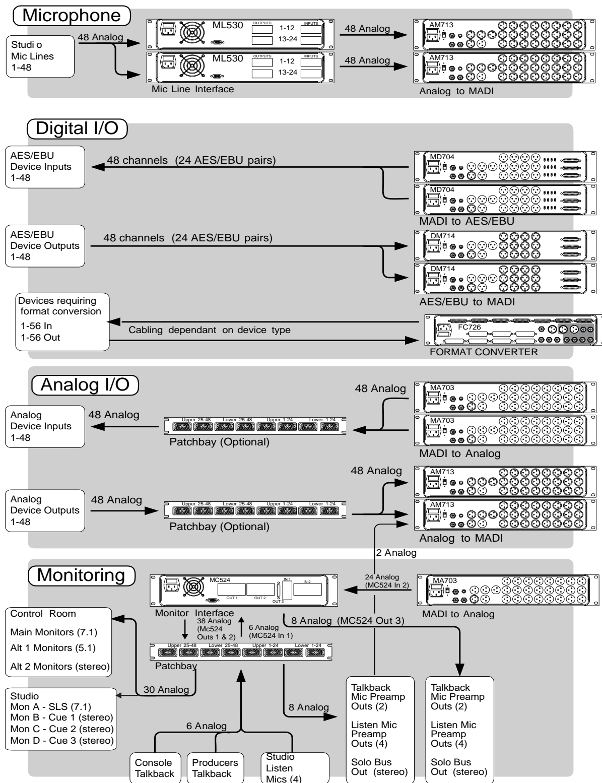
Figure 2-9 Audio Hookup
