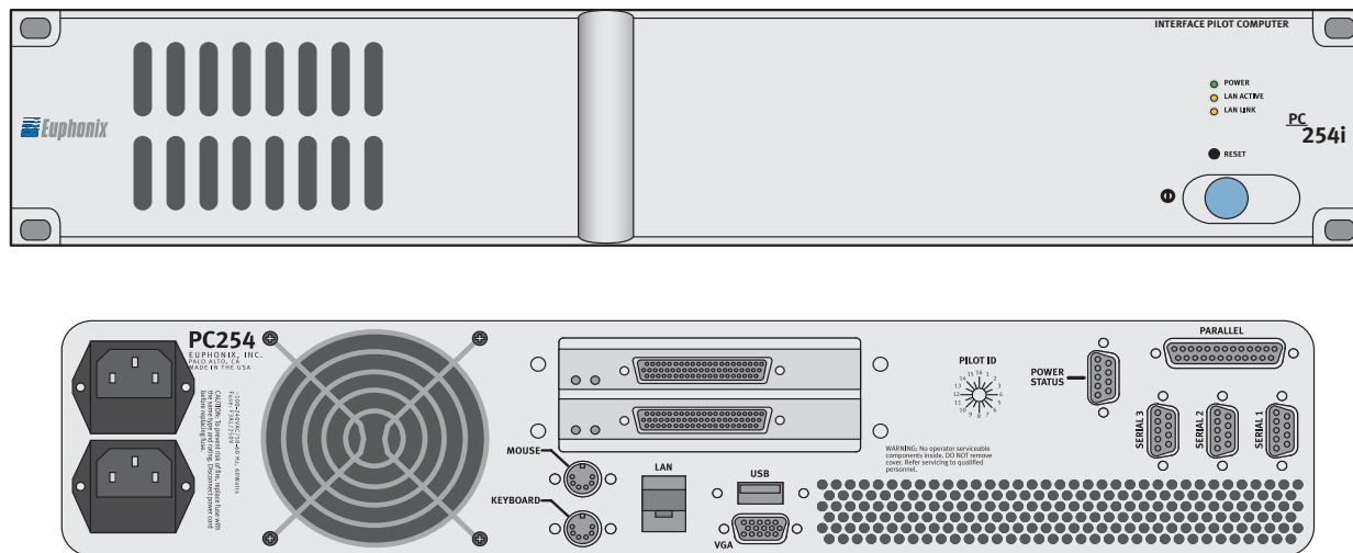
Figure 3-7 PC254i Front and Rear Panels
