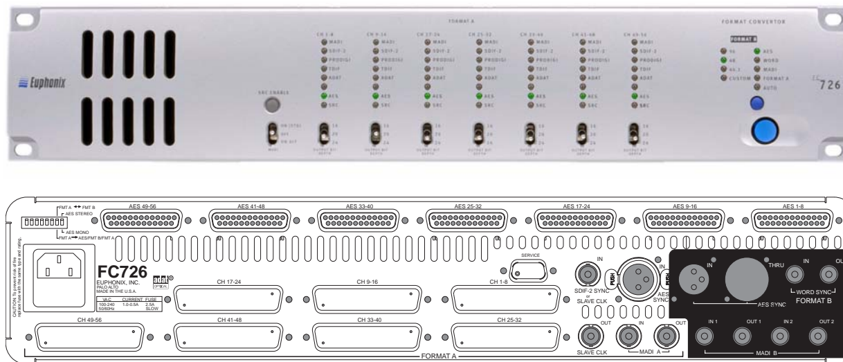
Figure 3-28 FC726 Front and Rear Panels
