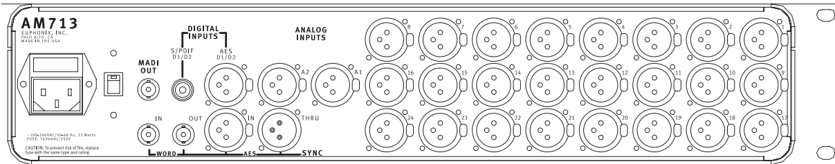
Figure 3-19 AM713 Rear Panel
