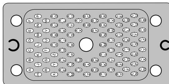
Figure 3-10 Elco 90 Connector
