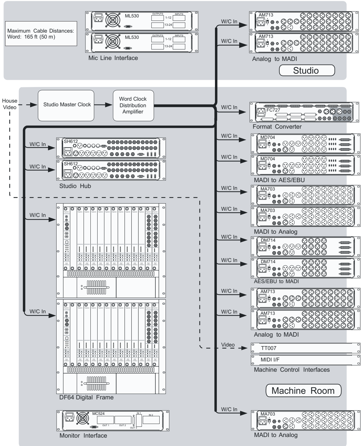
Figure 2-10 Synchronization Hookup (Word Clock shown, AES/EBU may be used)
