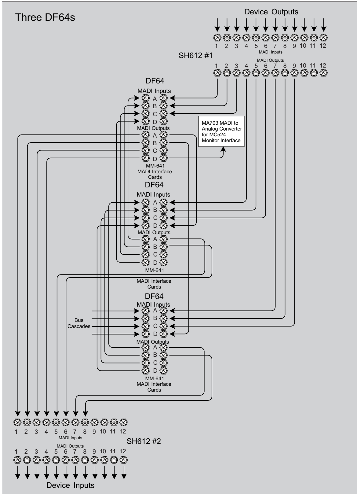
Figure 2-13 MADI hookup for three DF64 cores and two SH612 Studio Hubs
