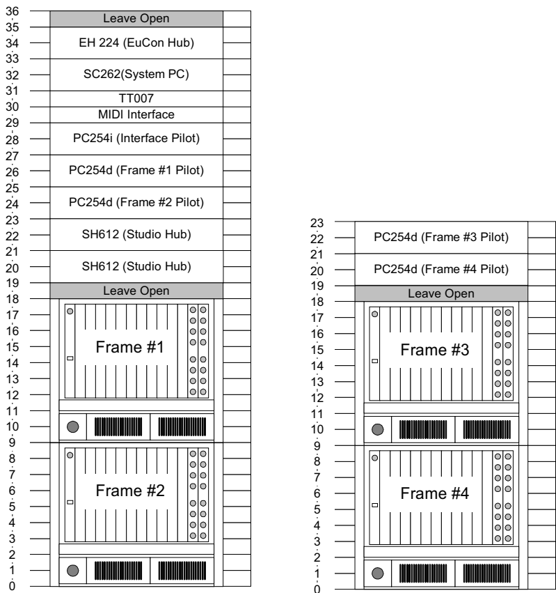
Figure 2-8 Four-frame System
