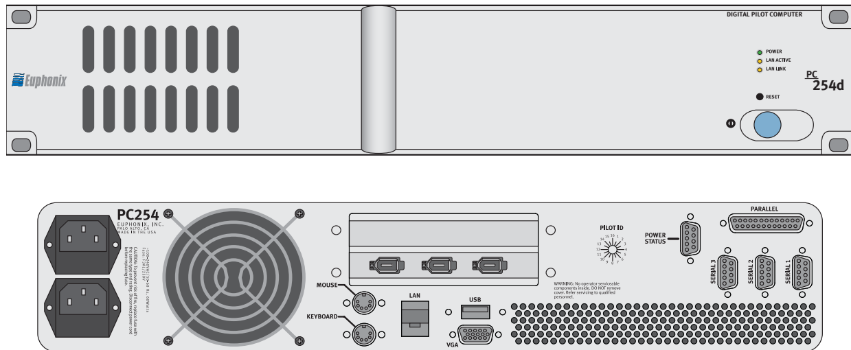
Figure 3-6 PC254d Front and Rear Panels
