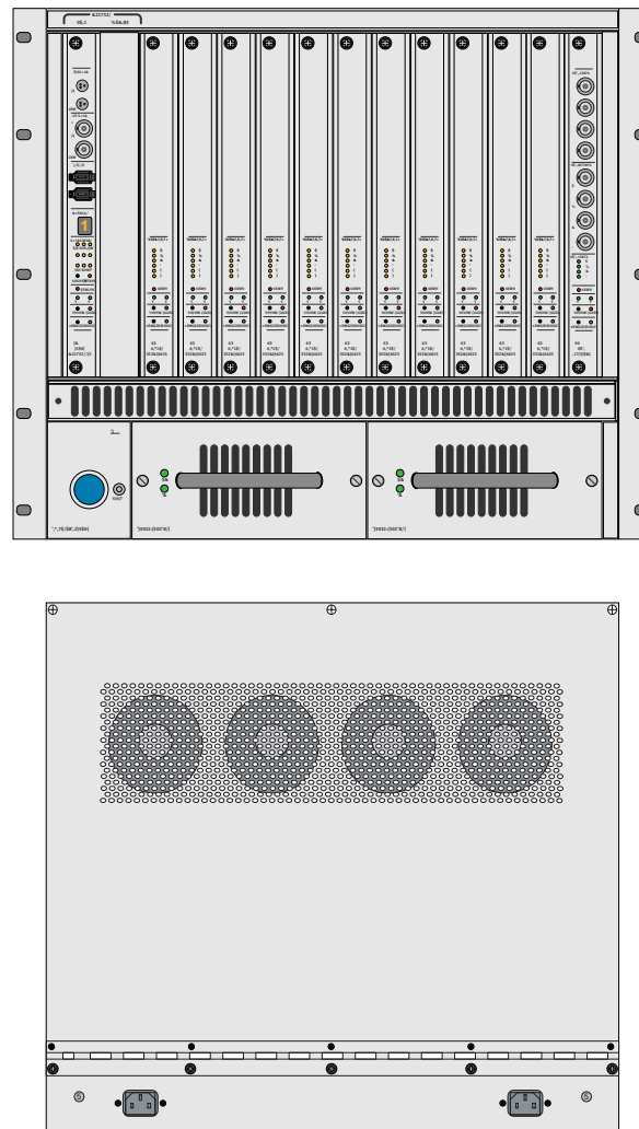
Figure 3-1 DF64 Digital Frame Front and Rear Panels
