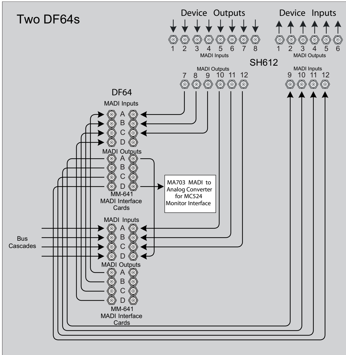
Figure 2-12 MADI hookup for two DF64 cores and one SH612 Studio Hub
