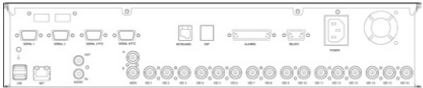
16 Input model
