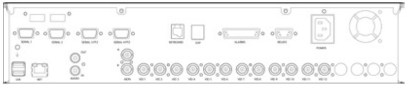
12 Input model
