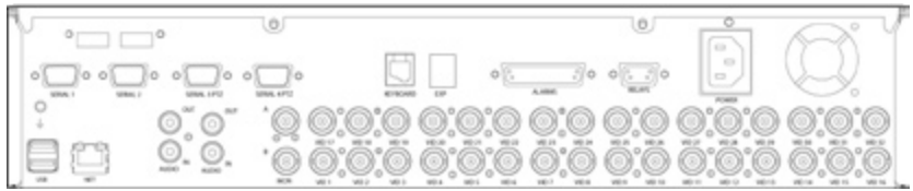
32 Input model
