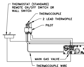
THERMOSTAT WIRING DIAGRAM 85-03-514
