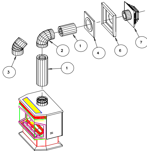
HORIZONTAL TERMINATION
