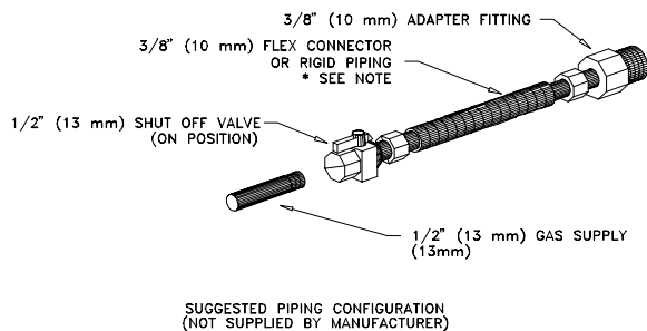
FIGURE 6: Piping Detail
