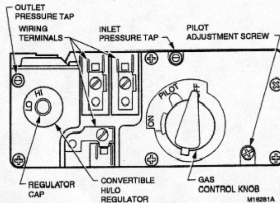
Fig. 1. Top view of a convertible High/Low combination gas control (VS8520E shown here).
