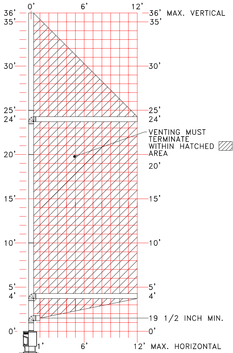
Figure 5: Minimum-Maximum Vent Requirements
