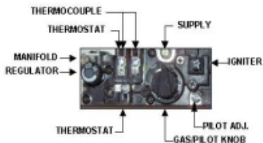
FIGURE 8: Gas Valve
