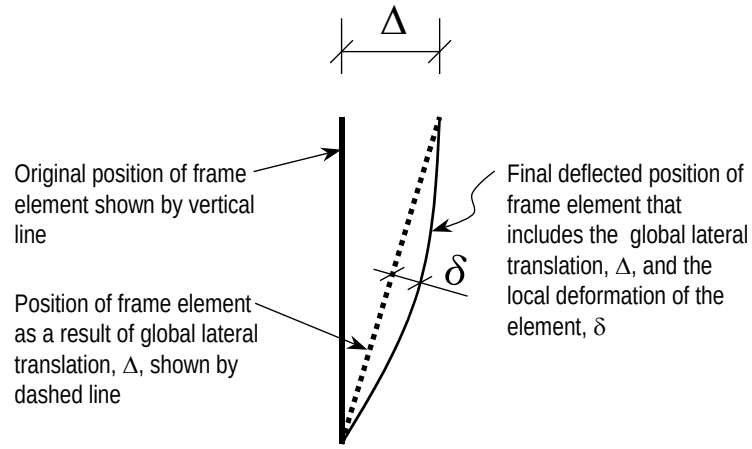
Figure 2-1 P- \Delta and P- \delta effects
