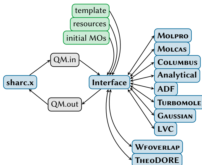
Figure 6.1: Communication between sharc.x , the interfaces, and the quantum chemistry codes.
