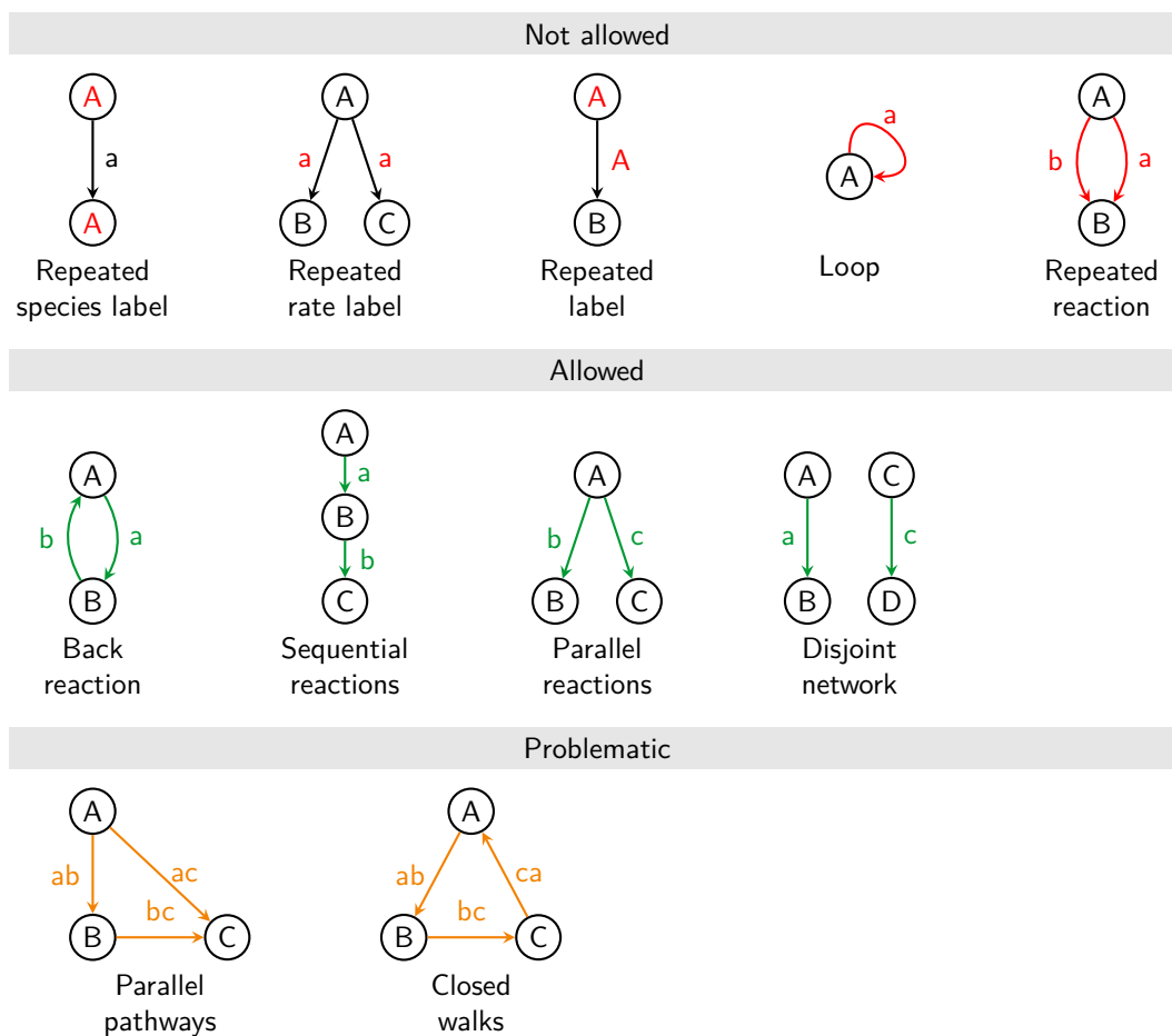
Figure 8.1: Forbidden and allowed features of the reaction network graphs.
