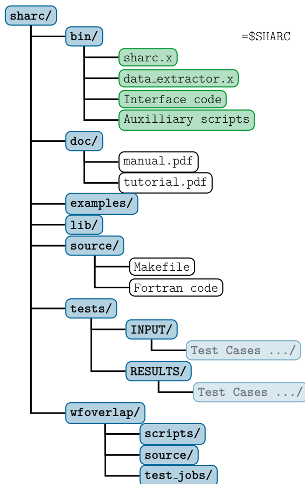
Figure 2.1: Directory tree containing a complete SHARC installation.
