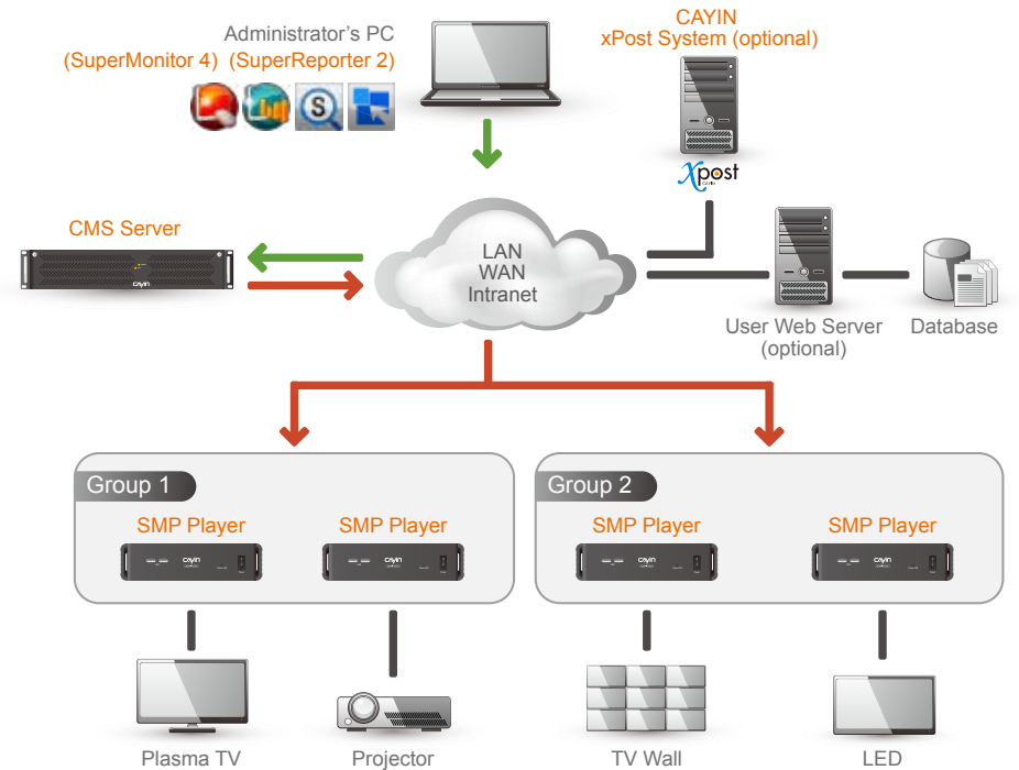
Digital Signage Network with Client-Server Structure (CMS server + SMP player)
