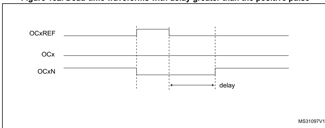
Figure 182. Dead-time waveforms with delay greater than the positive pulse
