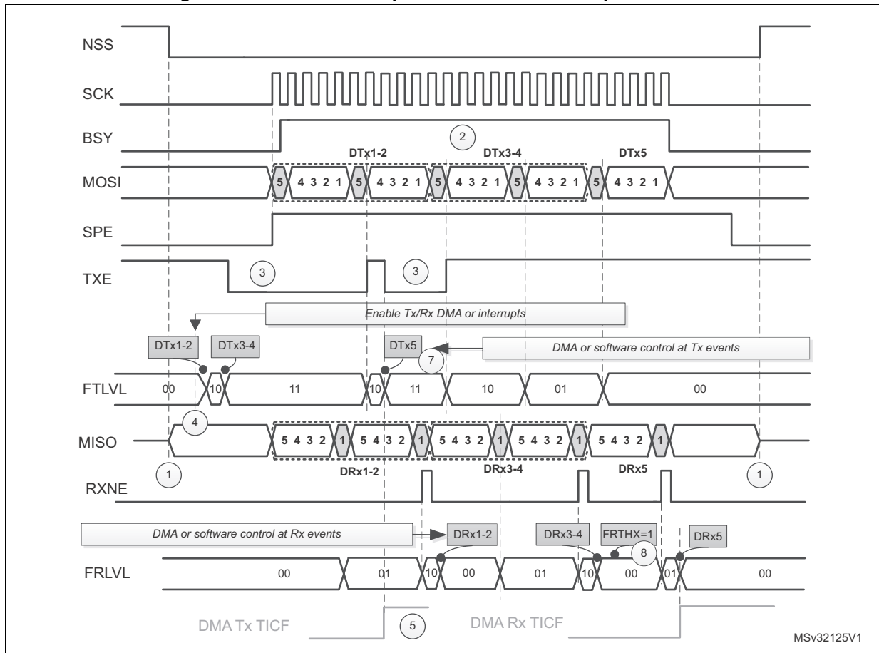
Figure 257. Master full duplex communication in packed mode
