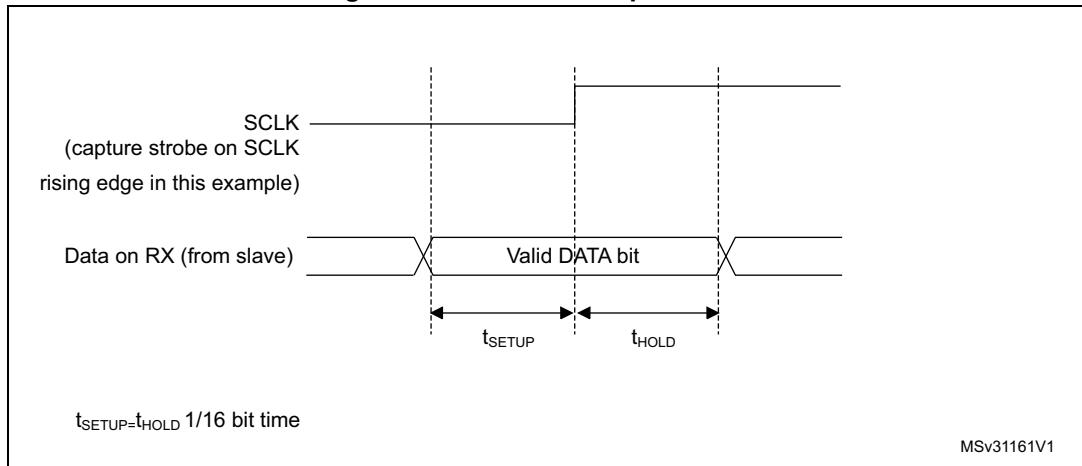
Figure 238. RX data setup/hold time
