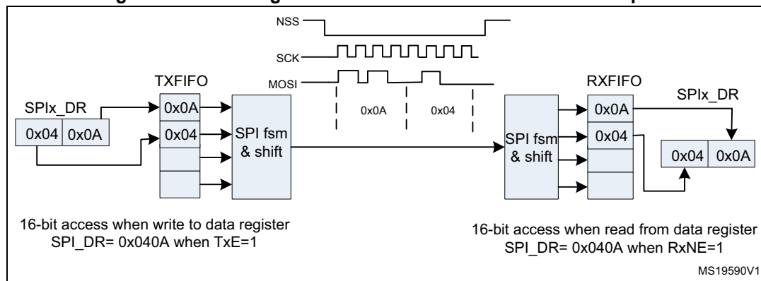
Figure 253. Packing data in FIFO for transmission and reception
