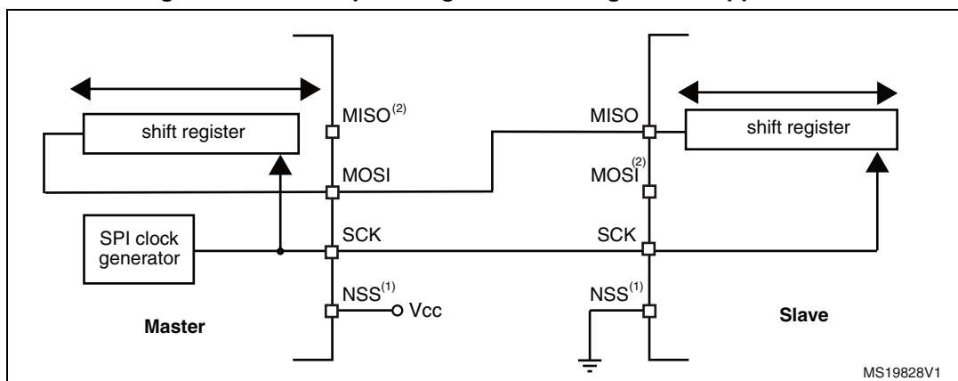
Figure 247. Half-duplex single master/ single slave application
