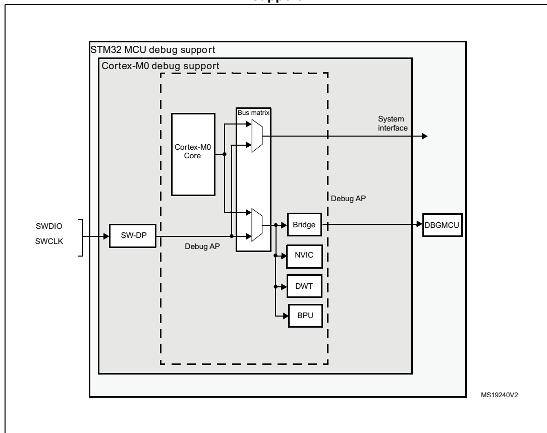
Figure 262. Block diagram of STM32F0x0 MCU and ARM® Cortex®-M0-level debug support
