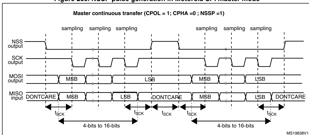
Figure 258. NSSP pulse generation in Motorola SPI master mode
