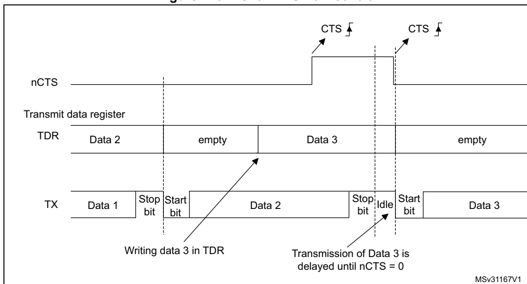
Figure 243. RS232 CTS flow control
