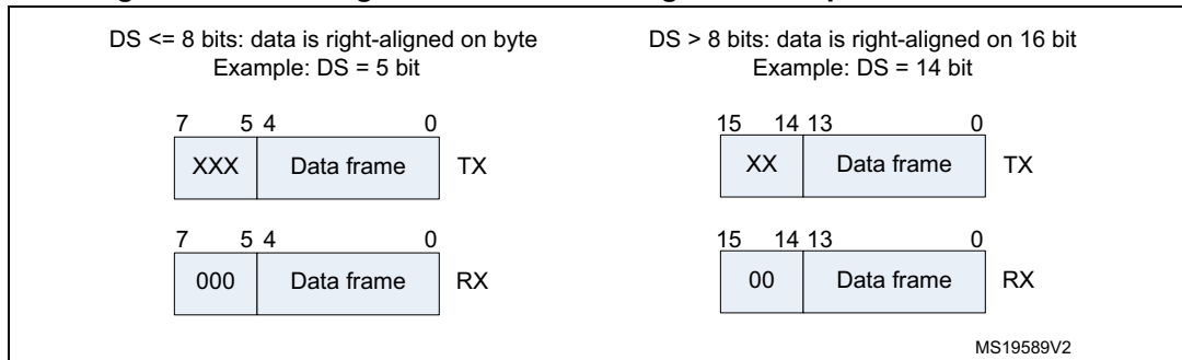
Figure 252. Data alignment when data length is not equal to 8-bit or 16-bit
