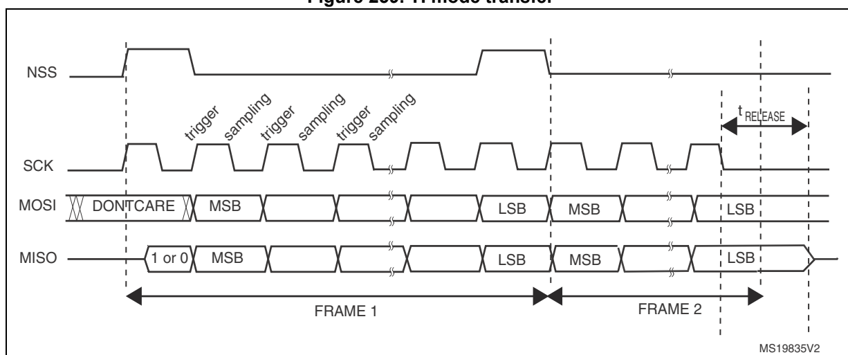
Figure 259. TI mode transfer
