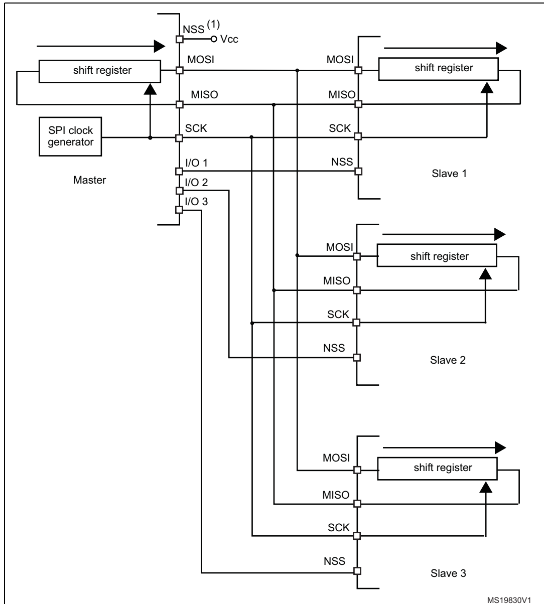
Figure 249. Master and three independent slaves
