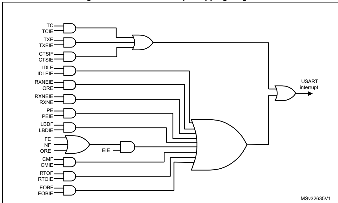
Figure 244. USART interrupt mapping diagram
