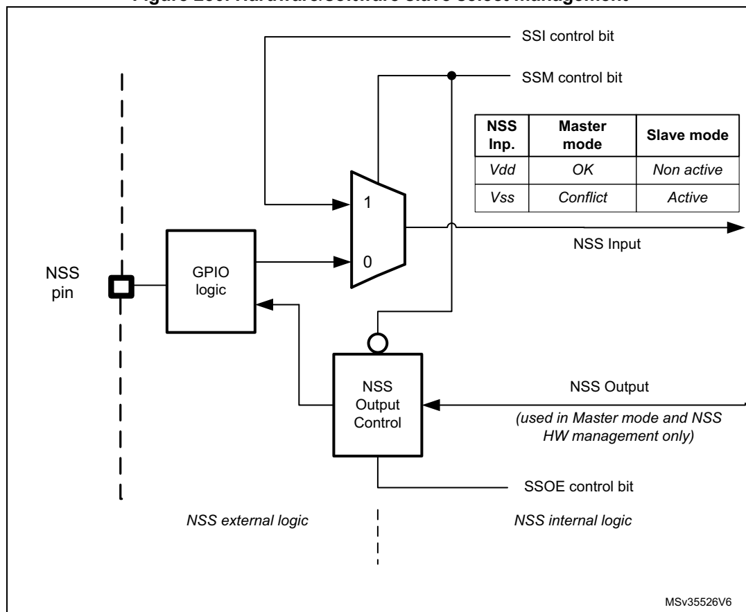
Figure 250. Hardware/software slave select management
