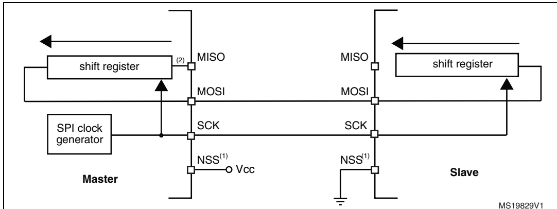
Figure 248. Simplex single master/single slave application (master in transmit-only/ slave in receive-only mode)
