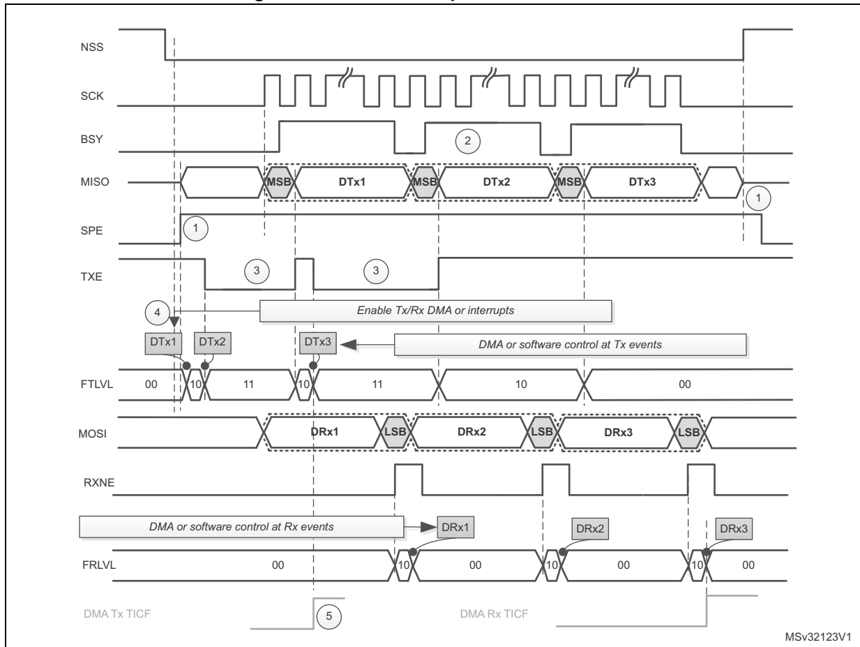
Figure 255. Slave full duplex communication
