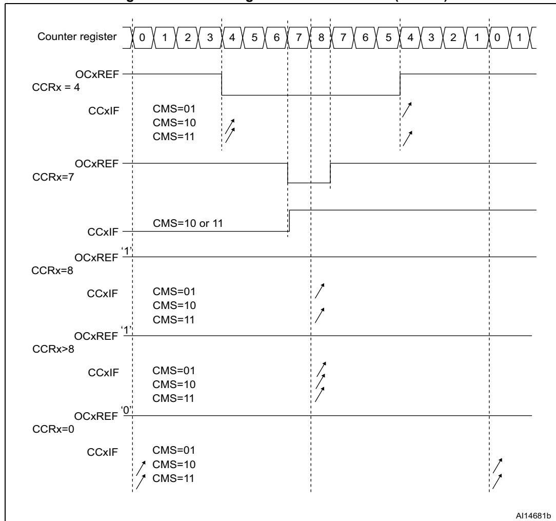
Figure 73. Center-aligned PWM waveforms (ARR=8)
