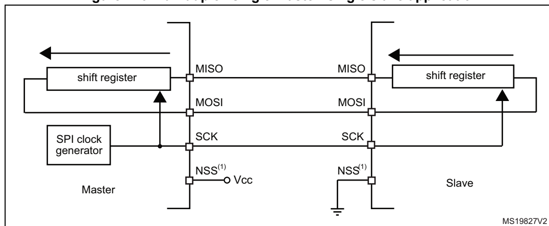
Figure 246. Full-duplex single master/ single slave application
