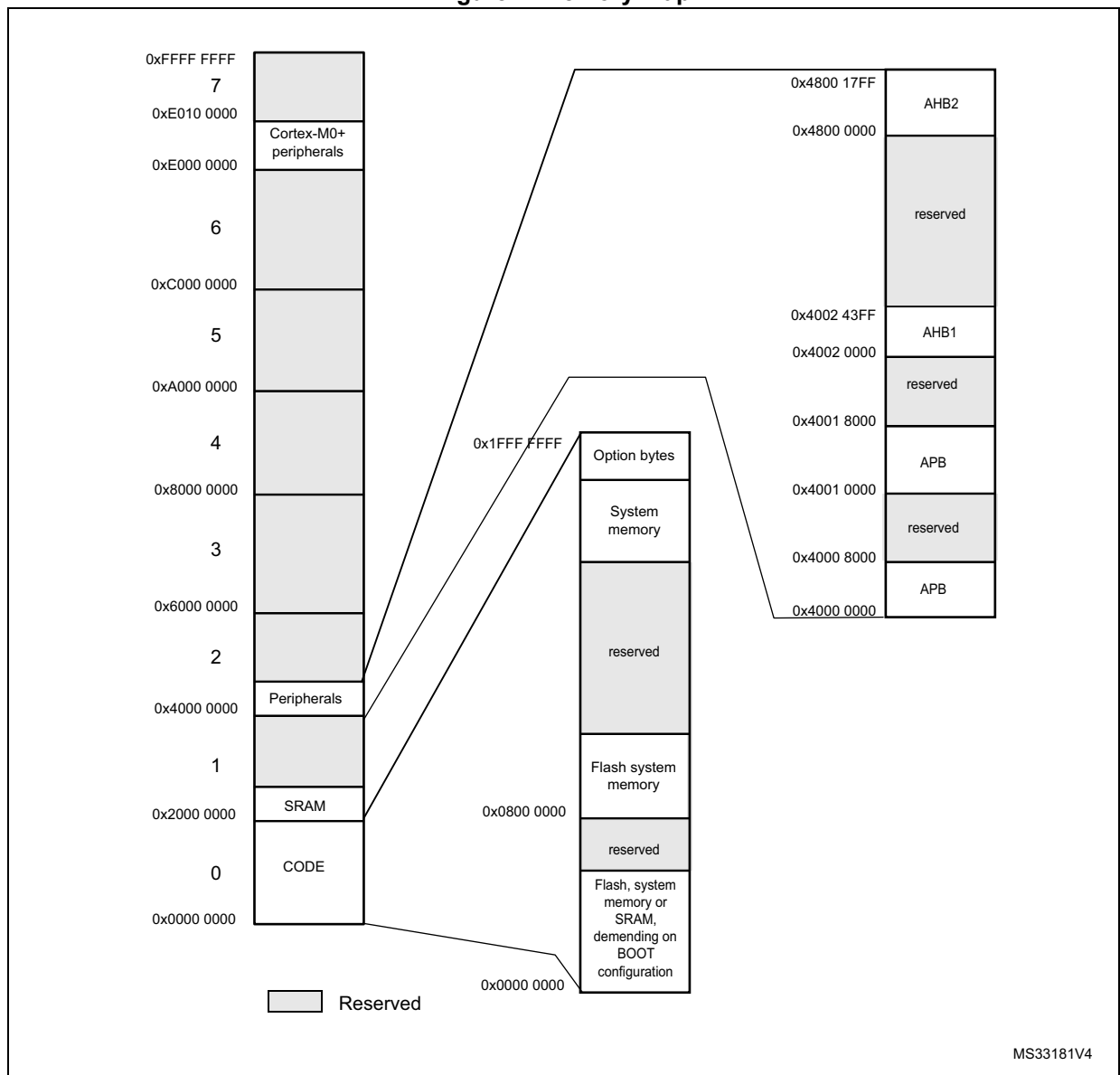
Figure 2. Memory map
