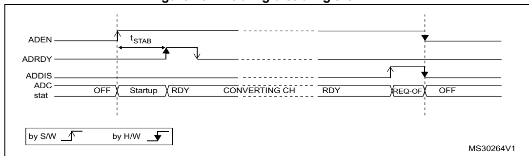
Figure 25. Enabling/disabling the ADC
