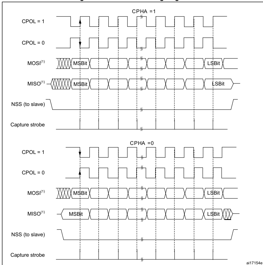
Figure 251. Data clock timing diagram
