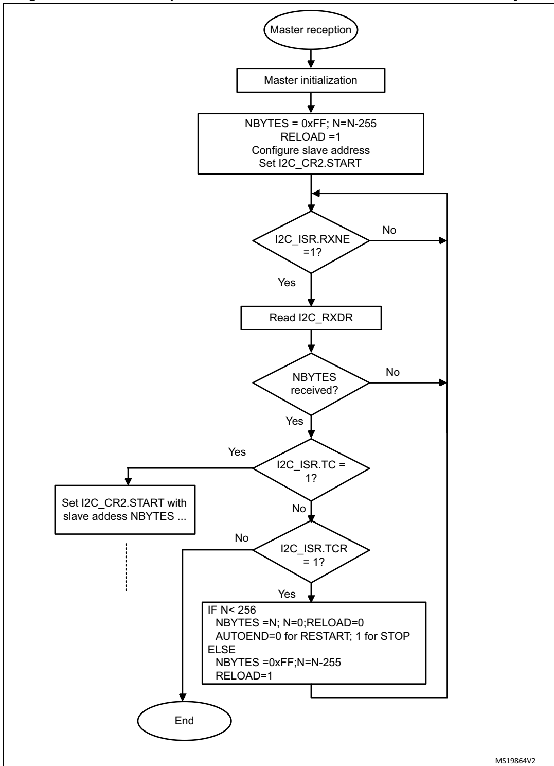
Figure 216. Transfer sequence flowchart for I2C master receiver for N >255 bytes
