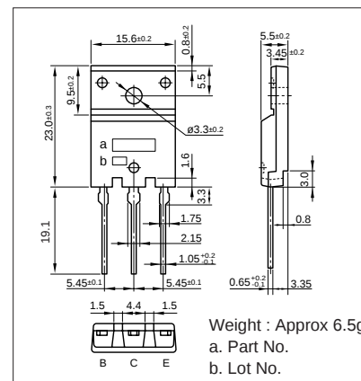
External Dimensions FM100(TO3PF)
