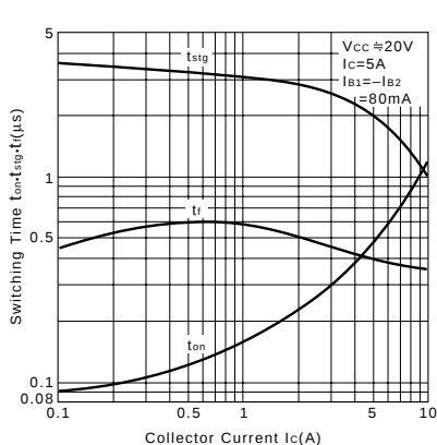
ton•tstg•tr-I c Characteristics (Typical)
