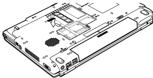
Figure 8-8 Inserting the memory module
