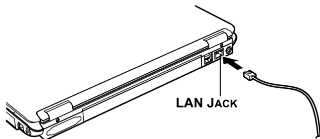
Figure 4-14 Connecting the LAN cable
