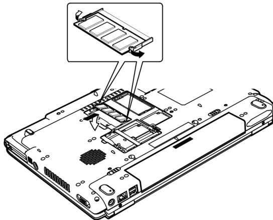
Figure 8-9 Removing the memory module
