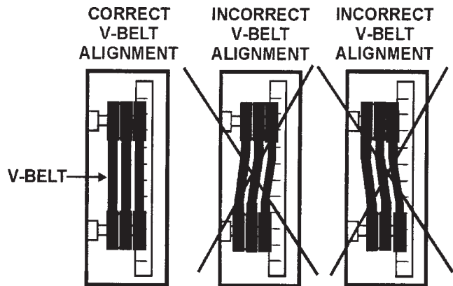
Figure 10. Pulley Alignment
