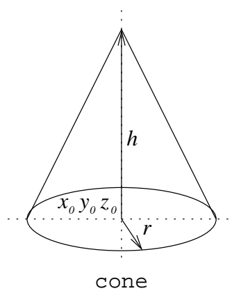
Figure 3.2: The cone surface.
