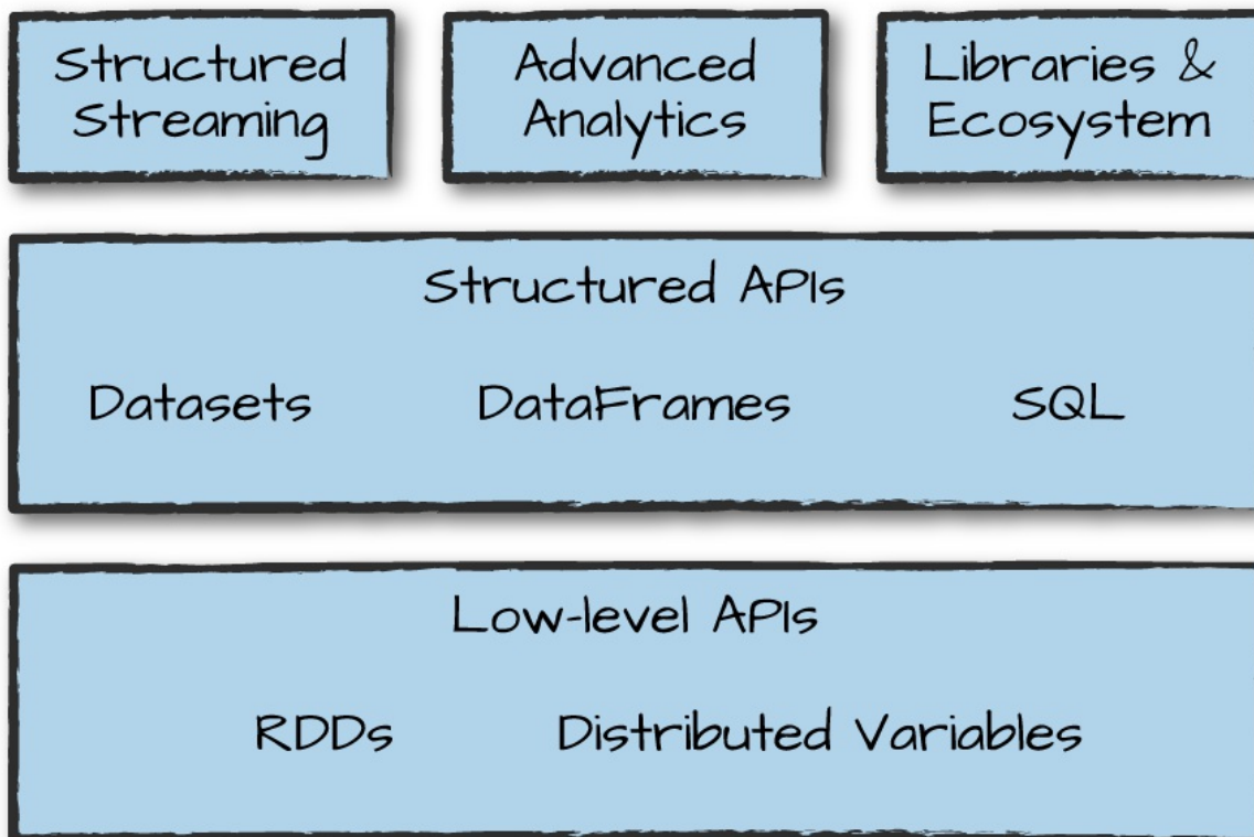
Figure 1-1. Spark's toolkit
