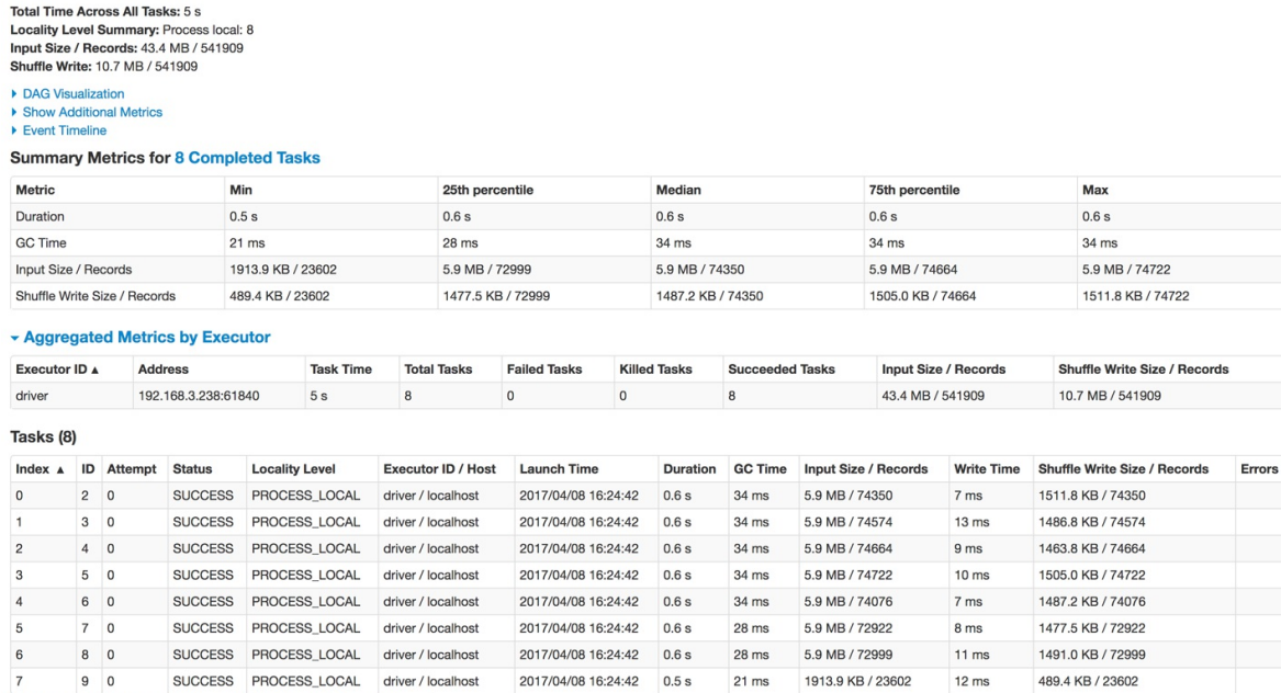
Figure 18-8. Spark tasks
