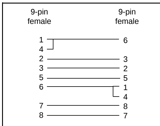
Figure 2-3 RS-232 DB9 to DB9 Cabling
