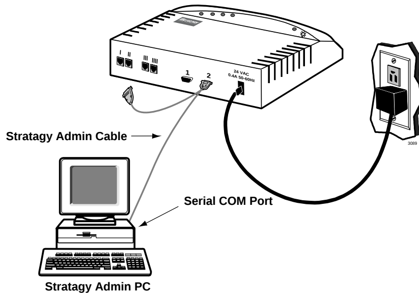
Figure 2-2 Strategy Flash/Strategy Admin PC Local Connection
