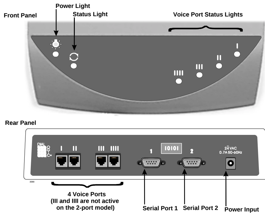
Figure 1-1 Flash Front and Back Panels
