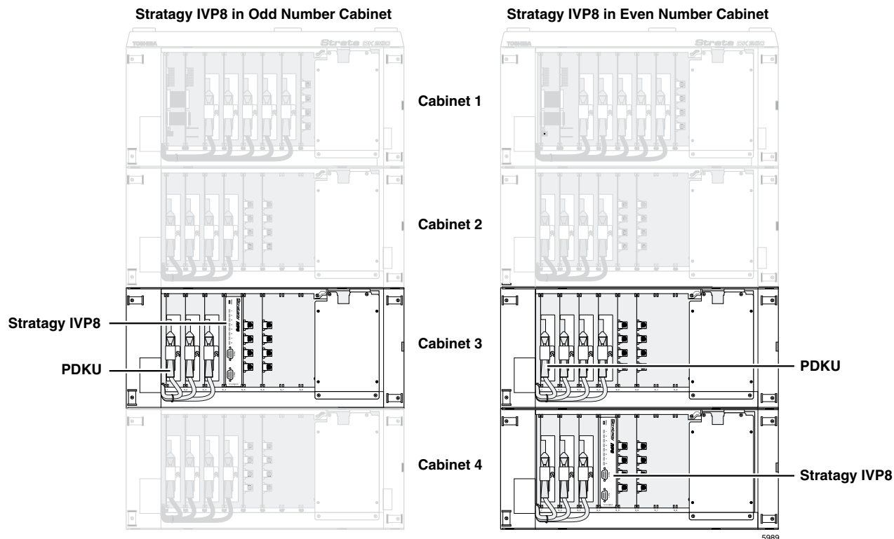
Figure 2-1 Strata DK424i/DK424/DK280 PDKU DSS/Busy Lamp Field Slot Assignment Examples (console_slot_id configured as 0)
