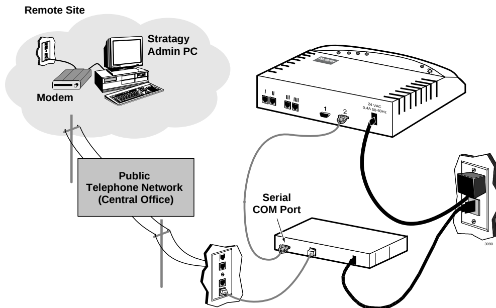
Figure 2-5 Flash/Strategy Admin PC Remote Connection
