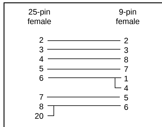
Figure 2-4 RS-232 DB25 to DB9 Cabling
