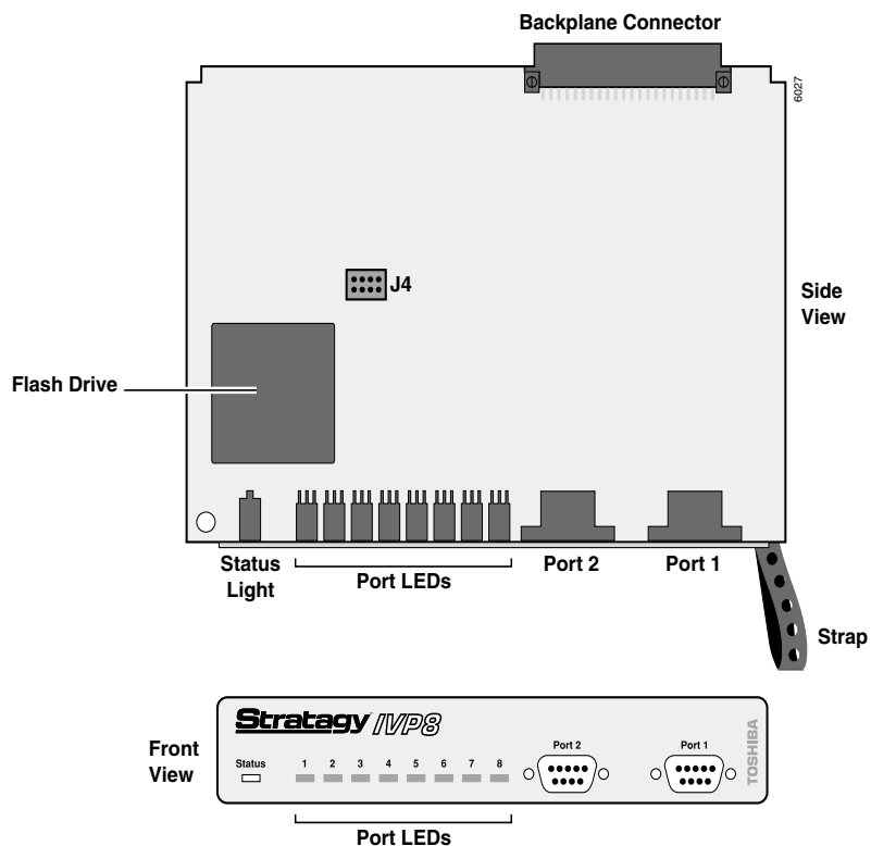
Figure 1-2 IVP8 Hardware Components
