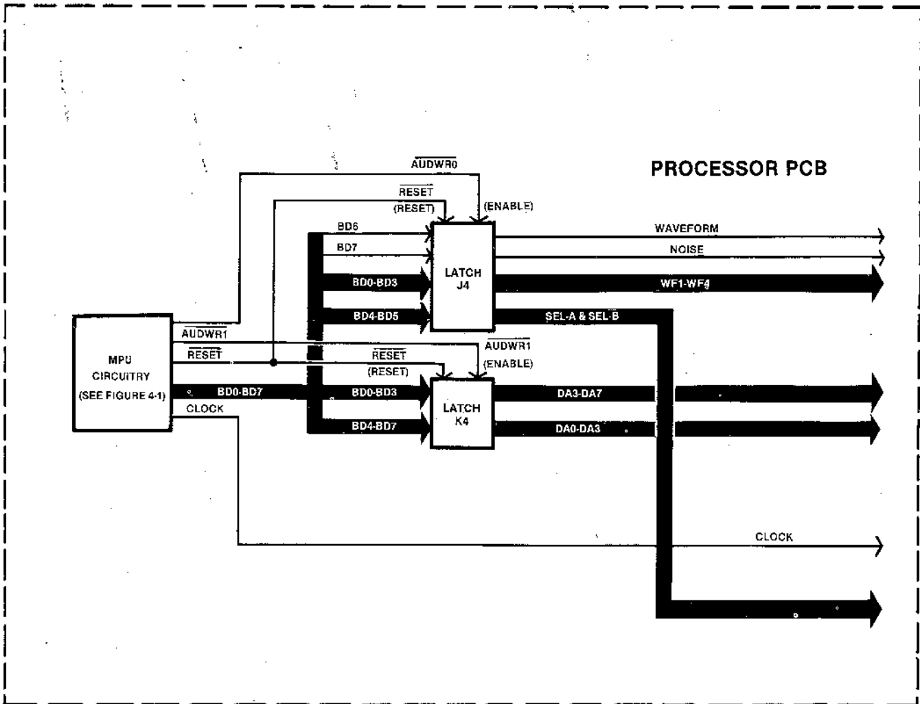
Figure 4-6 Audio Circuitry
