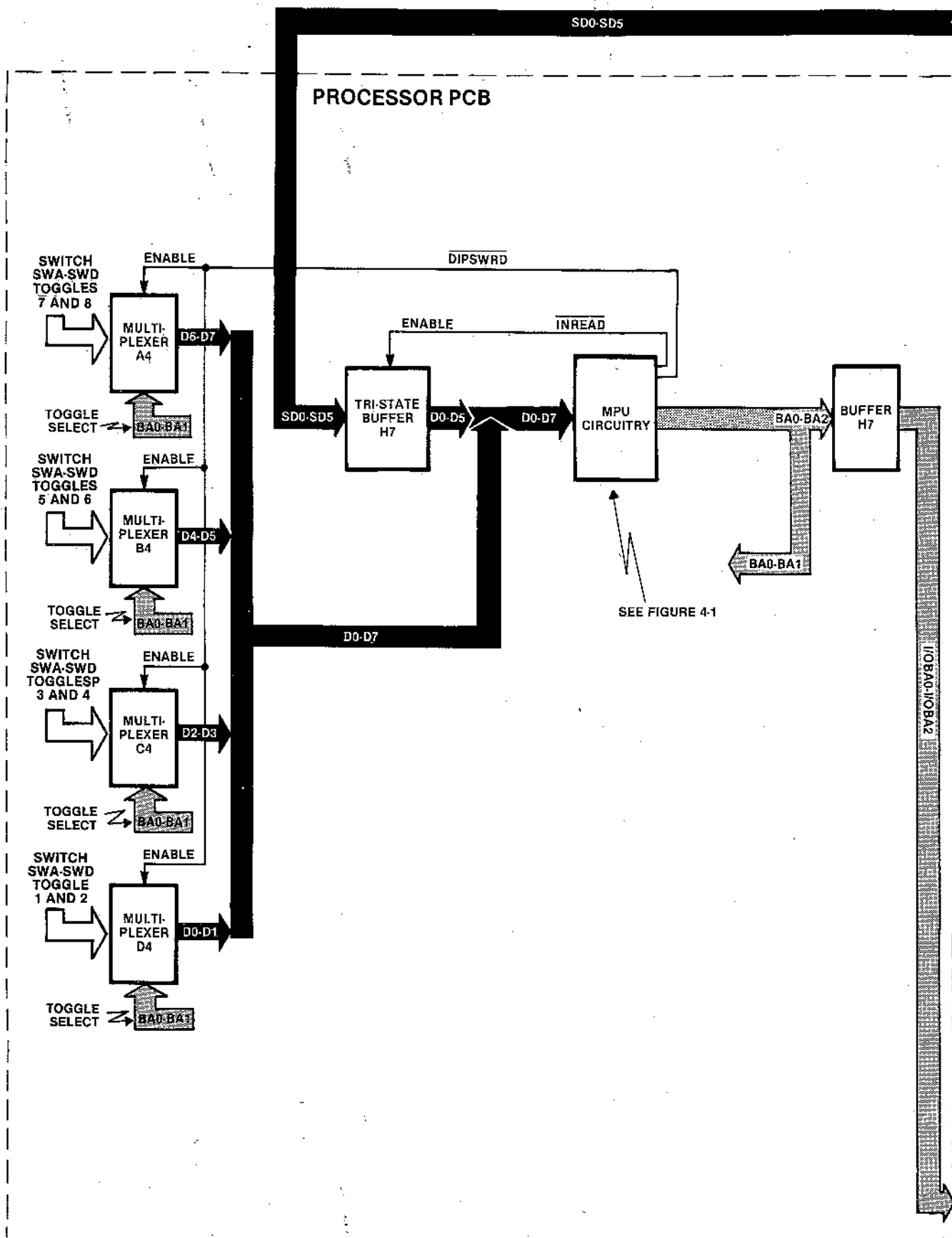
Figure 4-2 Switches Circuitry
