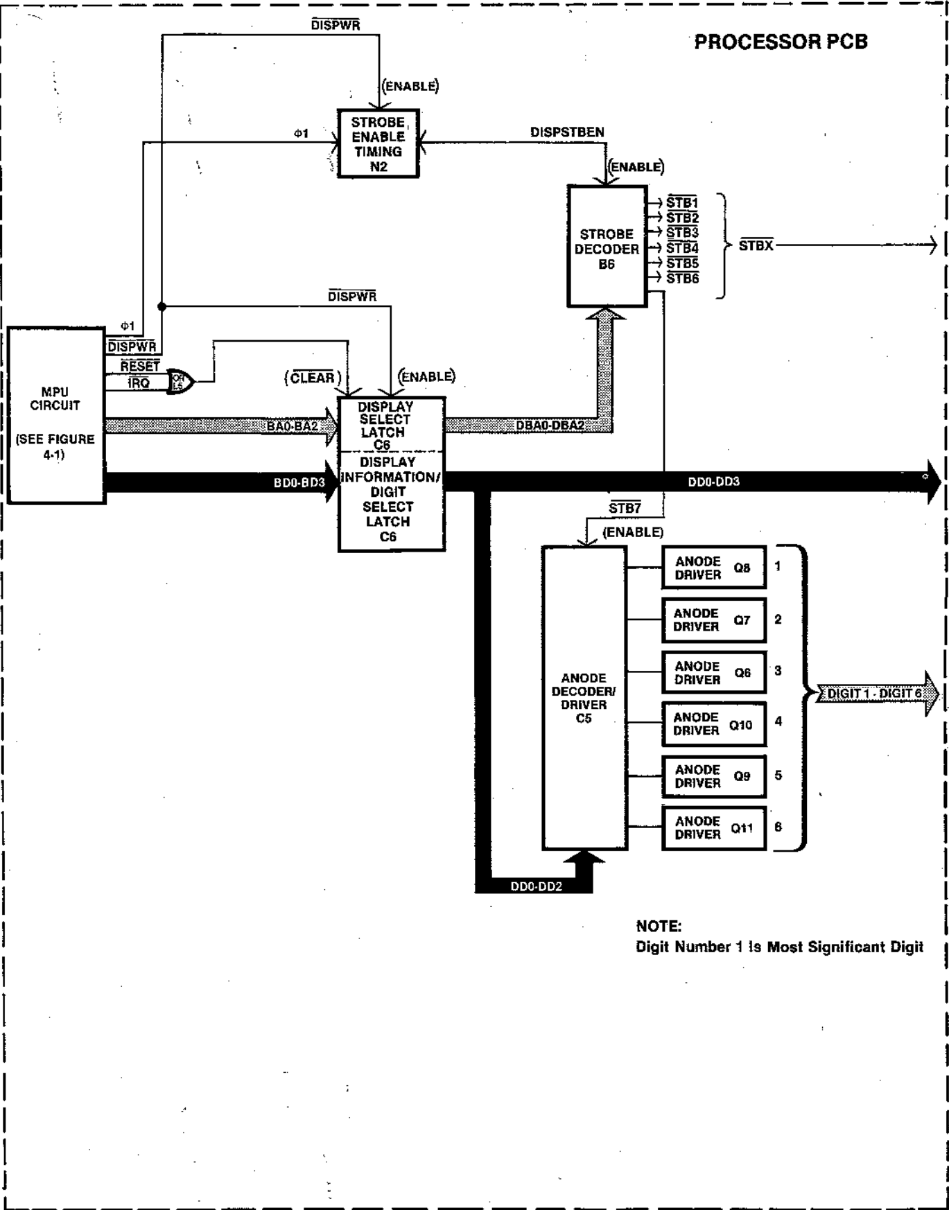
Figure 4-5 Display Circuitry
