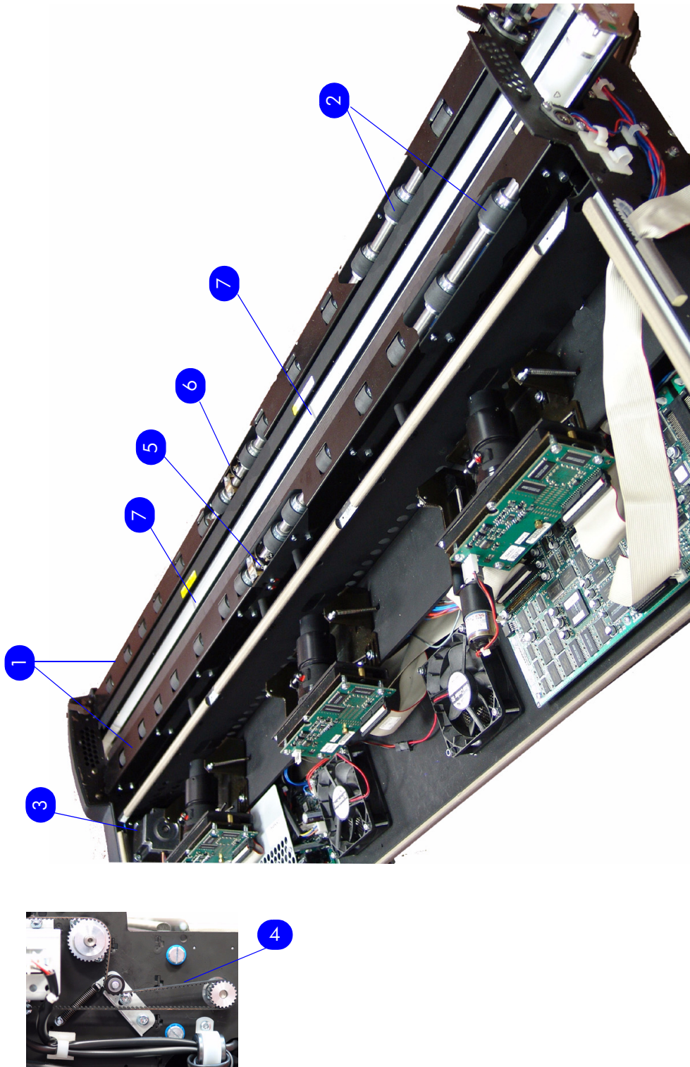
Figure 5: Drive Assemblies
