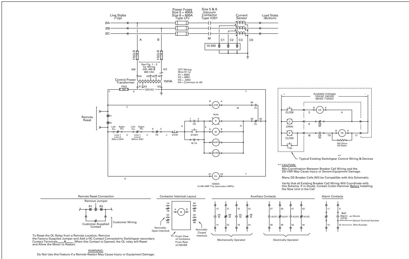
Figure 57-2. DS-VSR-540 Schematic
