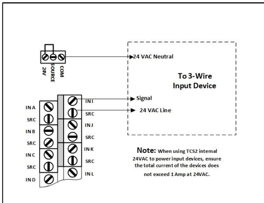
Figure 17: 3-Wire Input Device Wiring
