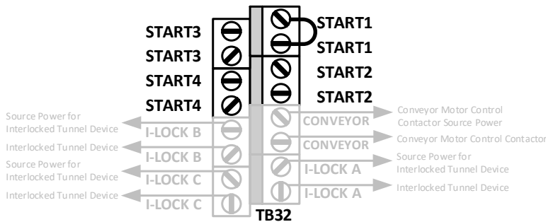
CONVEYOR CIRCUIT BOARD WIRING (Motherboard)
