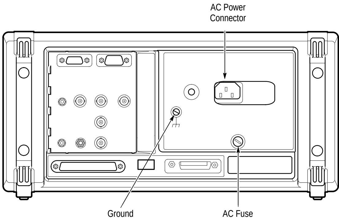
Figure 1–4: Rear-Panel Controls and Connectors Used in Setup
