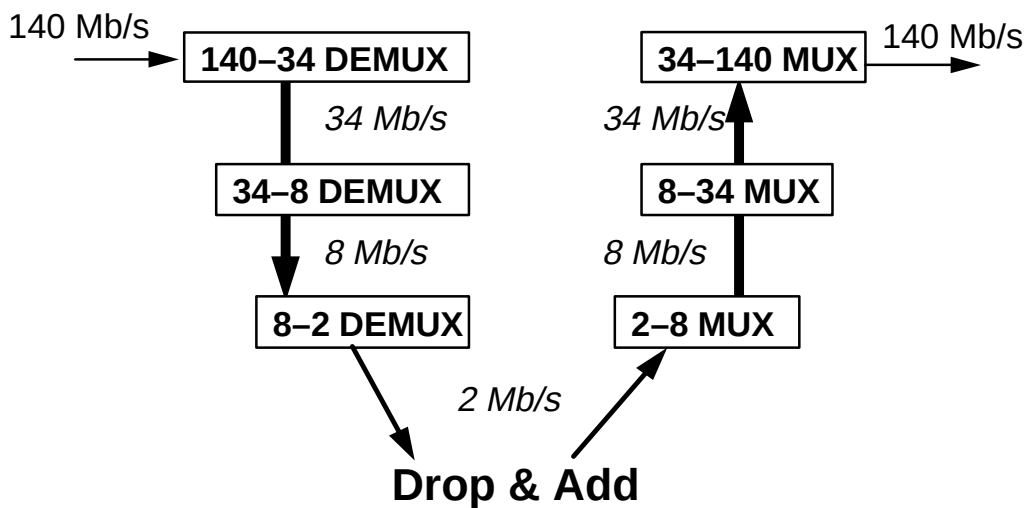
Figure 2–20: PDH Multiplexing by steps showing add/drop function
