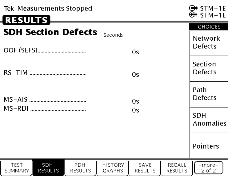
Figure 2-34: SDH Results, SDH Section Defects, from RESULTS menu
