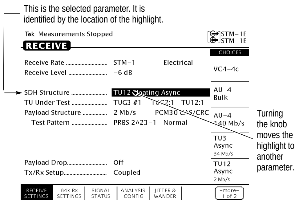
Figure 2–12: Selecting a Parameter
