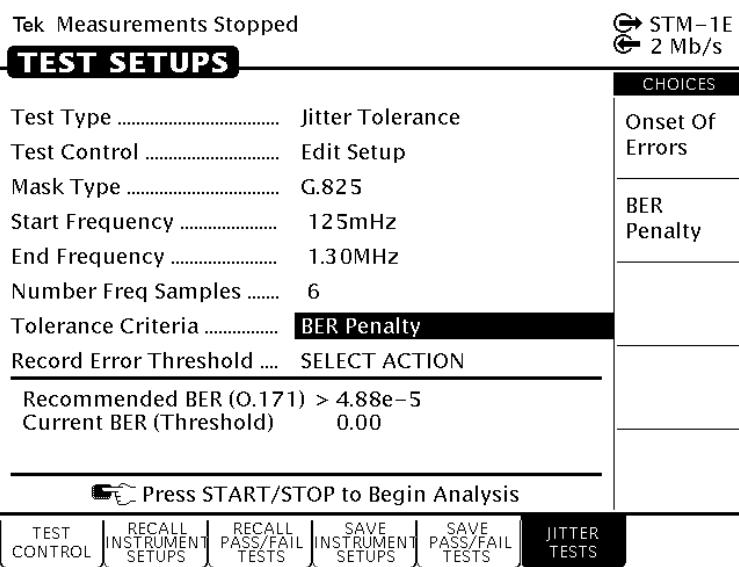
Figure 3-77: Example of TEST SETUP, Jitter Tests, BER Method
