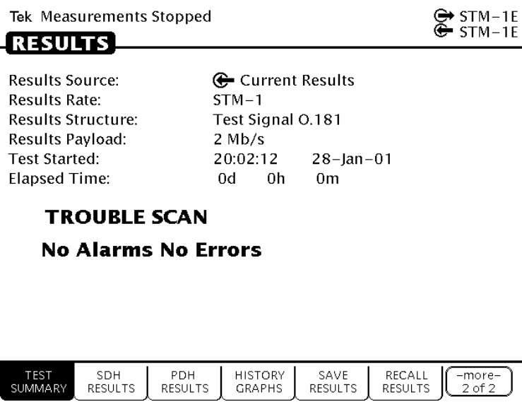
Figure 2–25: The TEST SUMMARY Page of the RESULTS Menu
