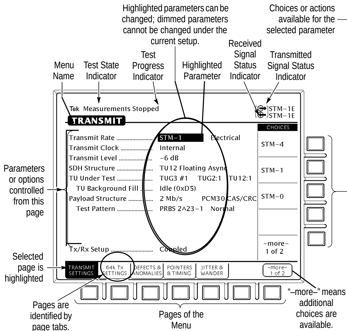
Figure 2–6: Specific Elements of the Display
