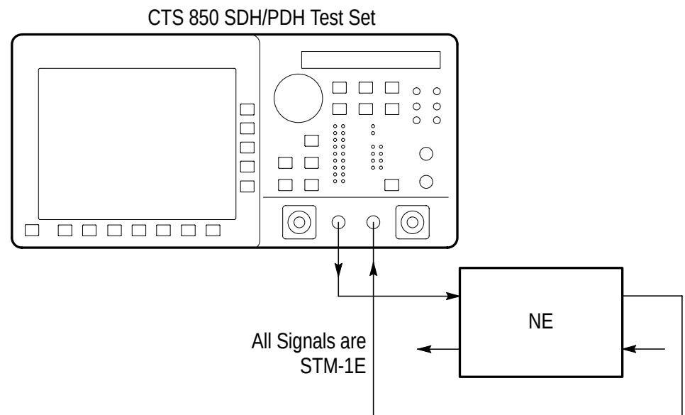
Figure 3–6: Setup to Check Line Frequency Offset Response
