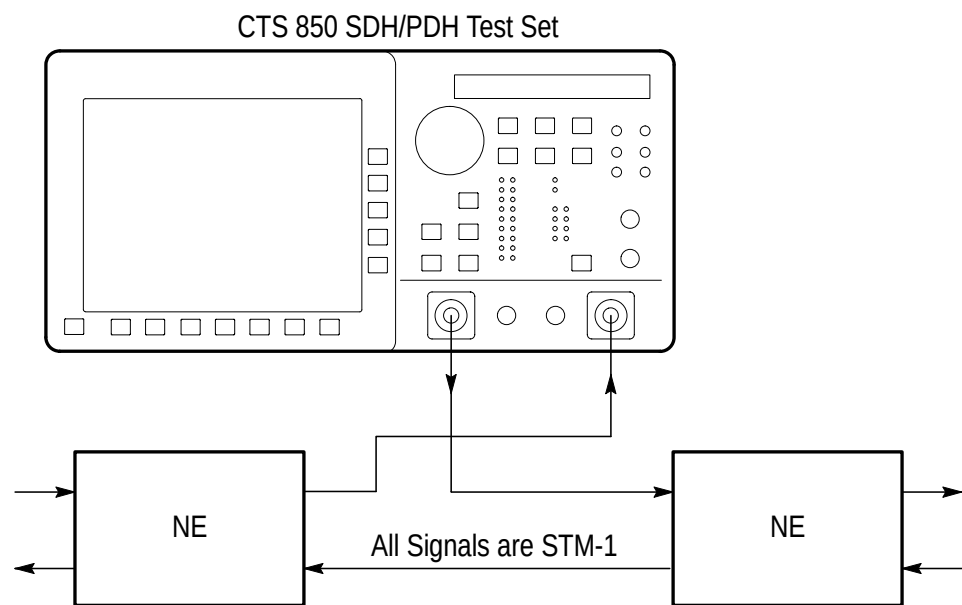
Figure 3-7: Setup to Monitor Performance
