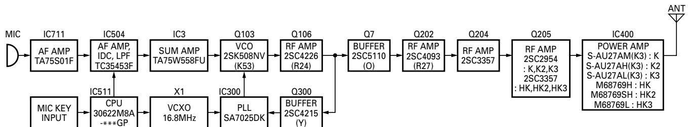
Fig. 6 Transmitter system
