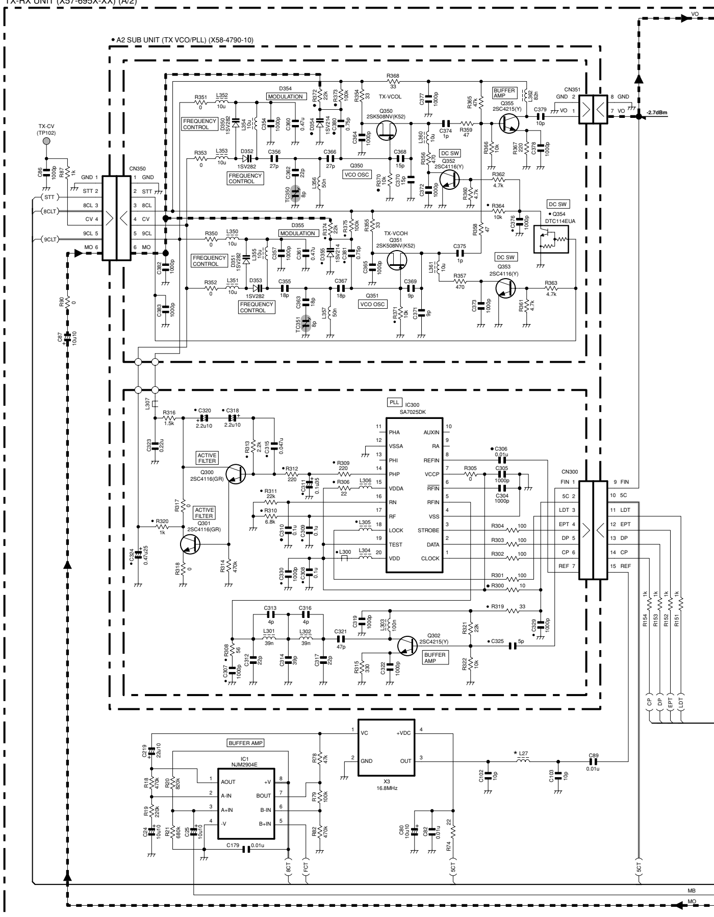
TX-RX UNIT (X57-695X-XX) (A/2)
