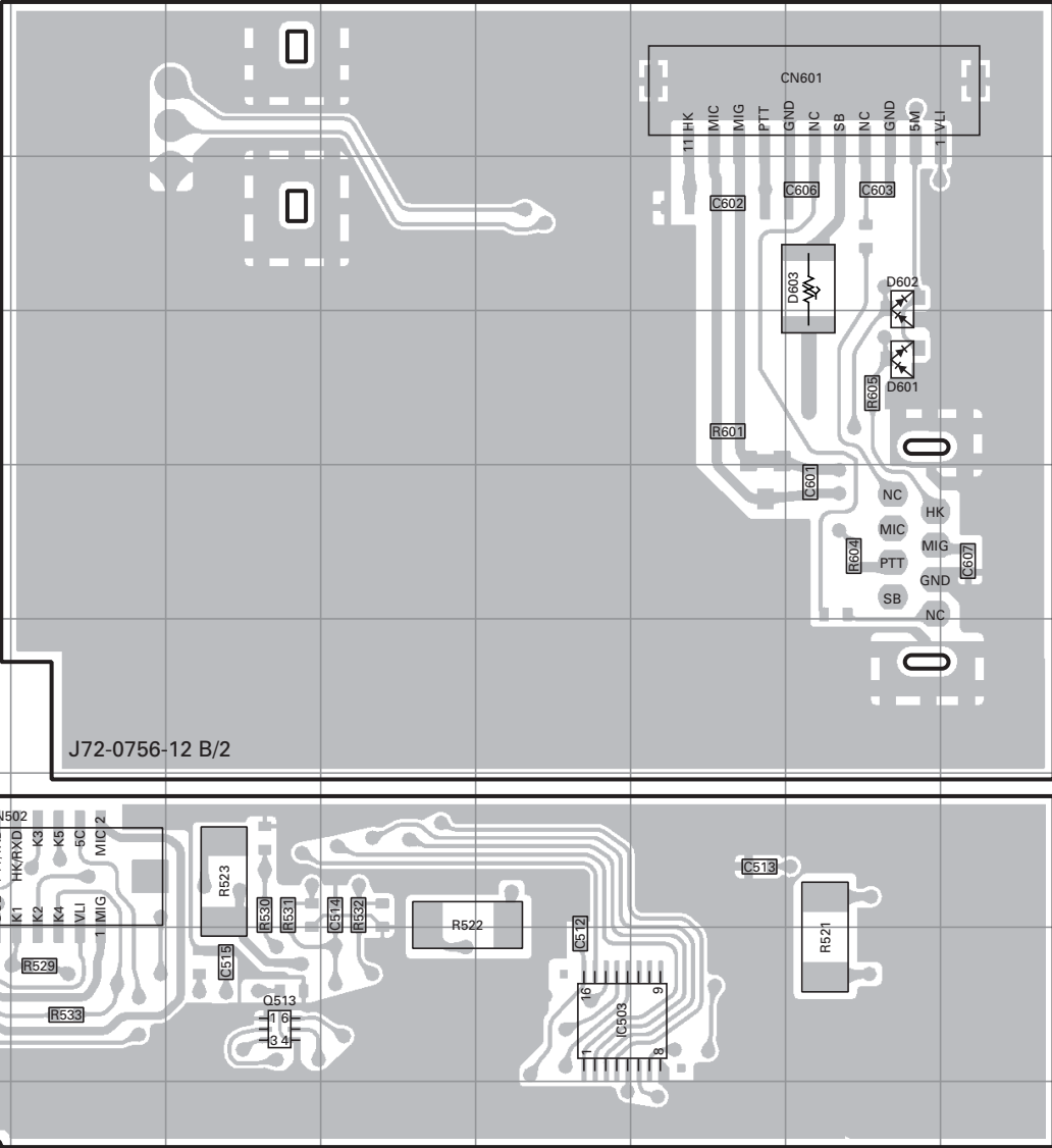
DISPLAY UNIT (X54-3330-21) Foil side view (J72-0756-12)
