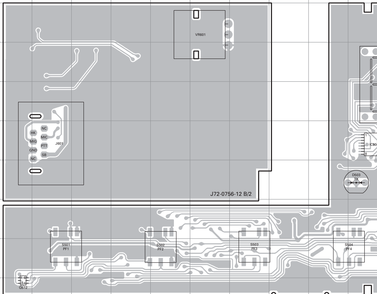
DISPLAY UNIT (X54-3330-21) Component side view (J72-0756-12)
