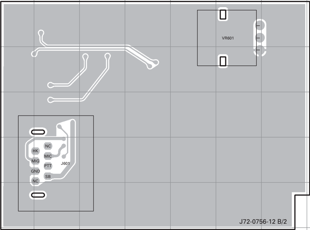
DISPLAY UNIT (X54-3330-21) Component side view (J72-0756-12)
