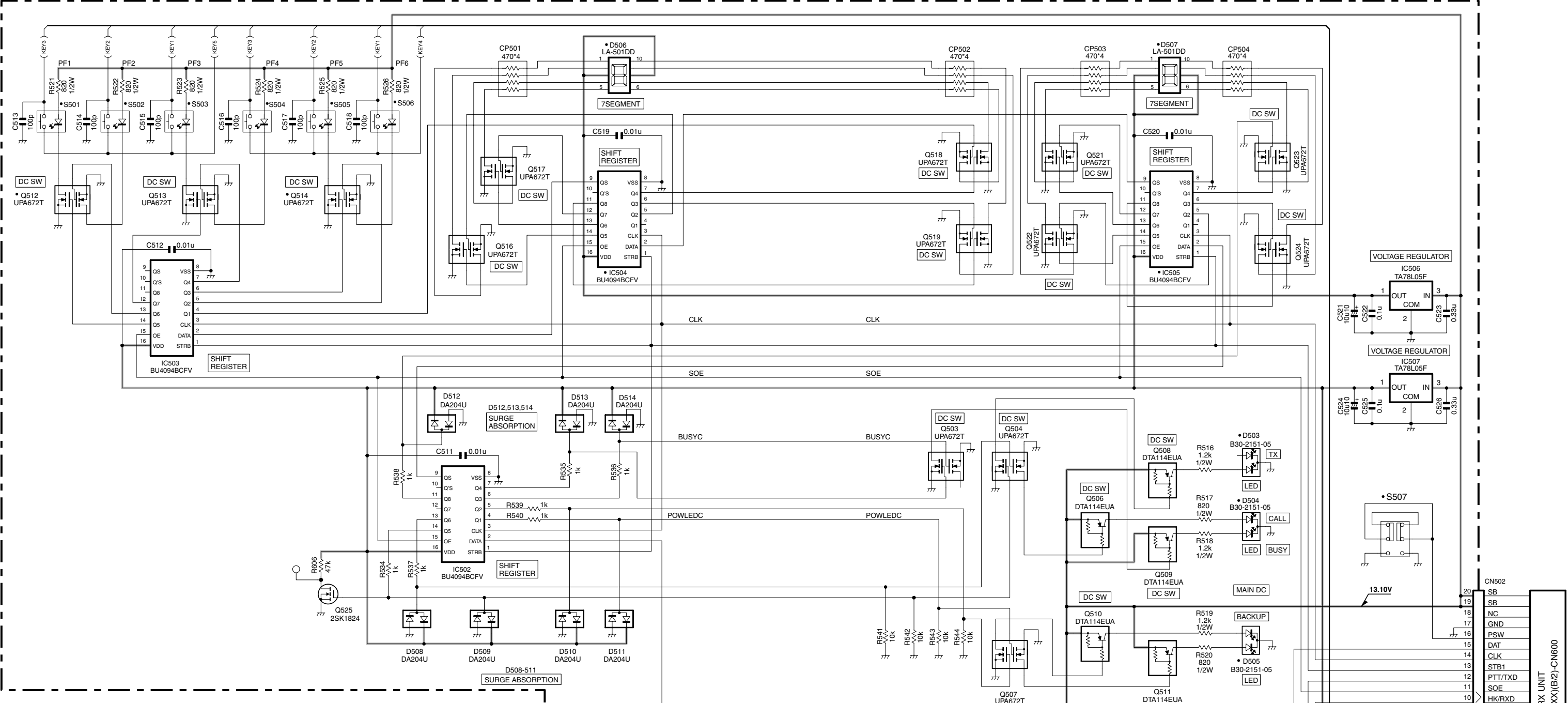
DISPLAY UNIT (X54-3330-21) (A/2)
