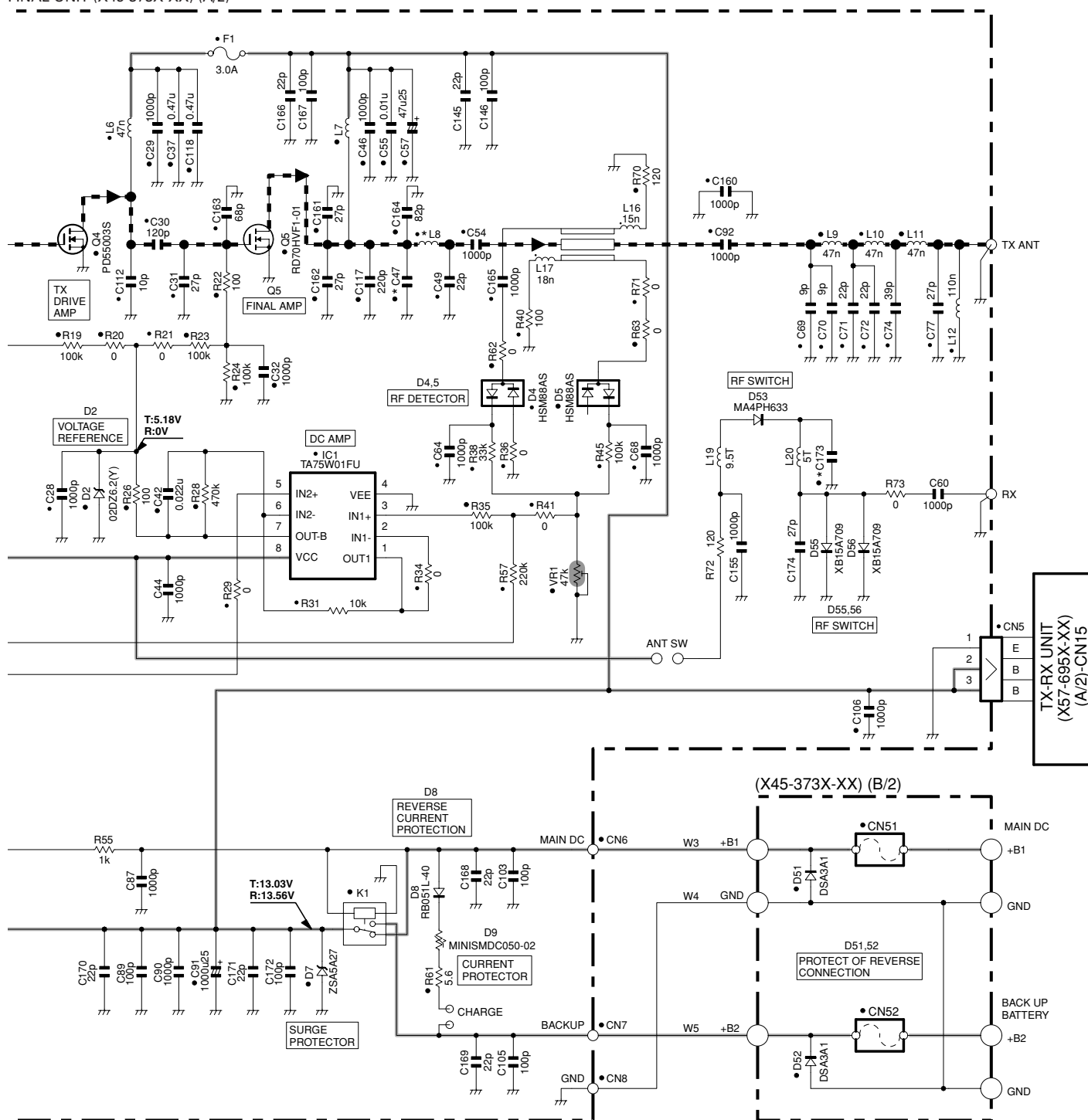
FINAL UNIT (X45-373X-XX) (A/2)
