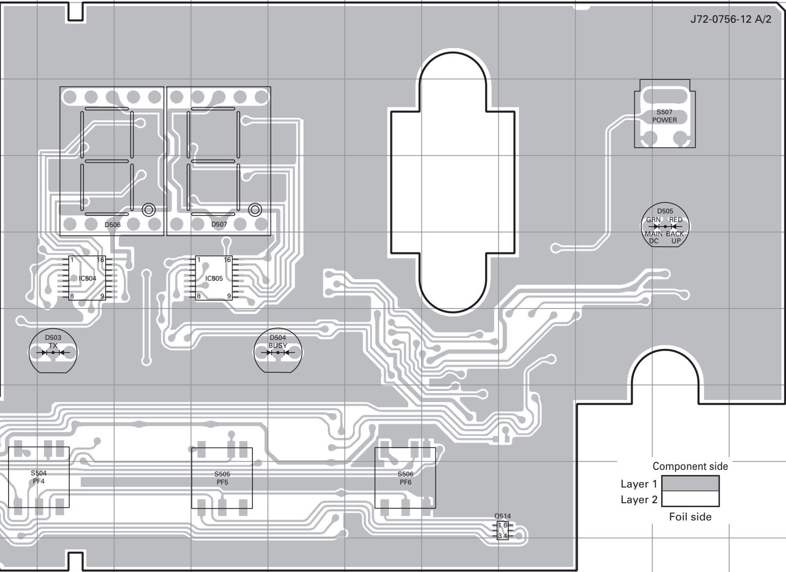
DISPLAY UNIT (X54-3330-21) Component side view (J72-0756-12)
