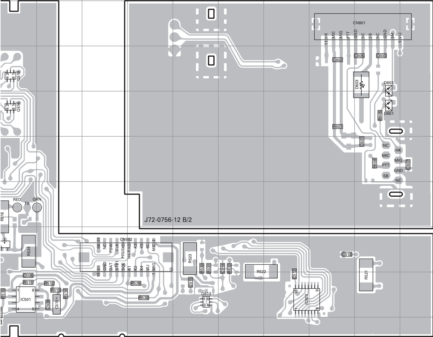
DISPLAY UNIT (X54-3330-21) Foil side view (J72-0756-12)
