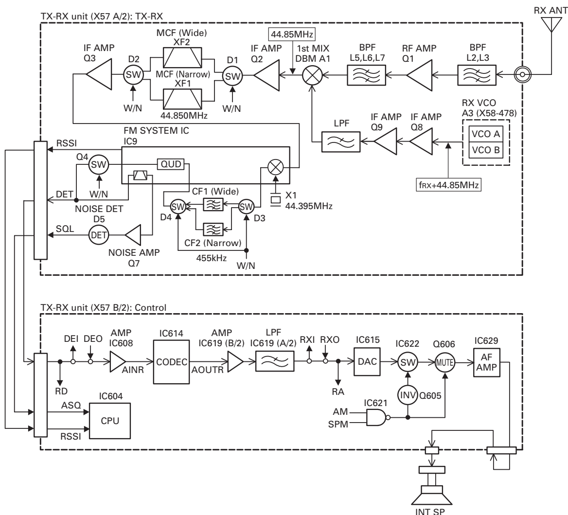
Fig. 1 Receiver circuit / 图1 接收机电路
