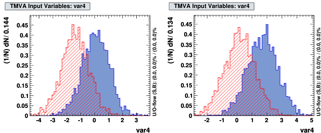
Figure 23: Examples for the usage of categories. The variable var4 depends on abs(eta) : for abs(eta) <= 1.3 (left plot), the signal and background Gaussian distributions are both shifted to lower values, while for abs(eta) > 1.3 (right plot) shifts to larger values have been applied. Ignoring this dependence, broadens the inclusive Gaussian distributions and generates variable correlations (here a coefficient of +0.4 between var3 and var4 ) due to the existence of distinct subsamples. The Category classifier treats the two cases independently, thus recovering optimal separation.
