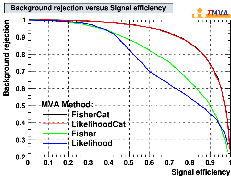
Figure 24: ROC curves for categorised and non-categorised Fisher and Projective Likelihood classifiers applied to an academic four-Gaussian example with eta -dependent mean values distinguishing two categories (cf. Fig. 23 for the category-dependent signal and background distributions of one of the four input variables). The categorised (“...Cat”) classifiers recover optimum performance (their red and black curves are superimposed).
