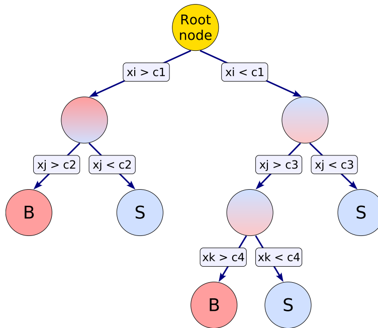
Figure 21: Schematic view of a decision tree. Starting from the root node, a sequence of binary splits using the discriminating variables x_i is applied to the data. Each split uses the variable that at this node gives the best separation between signal and background when being cut on. The same variable may thus be used at several nodes, while others might not be used at all. The leaf nodes at the bottom end of the tree are labeled “S” for signal and “B” for background depending on the majority of events that end up in the respective nodes. For regression trees, the node splitting is performed on the variable that gives the maximum decrease in the average squared error when attributing a constant value of the target variable as output of the node, given by the average of the training events in the corresponding (leaf) node (see Sec. 8.13.3).
