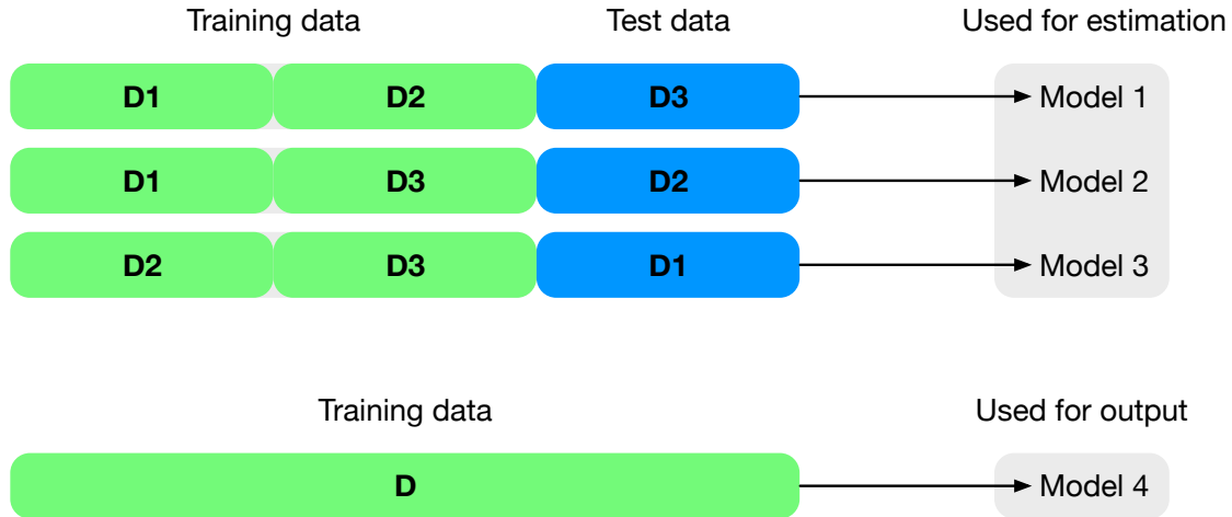
Figure 11: Model 1, 2, and 3 are used only for performance estimation and are then thrown away. A final model (model 4) is trained using the complete dataset.
