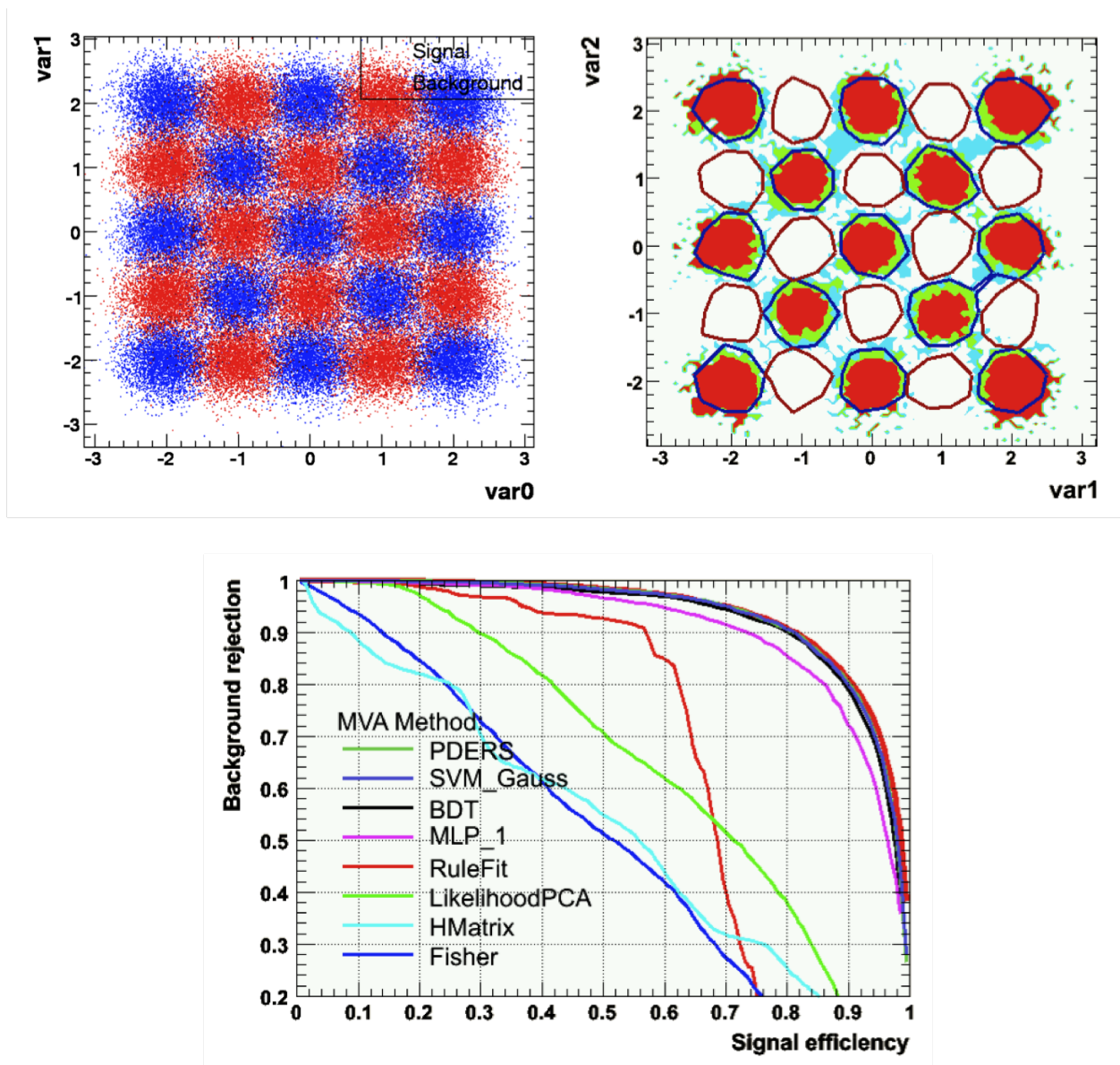
Figure 25: The top left plot shows the two-dimensional Gaussian-distributed signal (blue) and background (red) distributions for the “Schachbrett” toy Monte Carlo sample. In the top right plot is drawn as an example the Support Vector Machine’s classification response in terms of the weights given to events in the two dimensional plane. Dark red signifies large MVA output values, i.e. signal like event regions. The bottom plot gives the ROC curves obtained with several TMVA classifiers for this example after training. The theoretically best ROC curve is known and shown by the thick red outer line. While all the non-linear classification methods (after carefully tuning their parameters) are able to approximate the theoretical limit, the linear methods strongly underperform.
