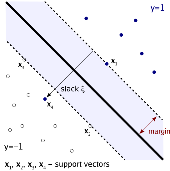
Figure 20: Hyperplane classifier in two dimensions. The vectors (events) \mathbf{x}_{1-4} define the hyperplane and margin, i.e., they are the support vectors.
