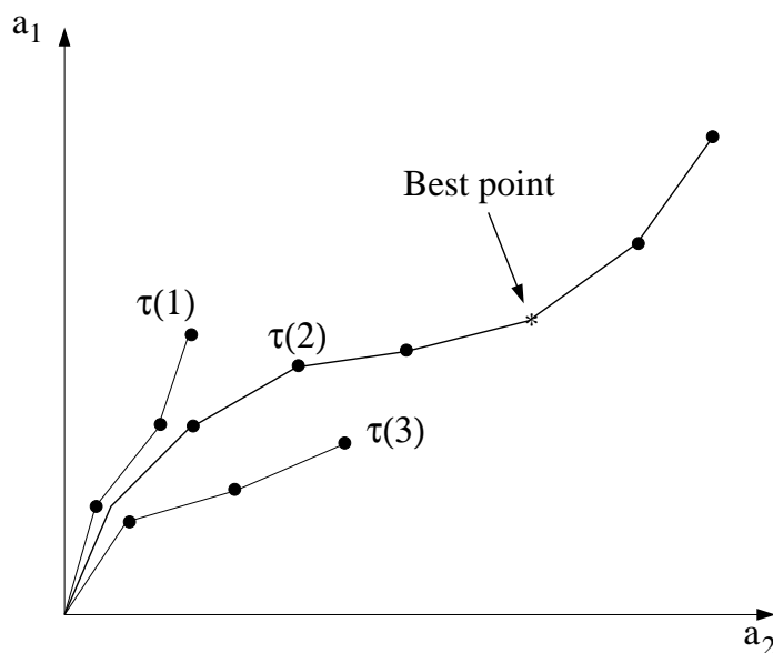
Figure 22: An example of a path scan in two dimensions. Each point represents an \epsilon in Eq. (117) and each step is given by \delta\epsilon . The direction along the path at each point is given by the vector \mathbf{g} . For the first few points, the paths \tau(1, 2, 3) are created with different values of \tau . After a given number of steps, the best path is chosen and the search is continued. It stops when the best point is found. That is, when the estimated error-rate is minimum.
