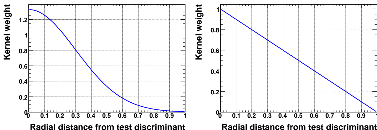
Figure 15: Kernel functions (left: Gaussian, right: Teepee) used to weight the events that are found inside the reference volume of a test event.
