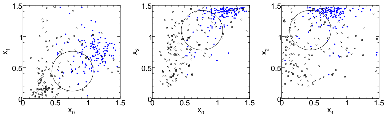
Figure 17: Example for the k-nearest neighbour algorithm in a three-dimensional space (i.e., for three discriminating input variables). The three plots are projections upon the two-dimensional coordinate planes. The full (open) circles are the signal (background) events. The k-NN algorithm searches for 20 nearest points in the nearest neighborhood (circle) of the query event, shown as a star. The nearest neighborhood counts 13 signal and 7 background points so that query event may be classified as a signal candidate.
