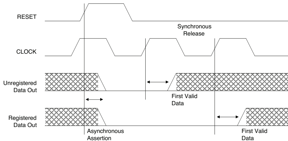
Figure 7. Asynchronous Reset with Synchronous Release
