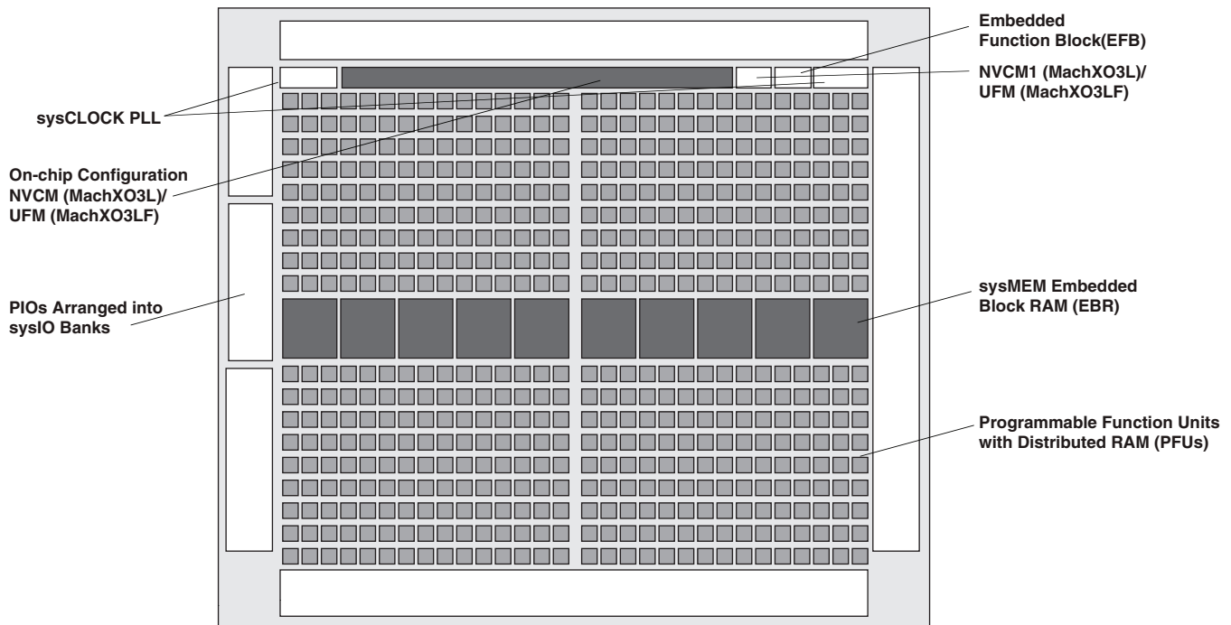
Figure 2. Top View of the MachXO3L/LF-4300 Device
