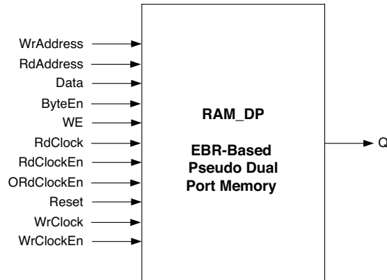
Figure 23. Pseudo Dual Port Memory Module Generated by IPexpress
