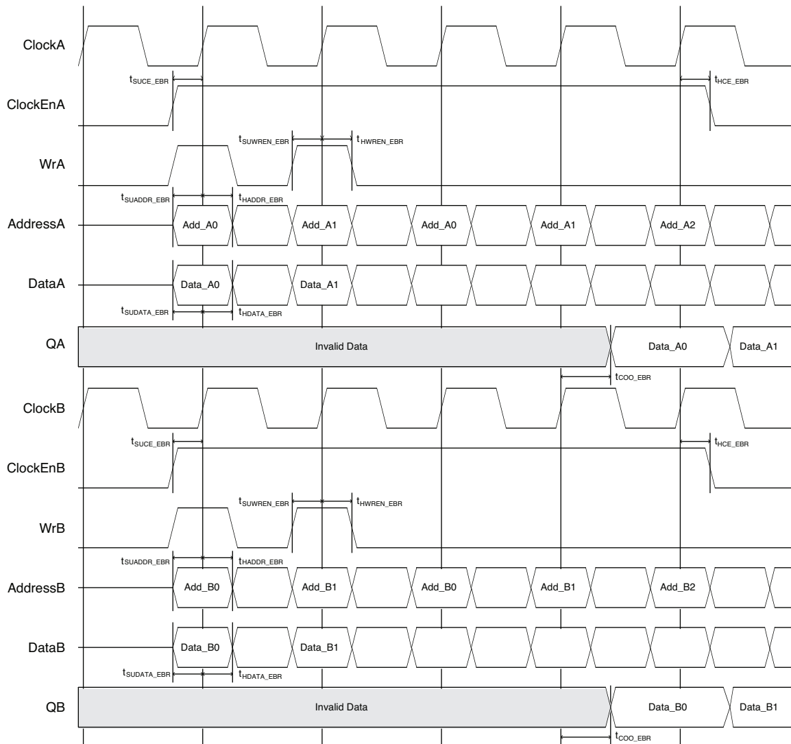
Figure 18. True Dual Port RAM Timing Waveform – NORMAL Mode with Output Registers
