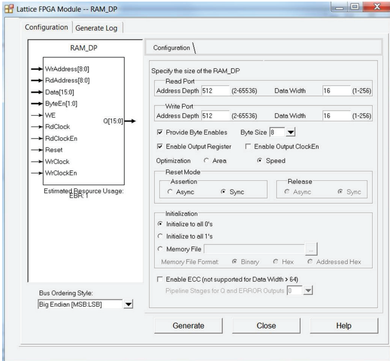
Figure 5. Example Generating Pseudo Dual Port RAM (RAM_DP) Module Customization (MachXO3L)
