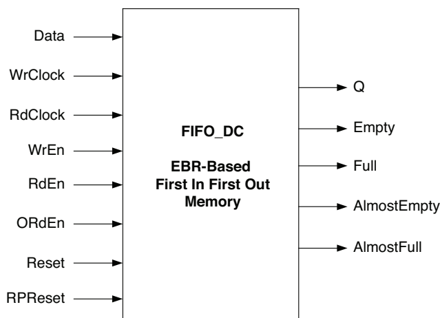
Figure 29. FIFO Module Generated by IPexpress
