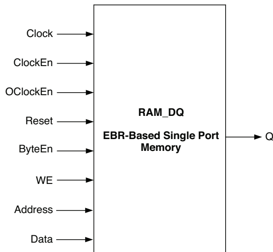
Figure 9. Single Port Memory Module Generated by IPexpress
