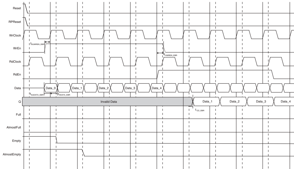
Figure 31. FIFO_DC With Output Registers (Pipelined)
