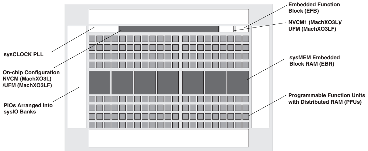
Figure 2. Top View of the MachXO3L/LF-4300 Device
