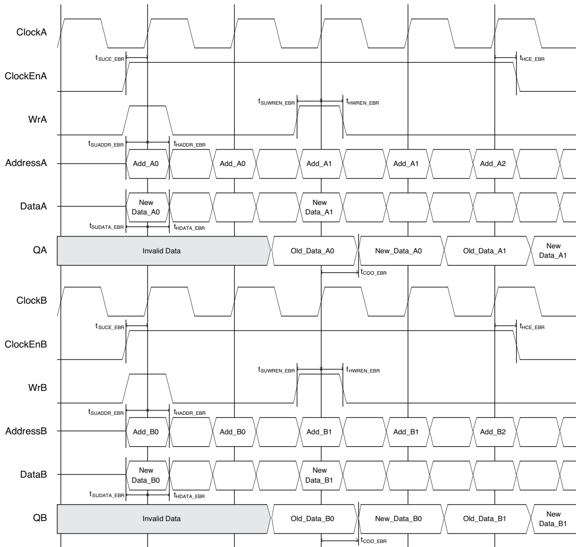
Figure 20. True Dual Port RAM Timing Waveform – READ BEFORE WRITE Mode, with Output Registers
