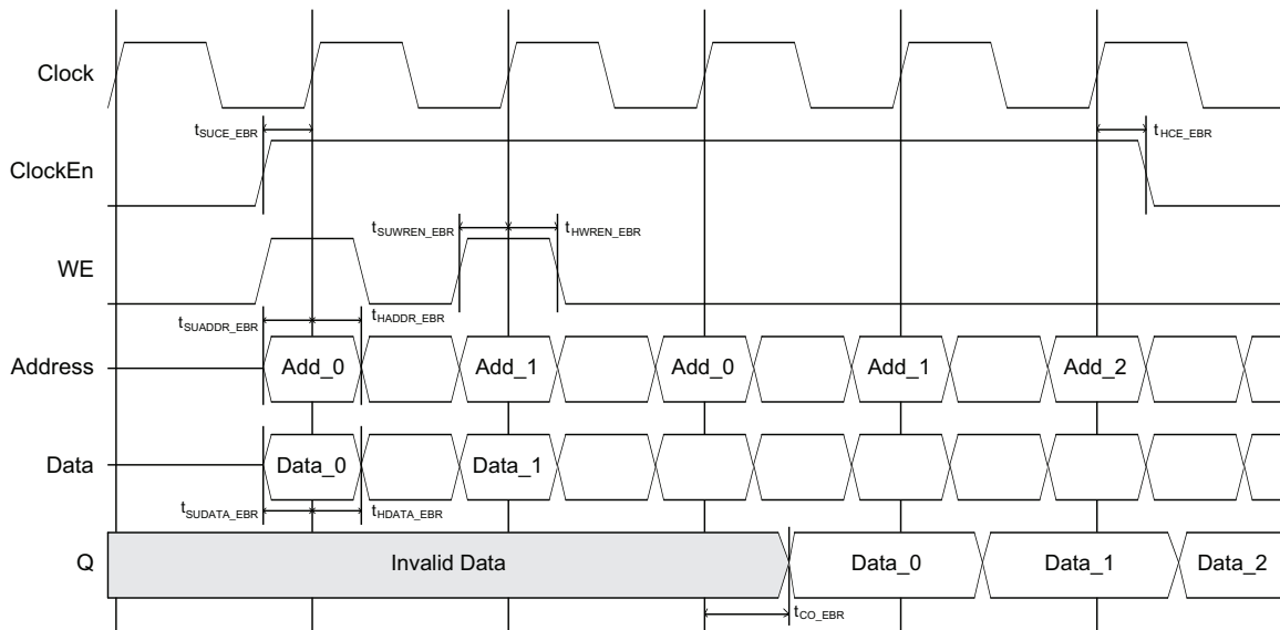
Figure 11. Single Port RAM Timing Waveform – NORMAL Mode, With Output Registers
