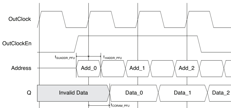
Figure 40. PFU-Based ROM Timing Waveform – With Output Registers
