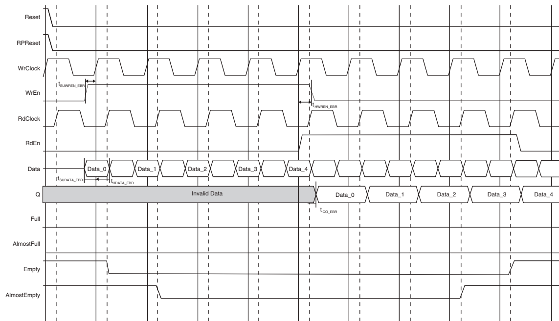
Figure 30. FIFO_DC Without Output Registers (Non-Pipelined)
