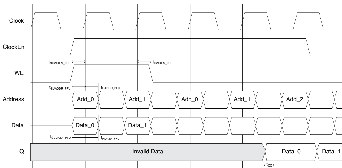
Figure 34. PFU- Based Distributed Single Port RAM Timing Waveform – With Output Registers
