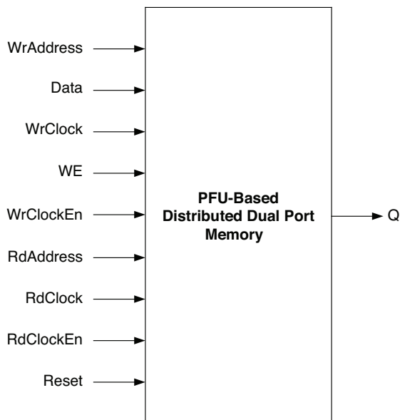
Figure 35. Distributed Dual Port RAM Module Generated by IPexpress
