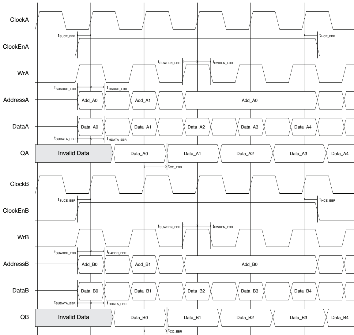
Figure 21. True Dual Port RAM Timing Waveform – WRITE THROUGH Mode, without Output Registers
