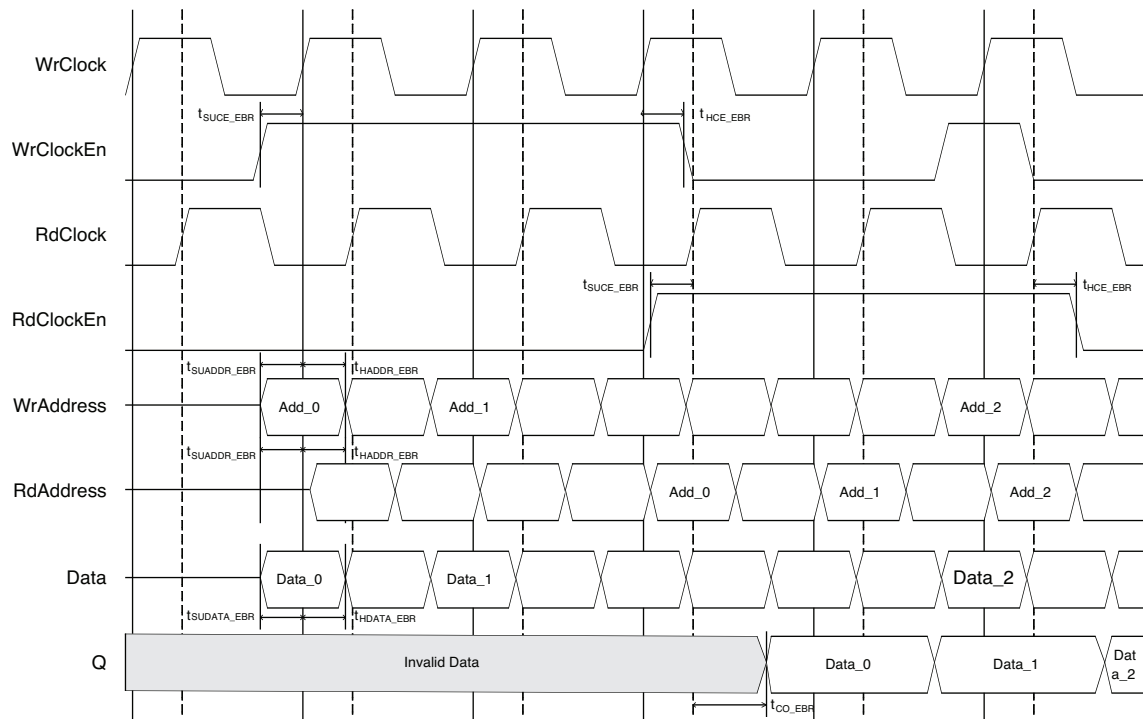
Figure 24. Pseudo-Dual Port RAM Timing Diagram – Without Output Registers
