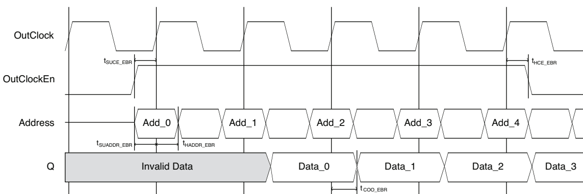
Figure 28. ROM Timing Waveform – With Output Registers
