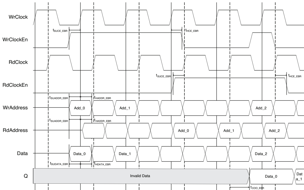
Figure 25. Pseudo-Dual Port RAM Timing Diagram – With Output Registers
