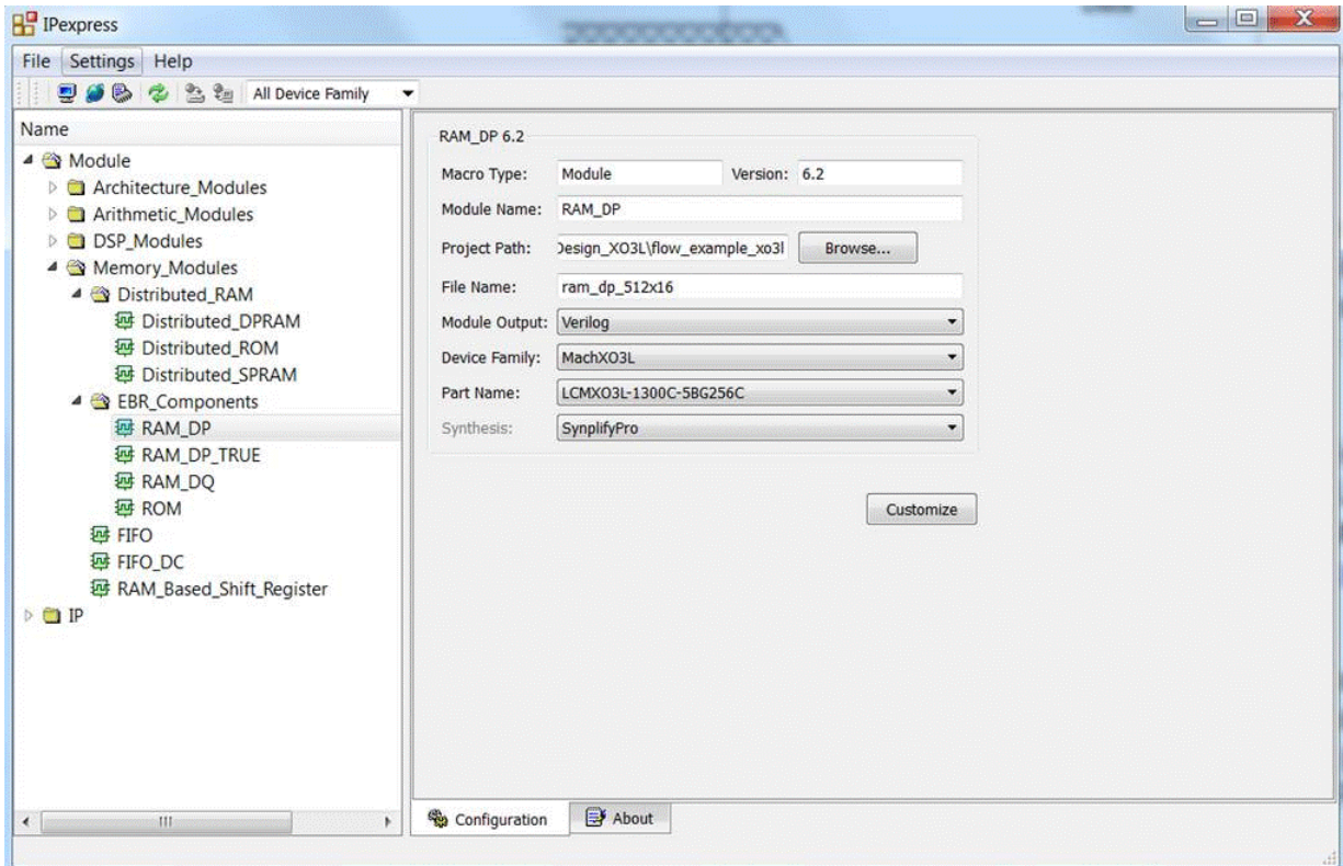
Figure 4. Example Generating Pseudo Dual Port RAM (RAM_DP) Using IPexpress
