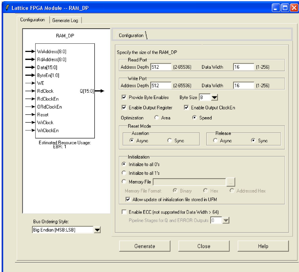
Figure 6. Example Generating Pseudo Dual Port RAM (RAM_DP) Module Customization (MachXO3LF)
