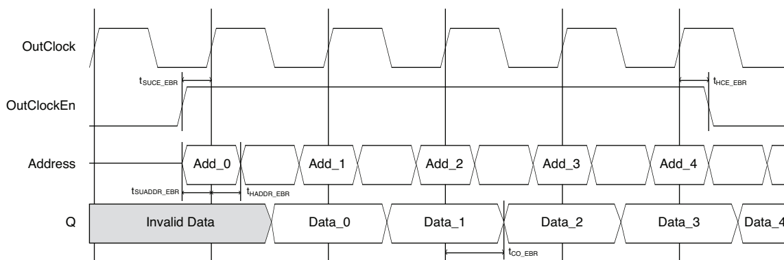
Figure 28. ROM Timing Waveform – With Output Registers
