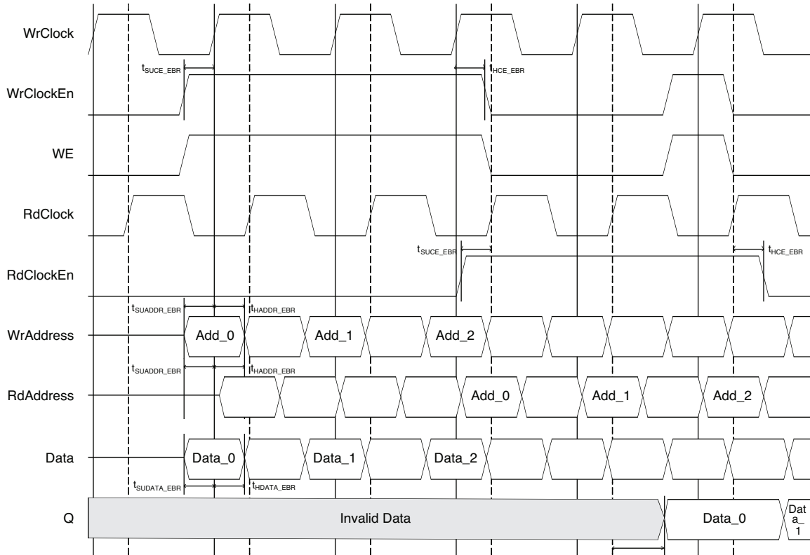
Figure 37. PFU-Based Distributed Dual Port RAM Timing Waveform – With Output Registers
