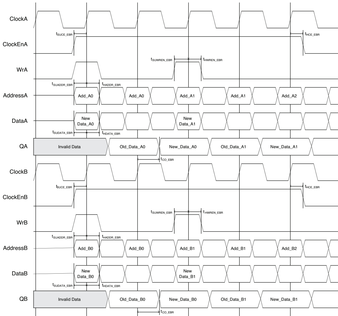
Figure 19. True Dual Port RAM Timing Waveform – READ BEFORE WRITE Mode, without Output Registers
