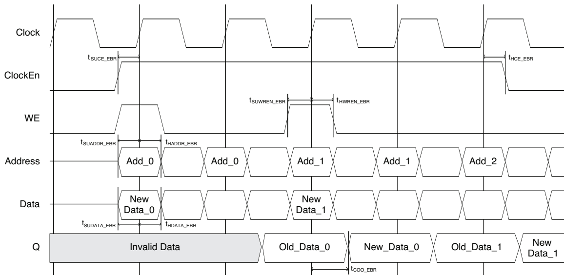
Figure 13. Single Port RAM Timing Waveform – READ BEFORE WRITE Mode, With Output Registers
