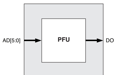
Figure 53. Distributed_ROM Primitive (ROM128X1A)
