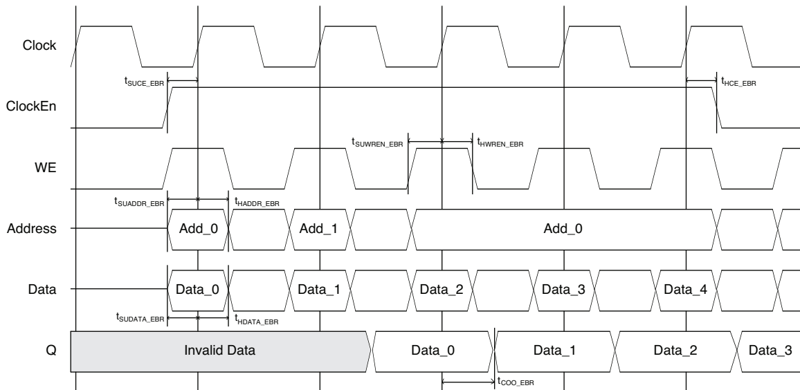
Figure 15. Single Port RAM Timing Waveform – WRITE THROUGH Mode, With Output Registers
