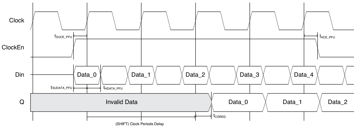
Figure 43. RAM-Based Shift Register Timing Waveform – With Output Registers (Shift = 2)
