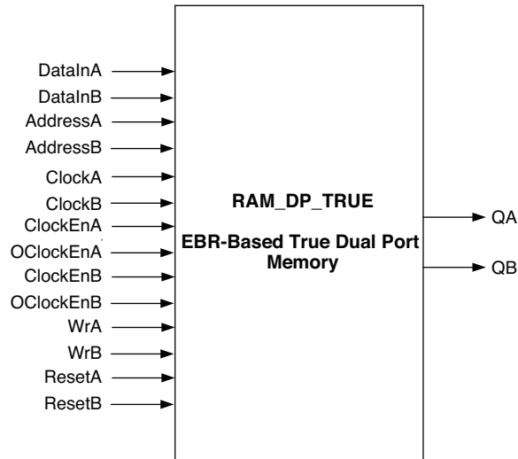
Figure 16. True Dual Port Memory Module Generated by IPexpress
