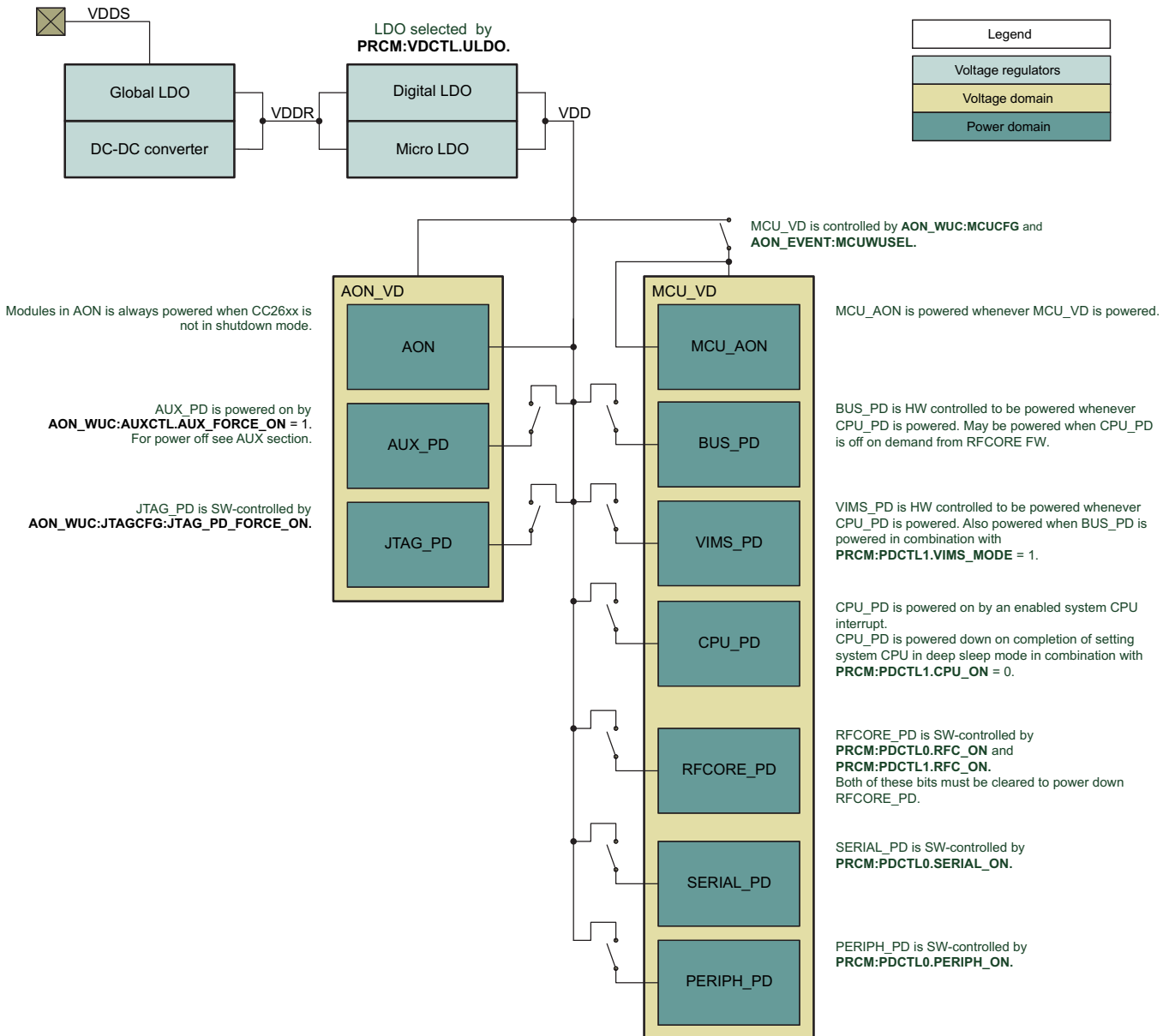
Figure 6-2. CC26xx and CC13xx Supply System
