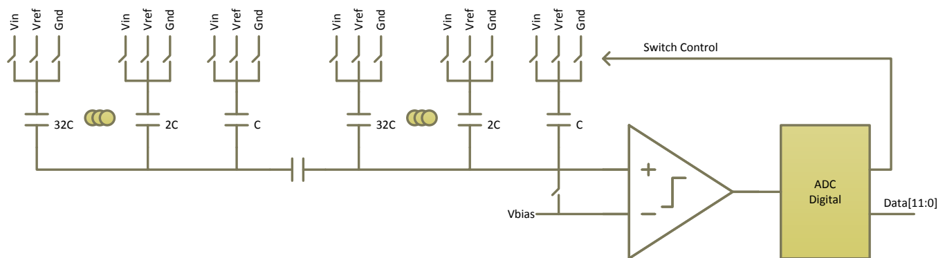
Figure 17-2. ADC Block Diagram
