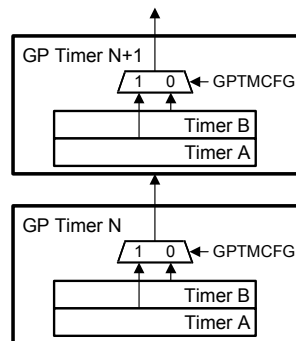
Figure 13-8. Timer Daisy-chain
