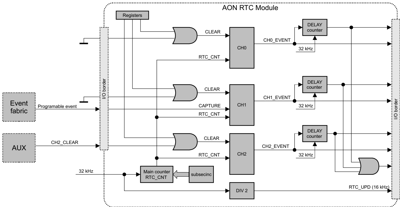
Figure 14-1. AON_RTC Channels
