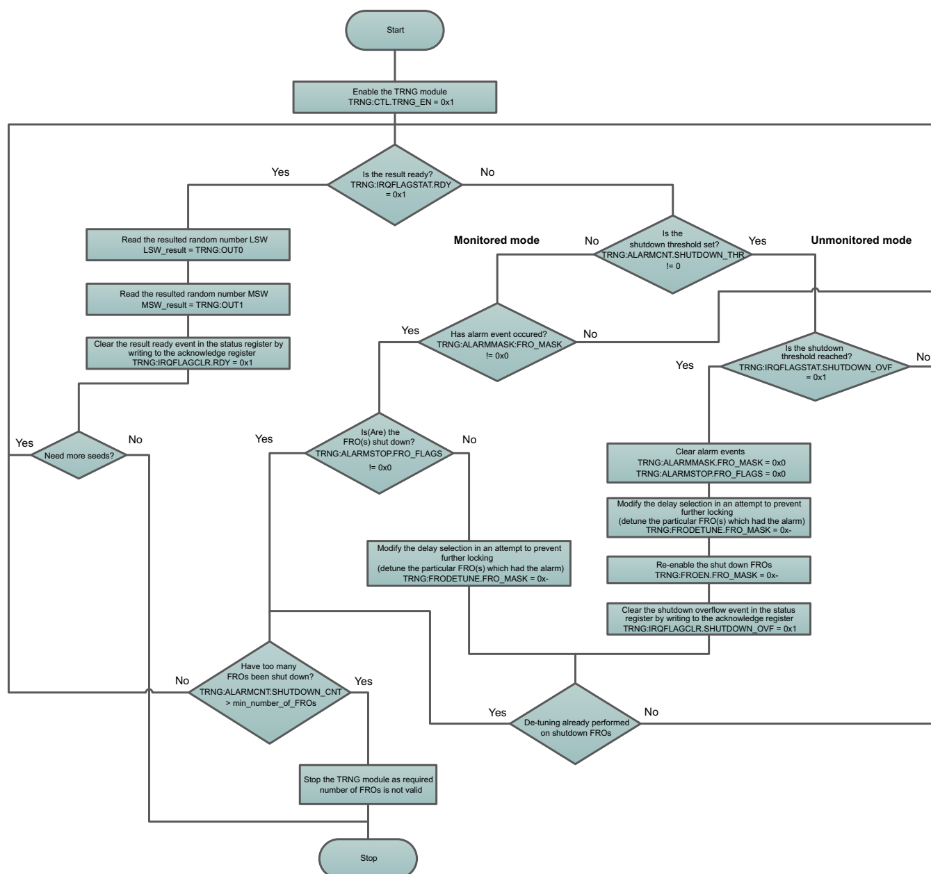
Figure 16-2. TRNG Polling Mode
