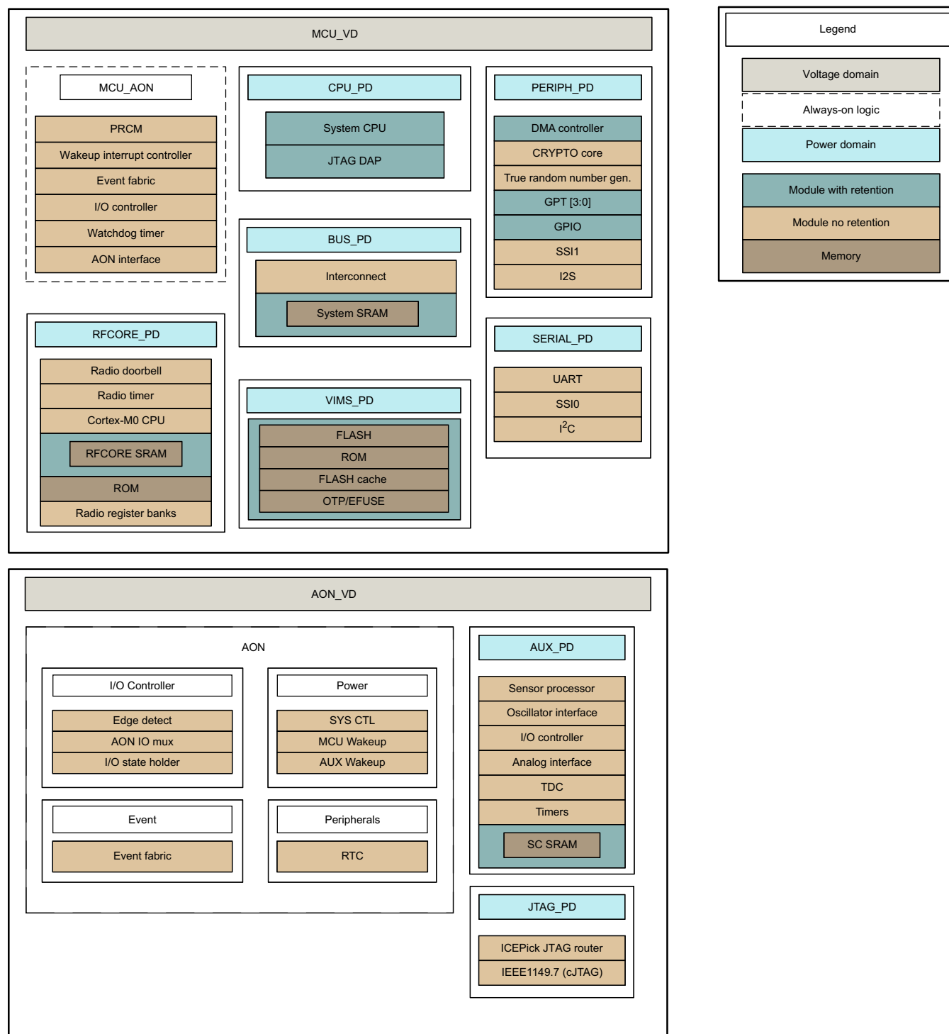
Figure 6-3. Digital Power Partitioning in CC26xx and CC13xx
