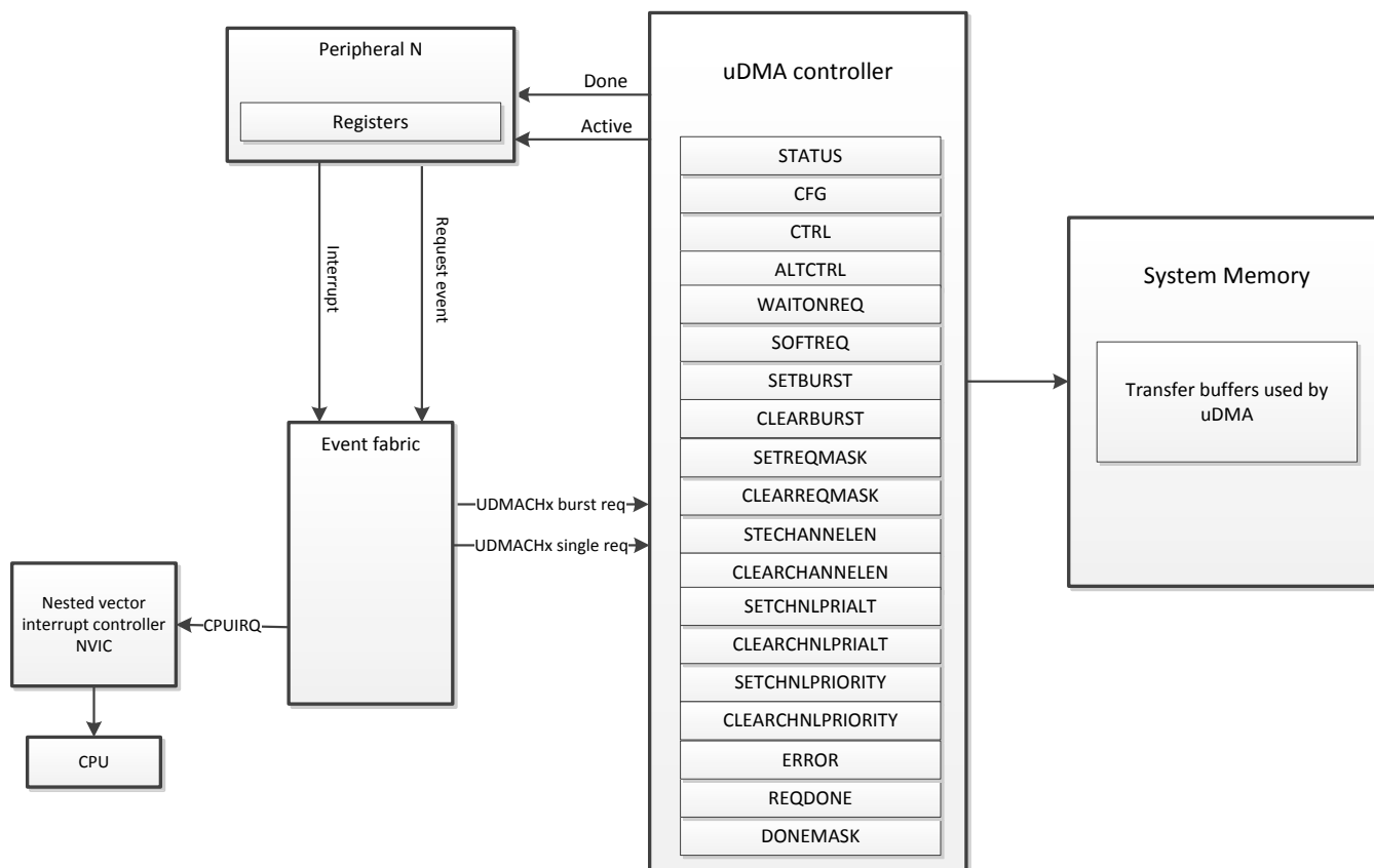
Figure 12-1. \mu DMA Block Diagram
