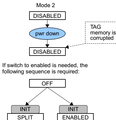
Figure 7-8. GPRAM Retention
