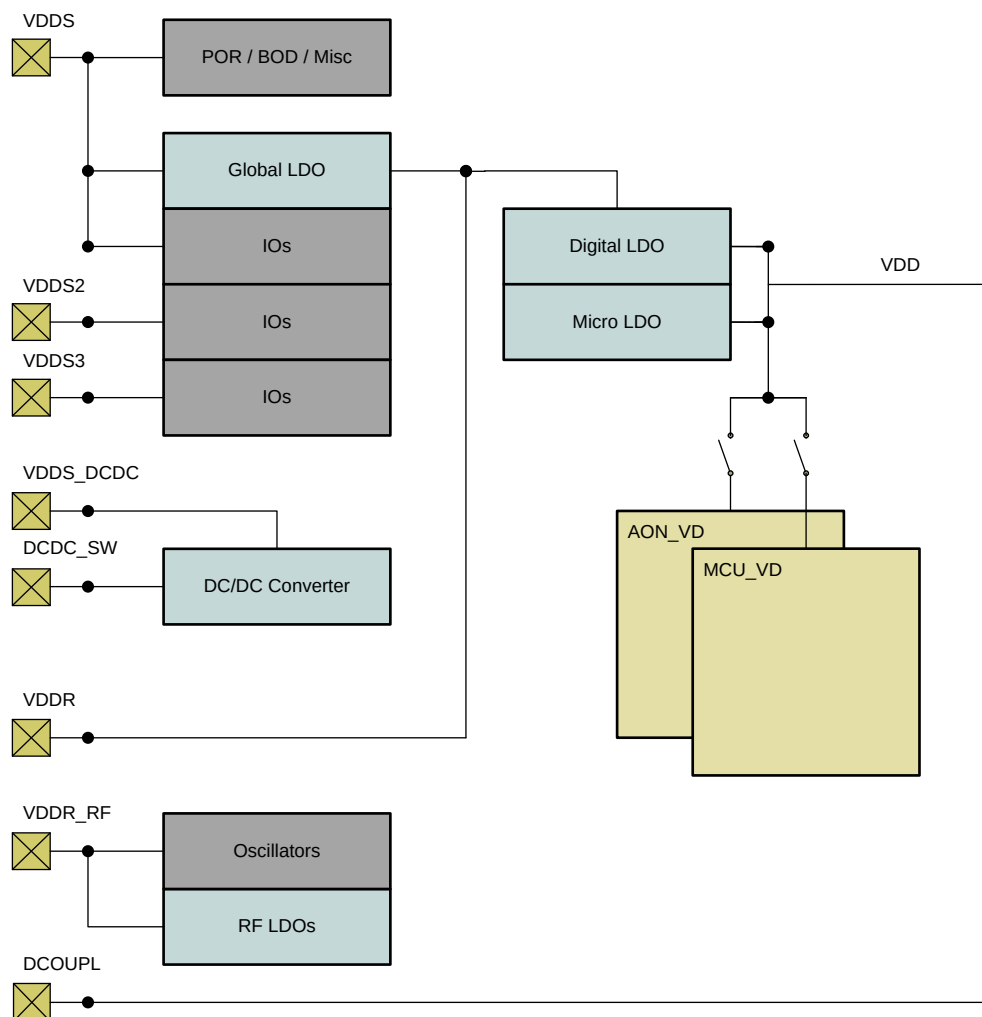
Figure 1-2. CC26xx and CC13xx Supply System
