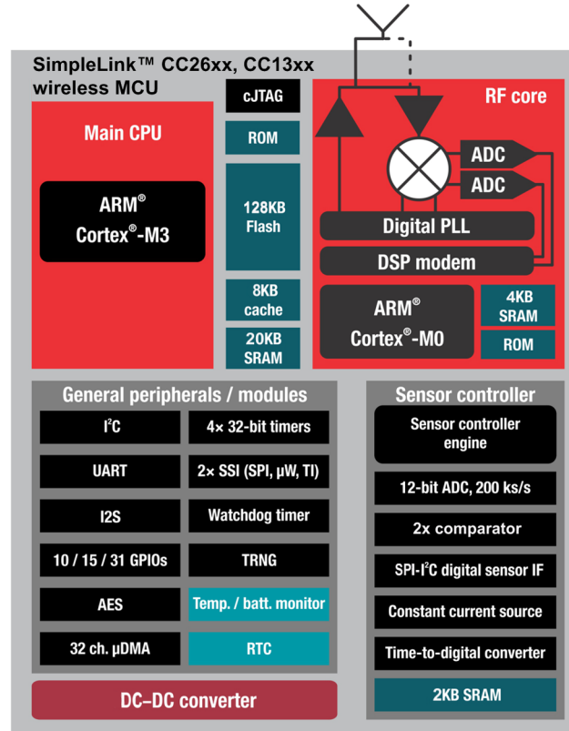
Figure 1-1. CC26xx and CC13xx Block Diagram
