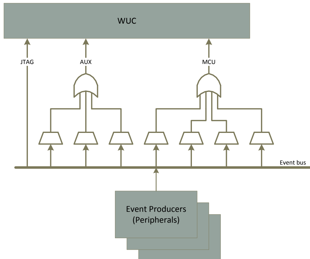
Figure 4-5. WUC Subscriber in AON Event Fabric
