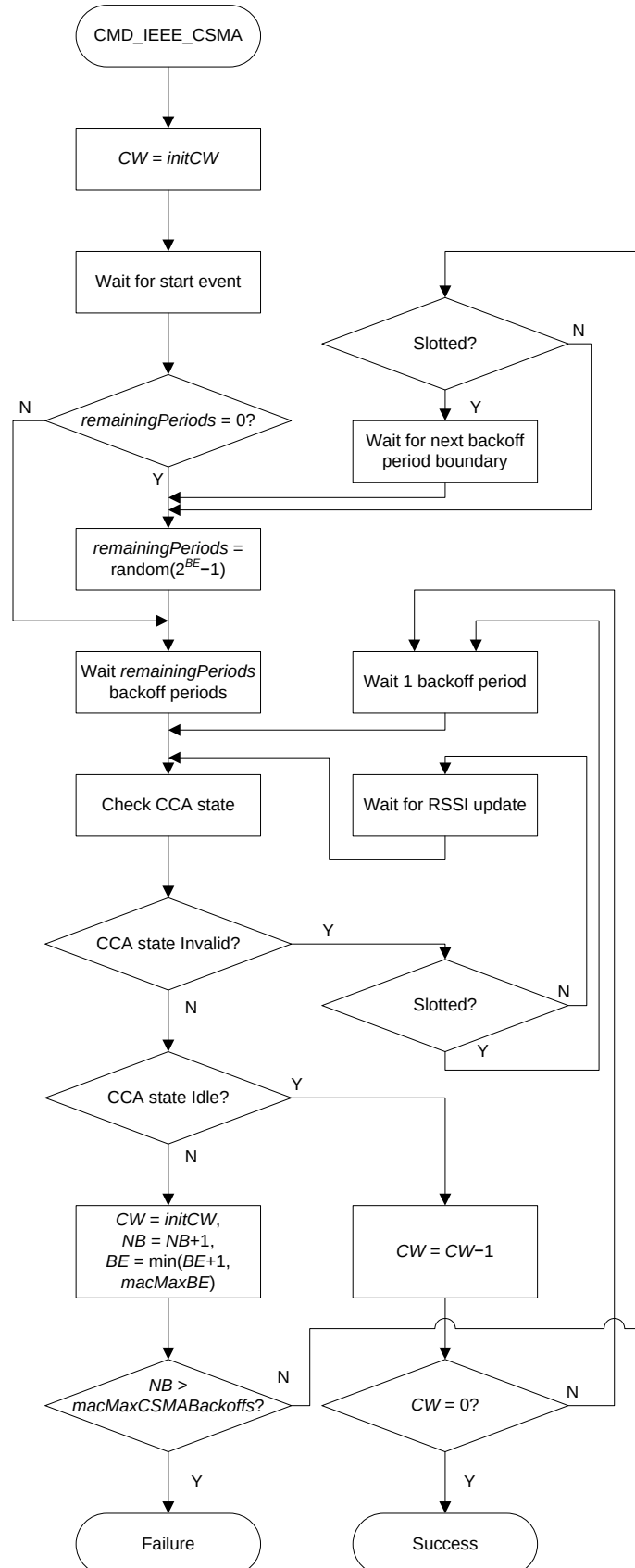
Figure 23-7. CSMA-CA Operation
