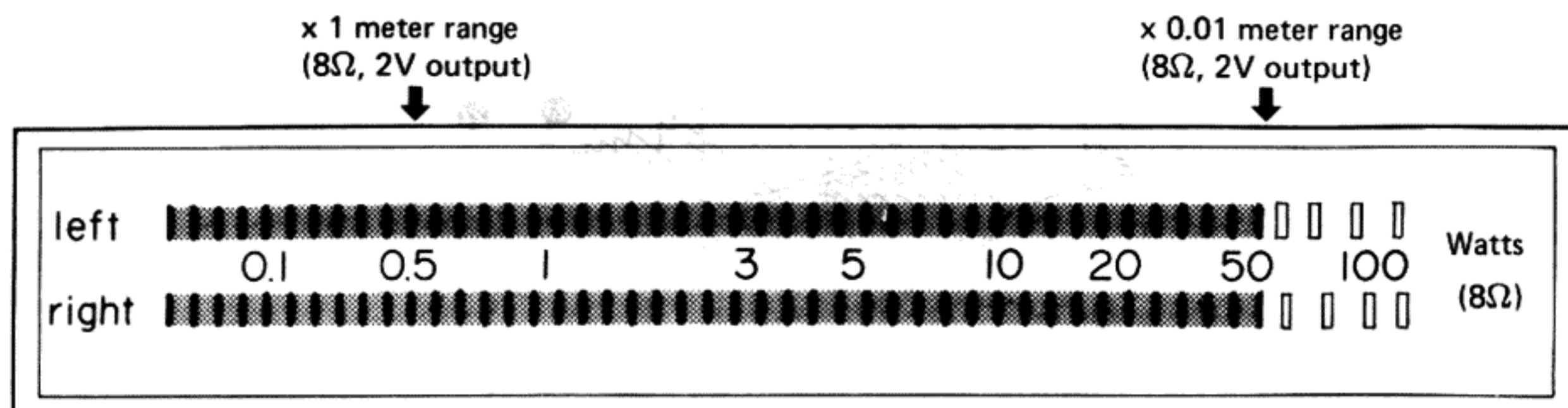
FL peak power meter: Fig. 19 (Abb. 19)
