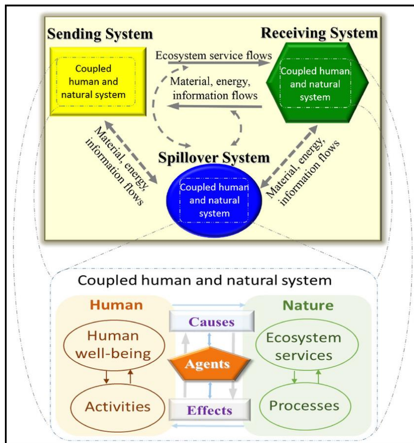
Figure 1. Framing ES in a telecoupling context (adapted from Liu et al. 2013). A “sending” system provides ES to a “receiving” system, and may influence another system (the “spillover” system) in the process. Feedbacks occur among different systems as a result of material energy, and information flows. Each system represents a coupled human and natural system, with two major components: humans and
