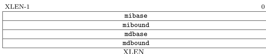
Figure 3.23: Separate instruction and data base-and-bound registers.
