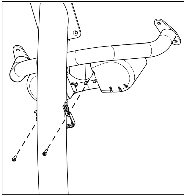
Figure 7: Installing the bottle holder
