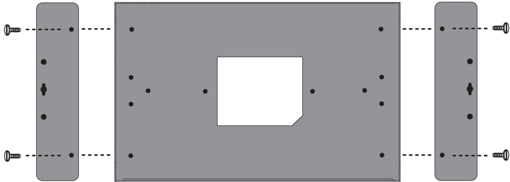
Figure A: UC-7420/7410 Universal Communicator—Wall Mounting Brackets (bottom view)
