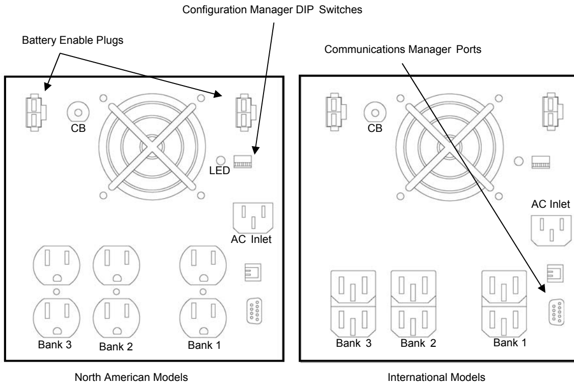
Figure 5 – Rear Panel 1440 VA Models
