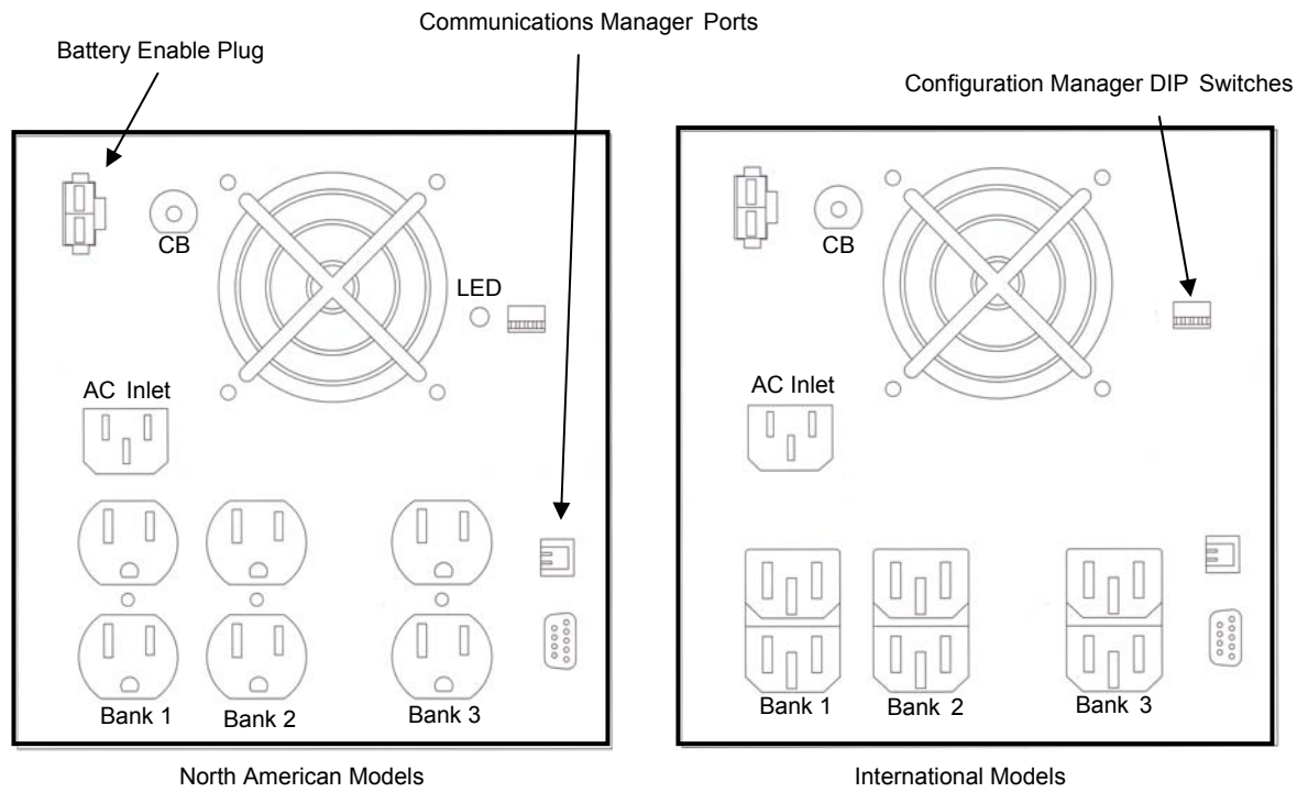
Figure 5 – Rear Panel 1100 VA Models
