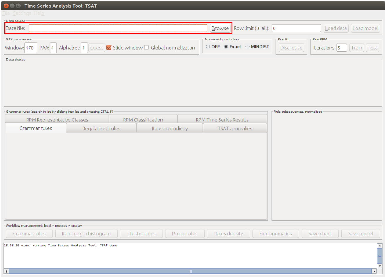
Figure 29: Loading a model
