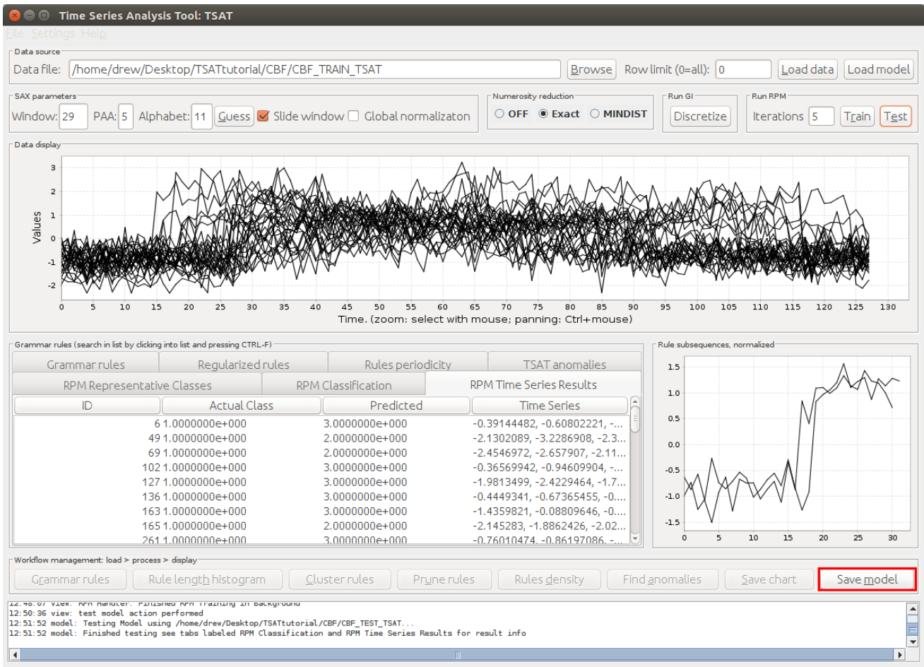
Figure 27: Saving the RPM model
