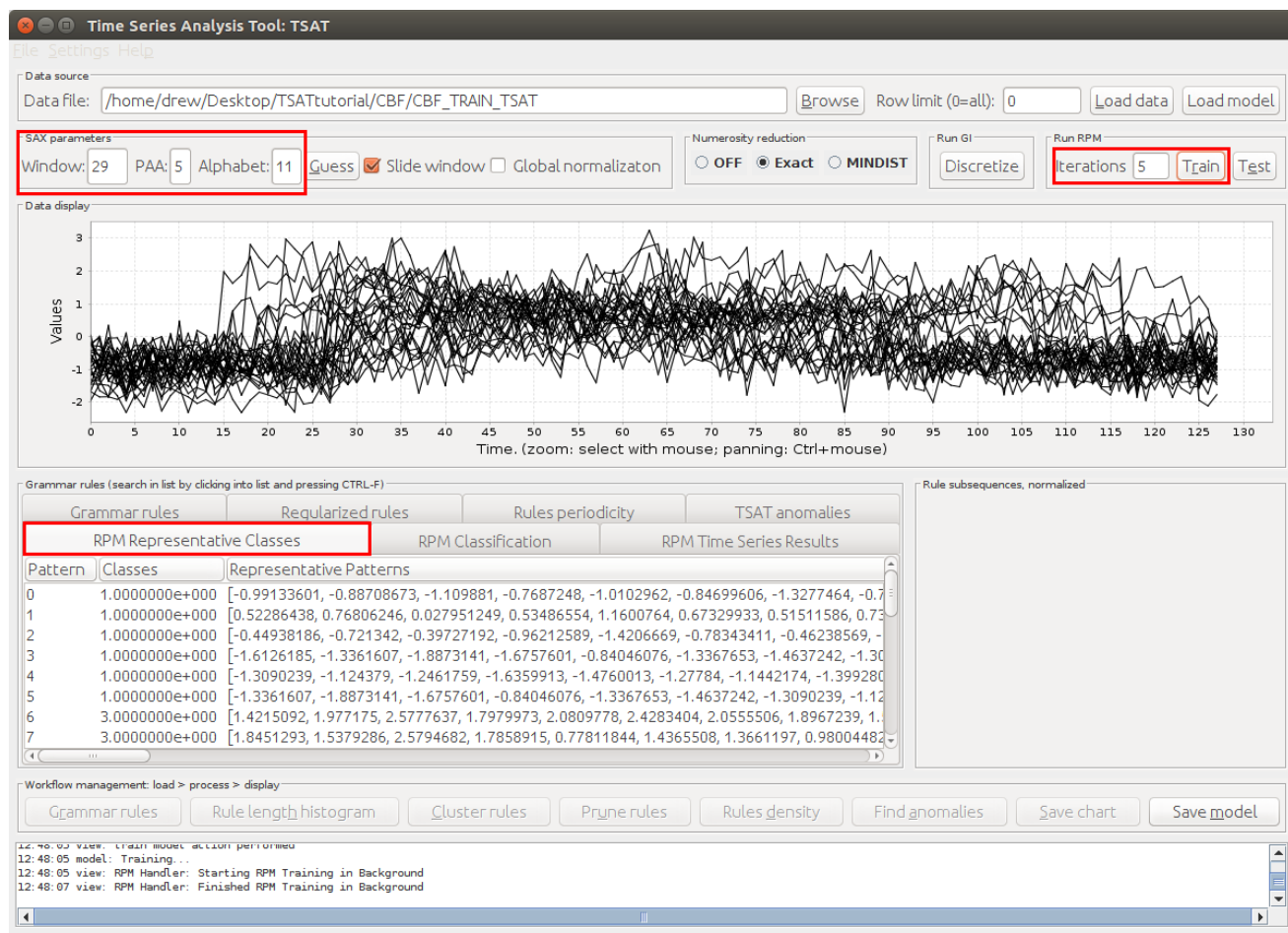
Figure 21: Representative Classes after Training
