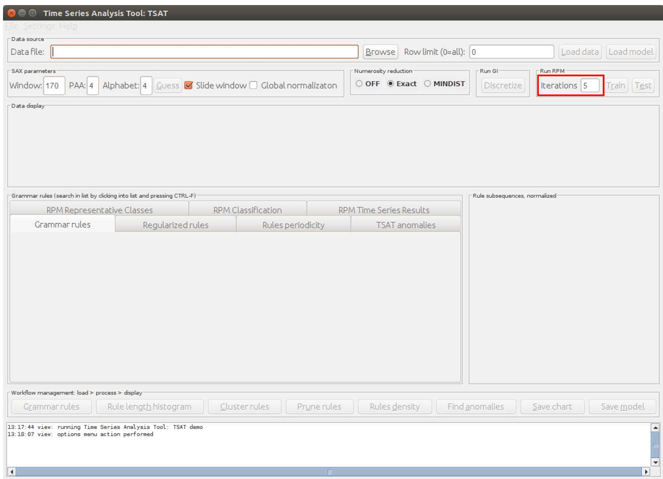
Figure 36: TSAT RPM Iteration Setting
