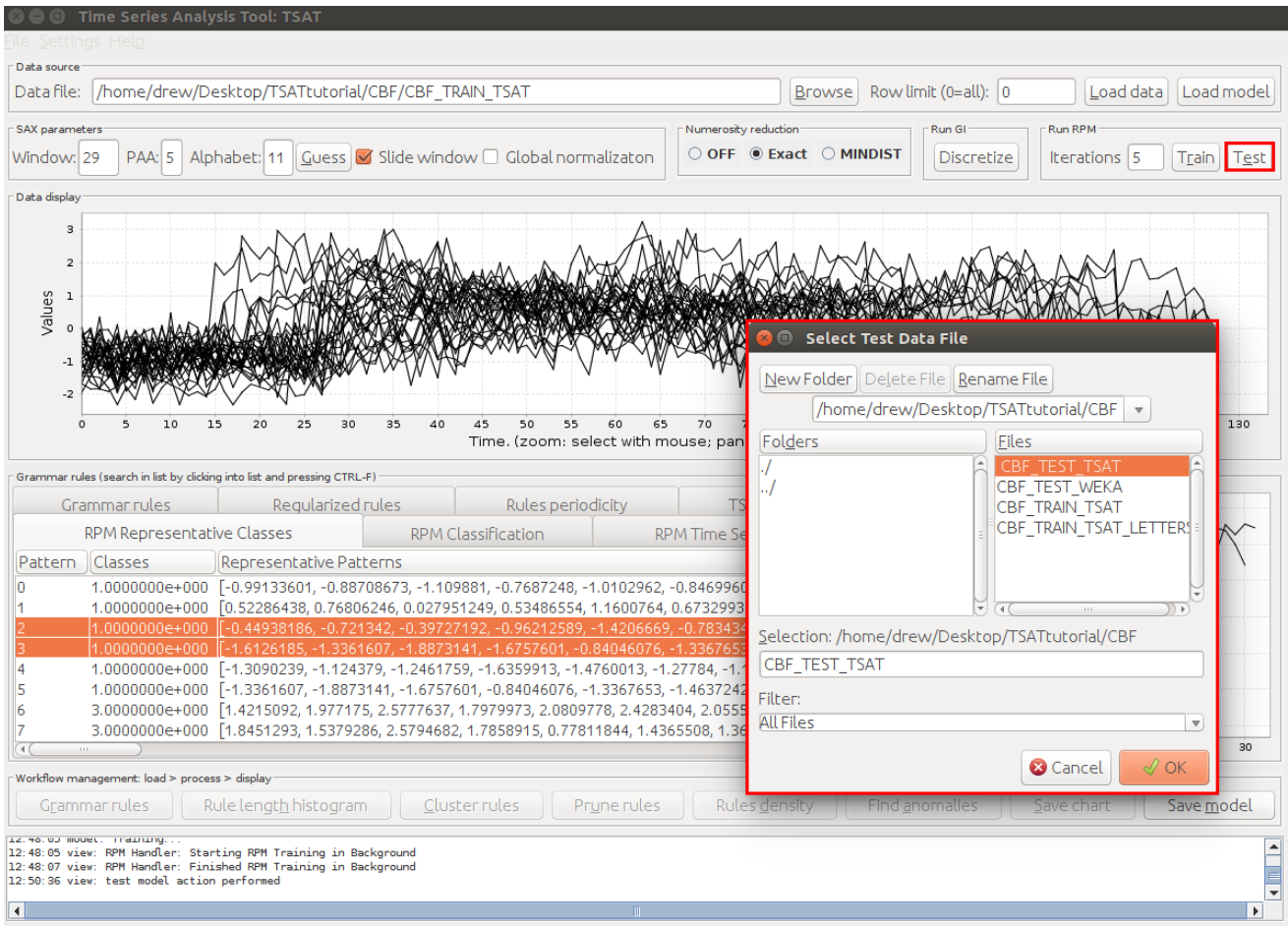
Figure 23: Testing the RPM model
