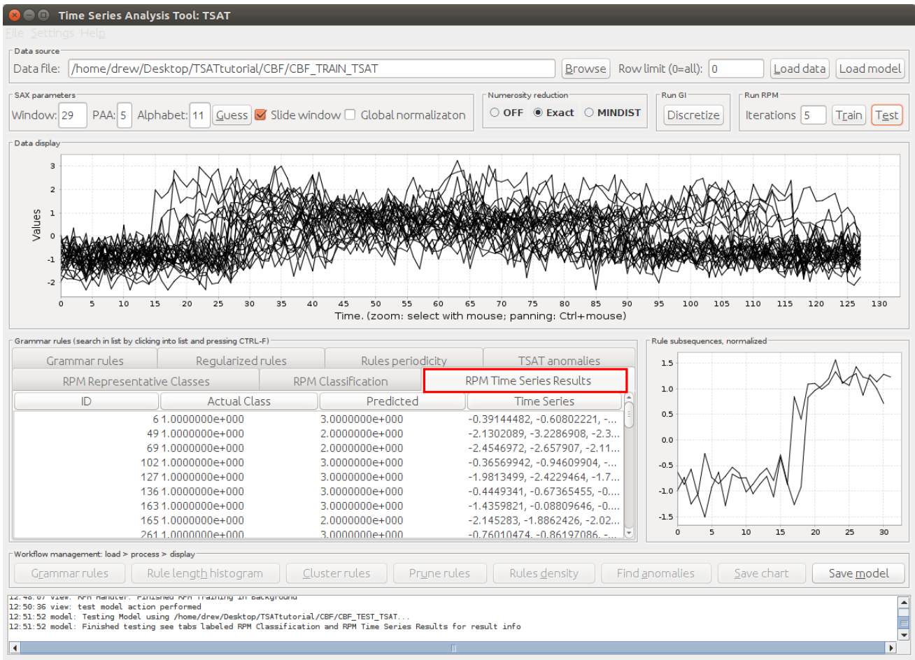
Figure 25: The results from the testing
