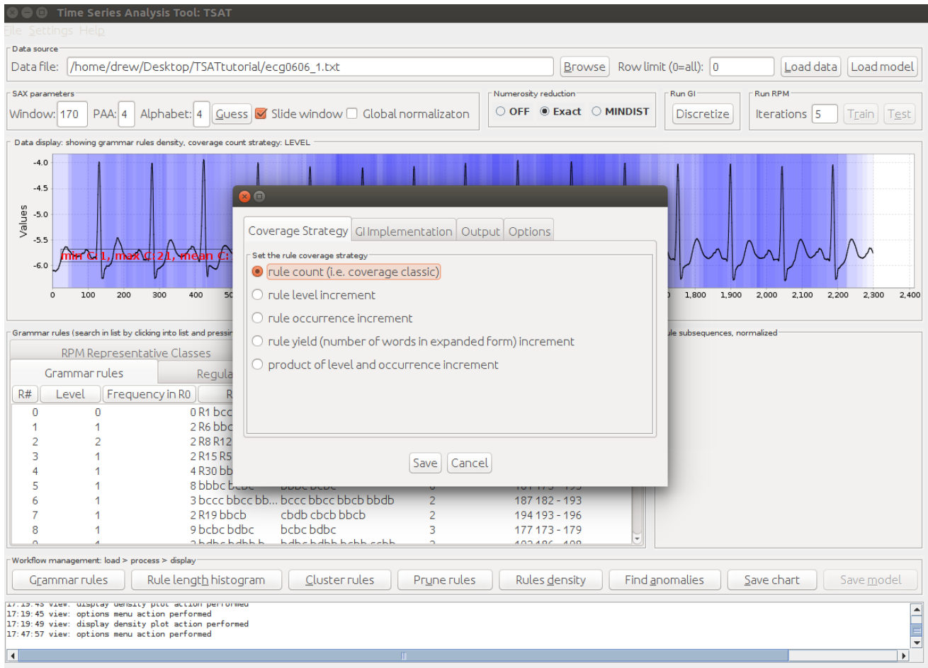
Figure 14: Changing the coverage strategy.
