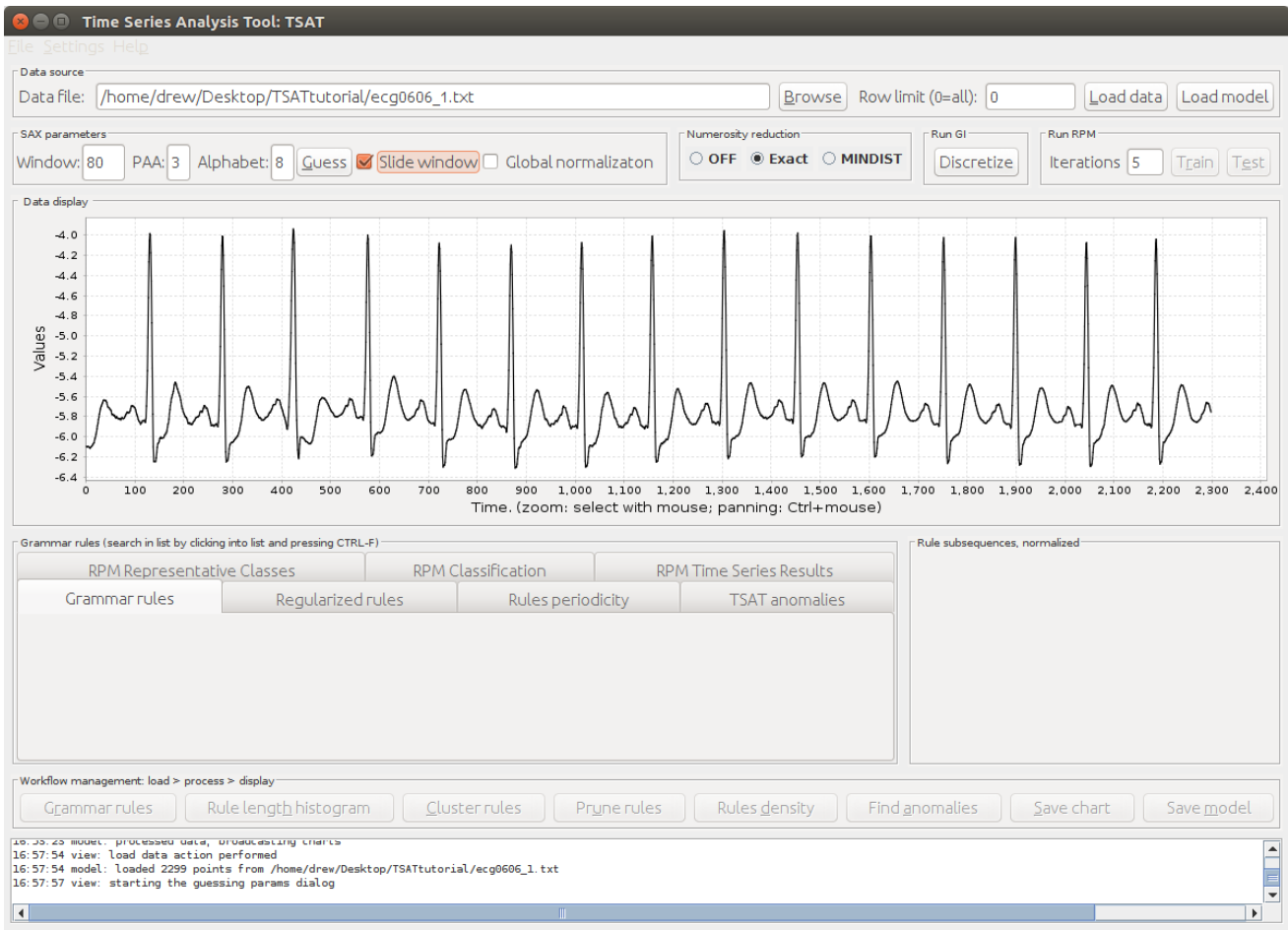
Figure 12: The inferred SAX parameters are filled in the “SAX parameters” section.
