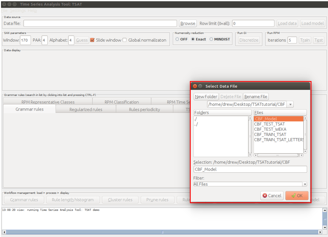
Figure 30: Open the file browser prompt
