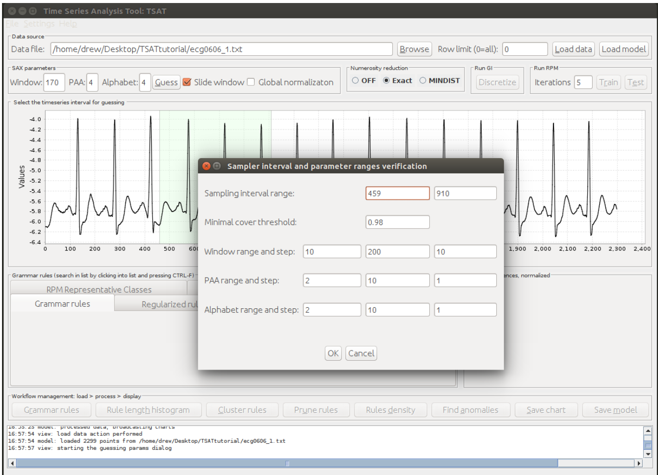
Figure 11: Adjust the range values as appropriate to your time series. Note that the larger the range the longer it will take to search.
