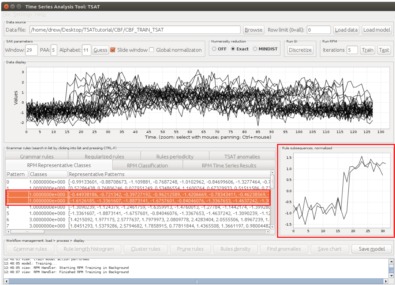
Figure 22: Representative pattern preview
