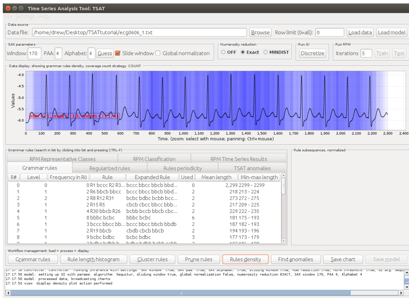
Figure 13: Rule density plot in the Data display area.
