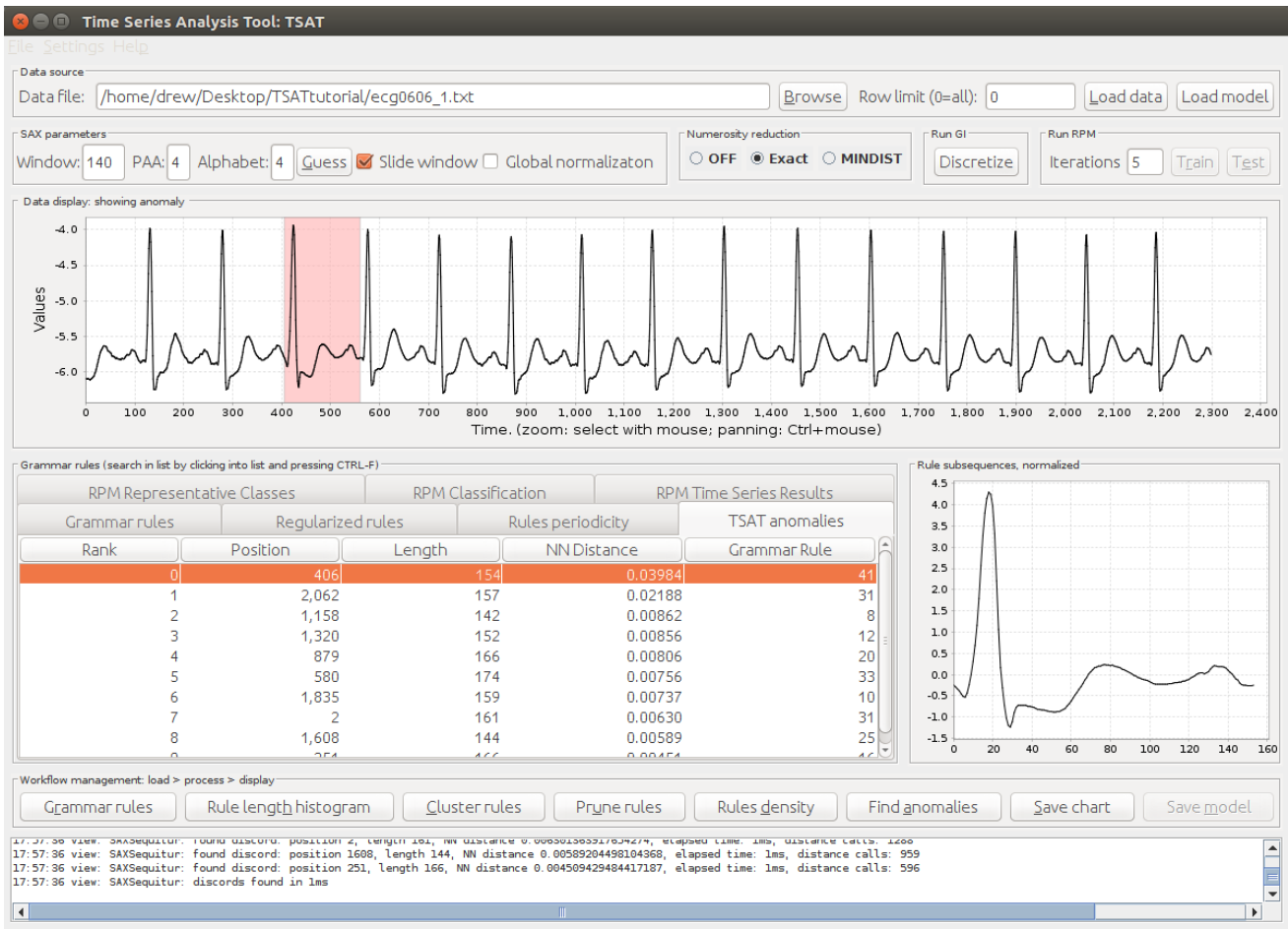
Figure 15: Rare Rule Anomalies listed in “TSAT anomalies” tab.
