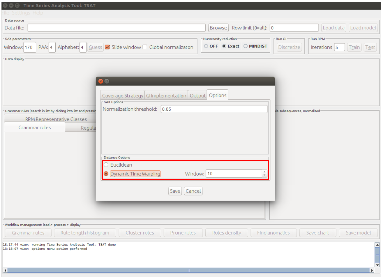
Figure 35: TSAT Settings Dialog Options DTW
