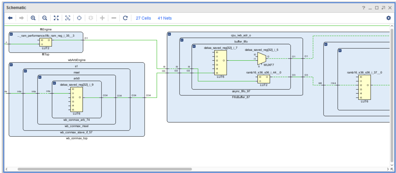
Figure 3-35: Schematic Window
