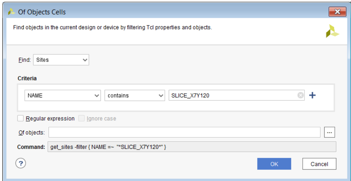
Figure 2-13: Finding an Object
