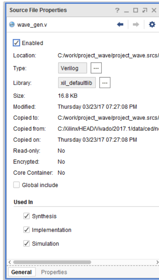
Figure 3-14: Source File Properties
