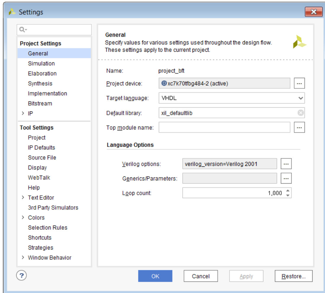
Figure 2-5: Settings Dialog Box—Project Settings General Category
