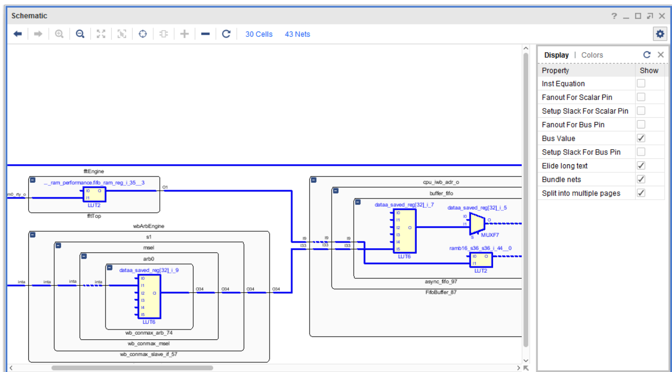
Figure 3-38: Schematic Window—Display Settings
