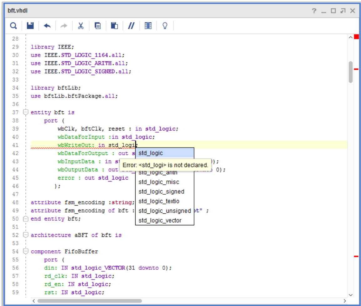
Figure 3-26: Text Editor Features
